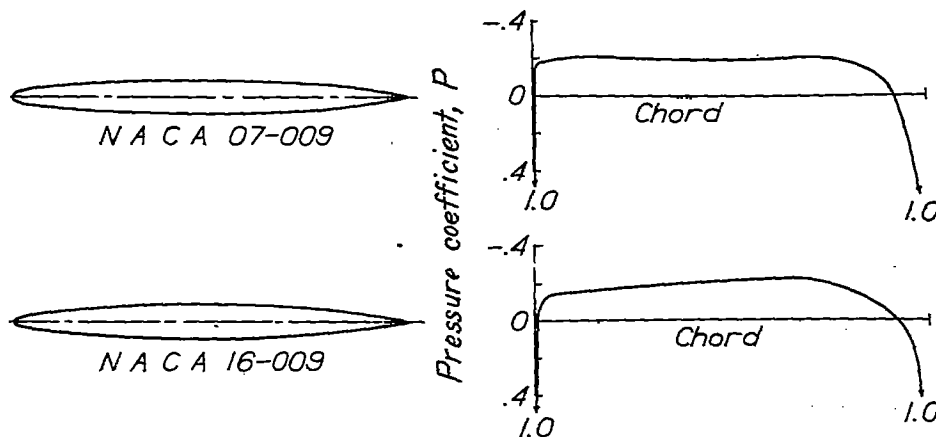
Figure 1.- Basic airfoils and theoretical pressure distributions.
