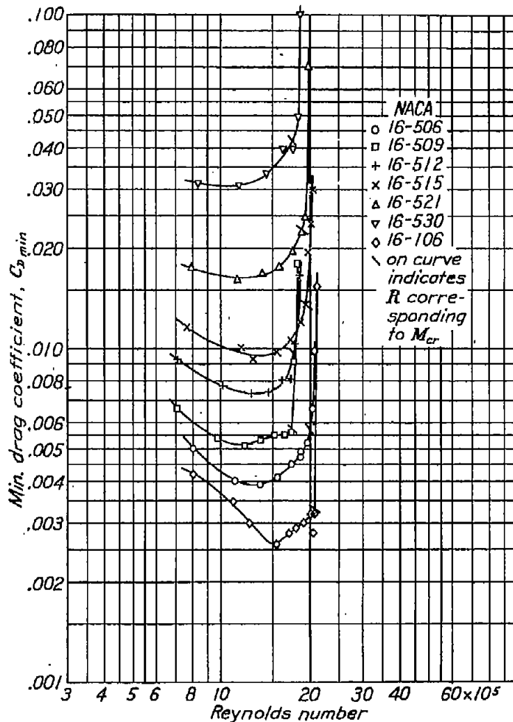
Figure 24. - Minimum drag for the NACA 16-500-series airfoils.
