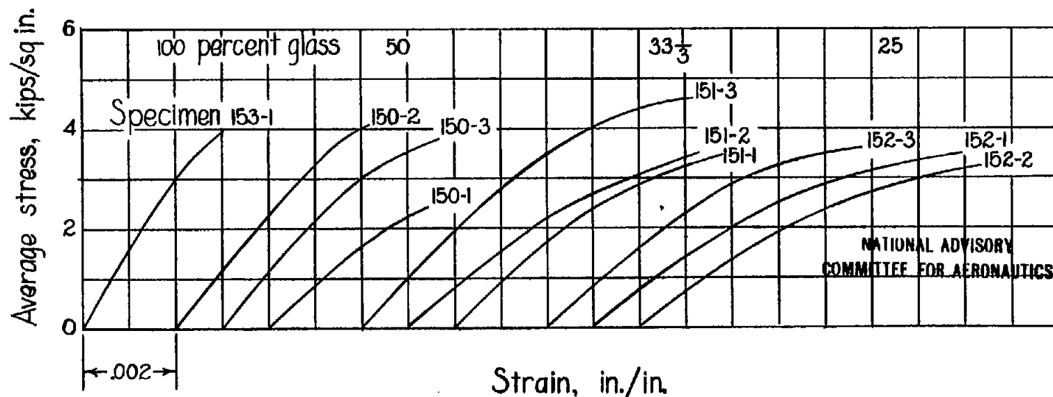
Figure 17. - Compressive panel stress-strain curves.
