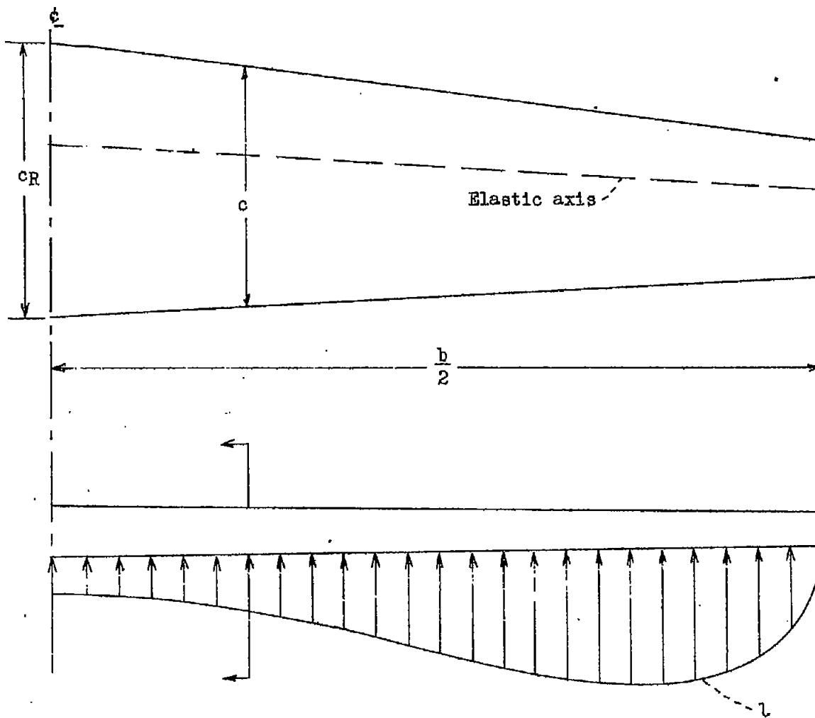
Figure 6.- Sketch of wing, showing lift distribution and elastic deformation.
