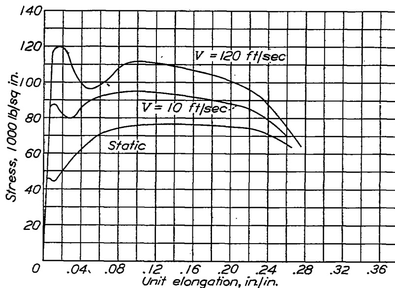
Figure 26.- Stress strain curves, SAE 1035 steel, fully annealed.
