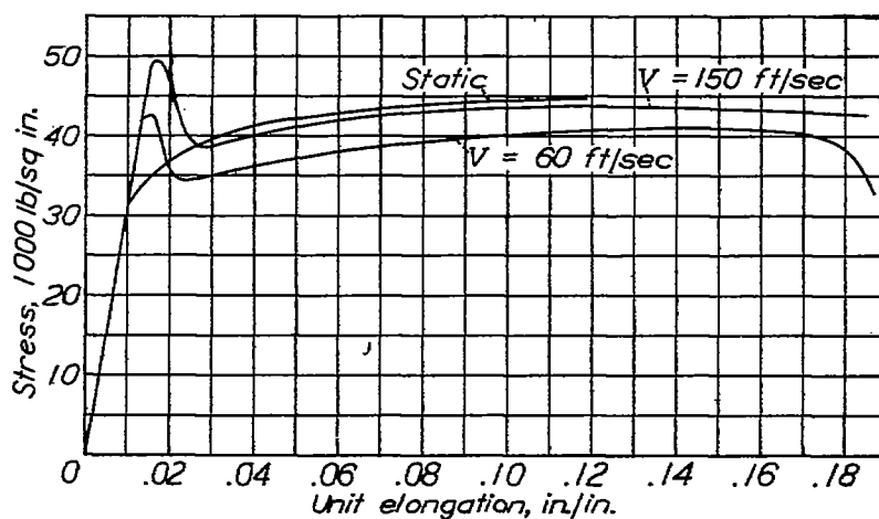
Figure 20.- Stress strain curves, Dow metal X.
