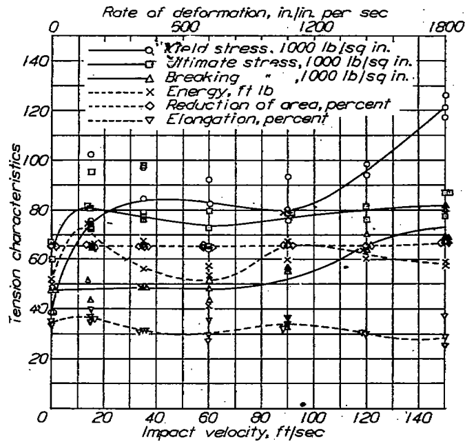
Figure 46.- Tension characteristics against impact velocity. Hot rolled steel.
