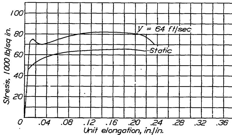
Figure 17.- Stress strain curves, 24ST aluminum alloy.
