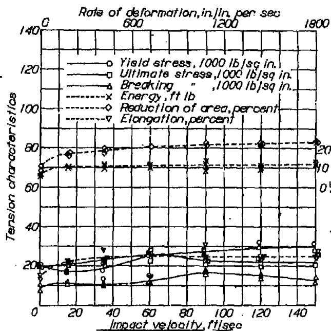
Figure 36.- Tension character- istics against impact velocity. Aluminum.
