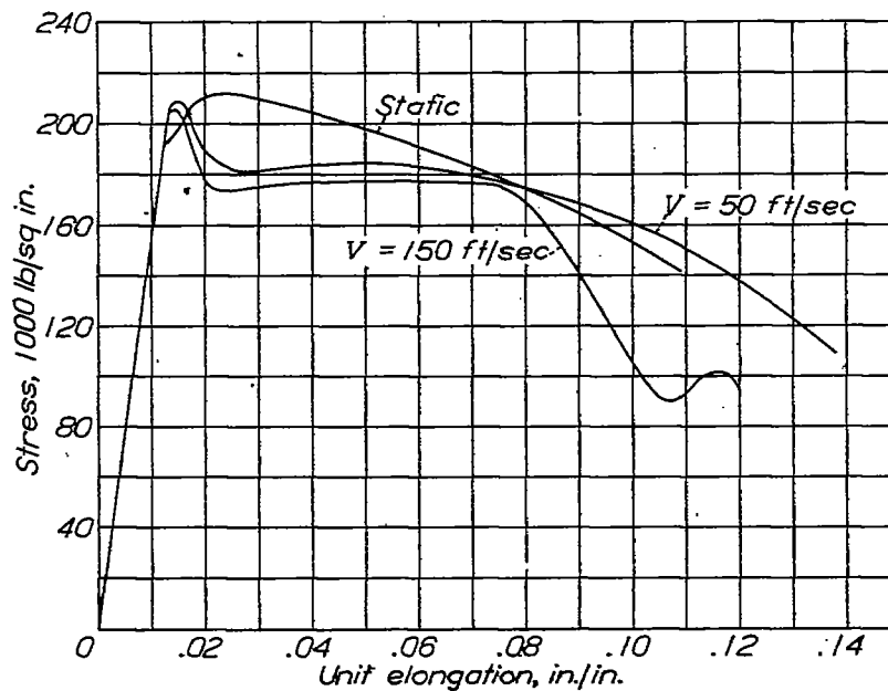
Figure 27.- Stress strain curves, SAE X4130, drawn 600°F.
