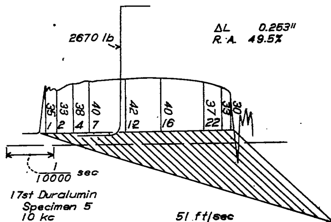
Figure 12.- Typical analysis of enlarged force-time diagram.
