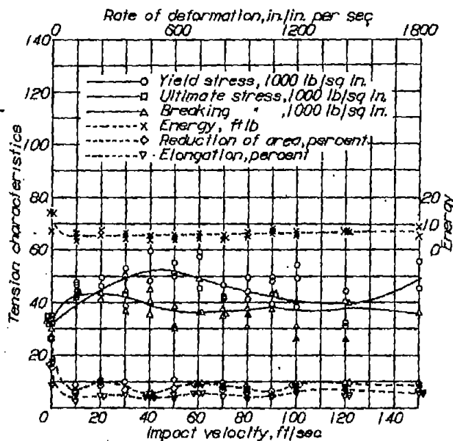
Figure 40.- Tension character- istics against impact velocity. Dow metal M.
