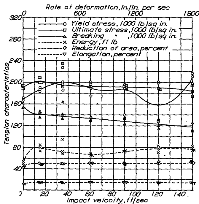
Figure 52.- Tension characteristics against impact velocity. SAE 6140 drawn 1020°F.
