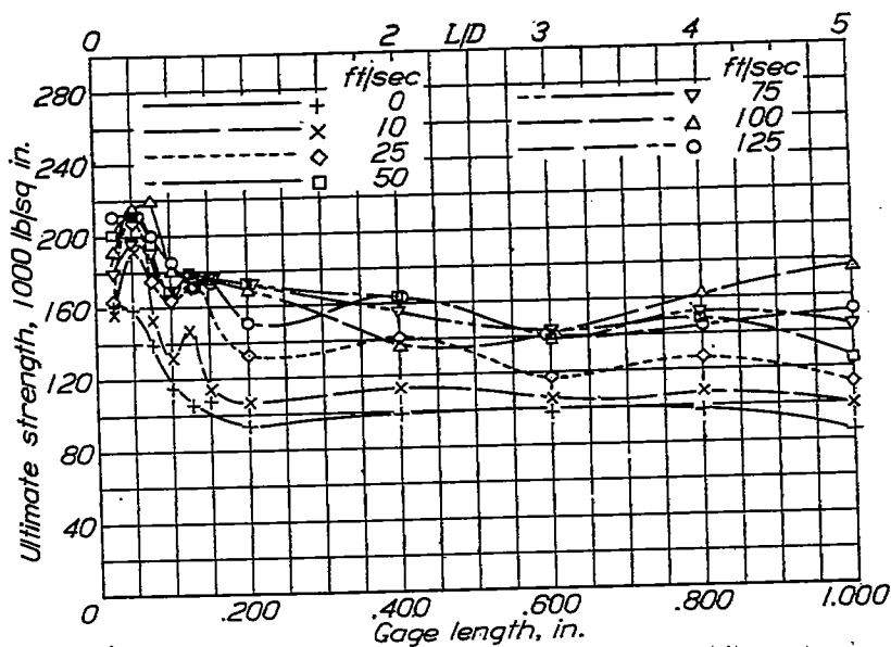
Figure 60.- Ultimate strength against gage length.
