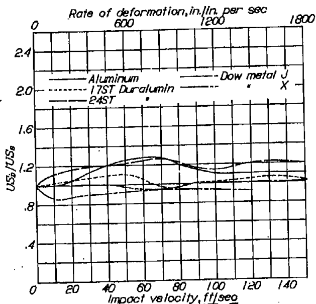
Figure 58a.- Ratio of dynamic to static ultimate stress against impact velocity. Aircraft materials.
