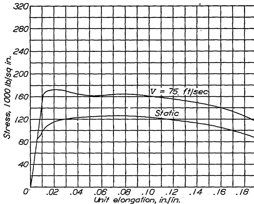
Figure 34.- Stress strain curves, 16-2 stainless steel, drawn 12000.
