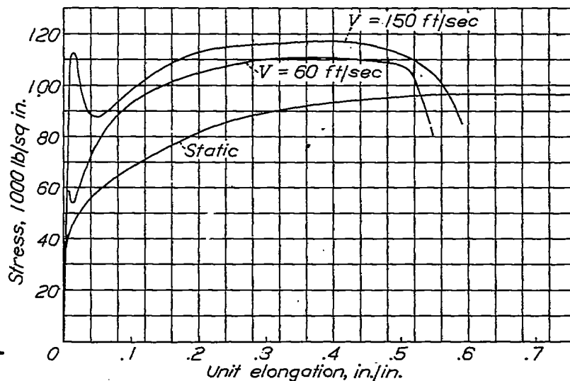
Figure 35.- Stress strain curves, 18-8 stainless steel.
