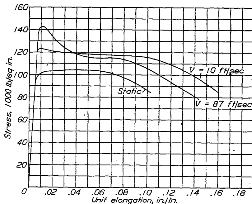
Figure 24.- Stress strain curves, SAE 1112 steel, cold drawn.
