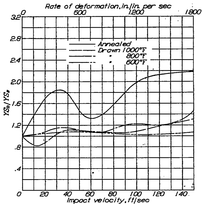
Figure 57c.- Ratio of dynamic to static yield stress against impact velocity. SAE X4130.
