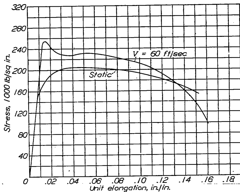
Figure 32.- Stress strain curves, 16-2 stainless steel, drawn 7000°.
