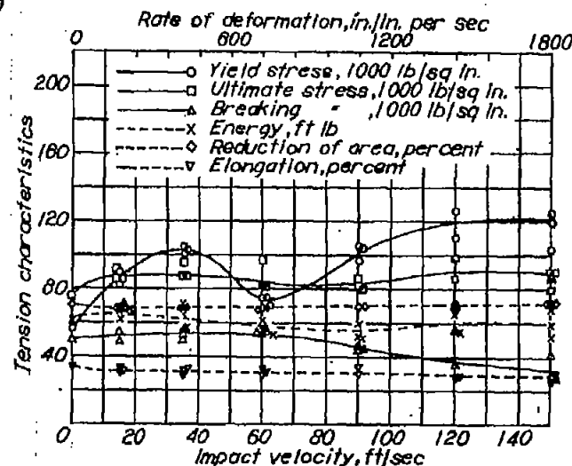
Figure 51.- Tension character- istics against impact velocity. SAE X4130 annealed.
