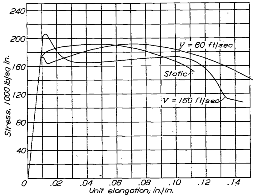
Figure 31.- Stress strain curves, SAE 6140, drawn 1020°F.
