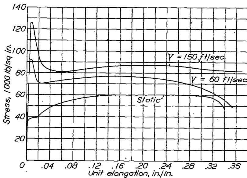
Figure 25.- Stress strain curves, hot rolled steel.
