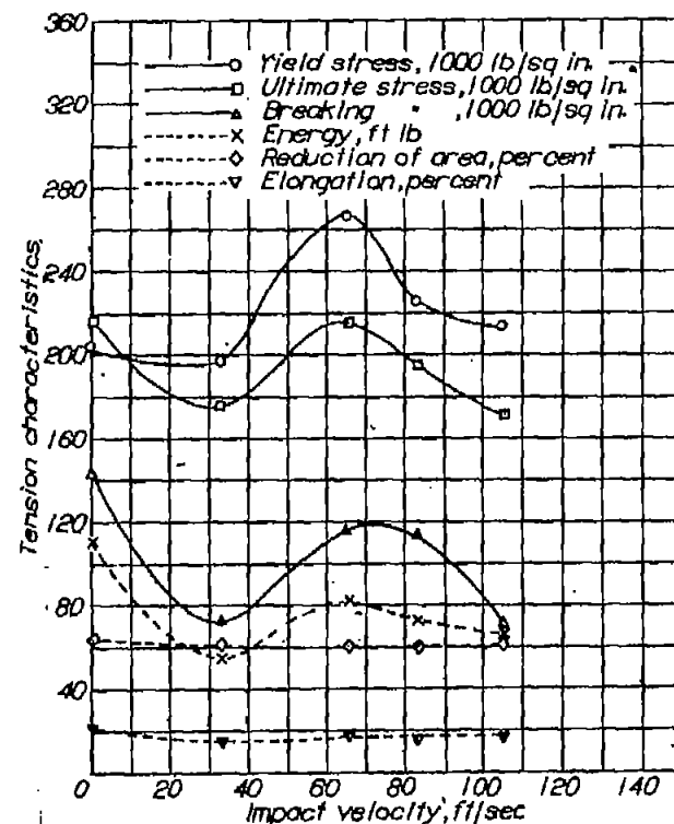
Figure 55.- Tension characteristics against impact velocity. 16-2 stainless steel, oil quenched, drawn 900°.
