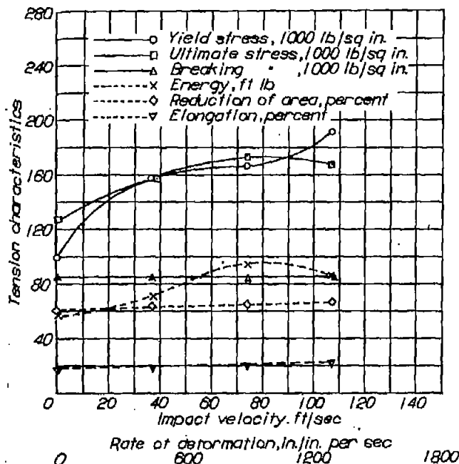
Figure 54.- Tension characteristics against impact velocity. 16-2 stainless steel, oil quenched, drawn 1200°
