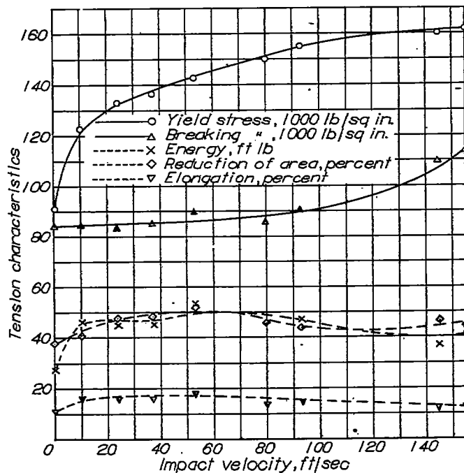
Figure 45.- Tension characteristics against impact velocity. SAE 1112 steel, cold drawn.
