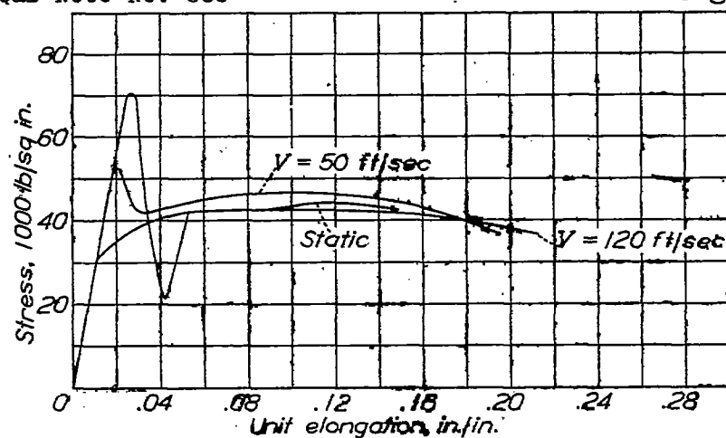
Figure 18.- Stress strain curves, Dow metal J.
