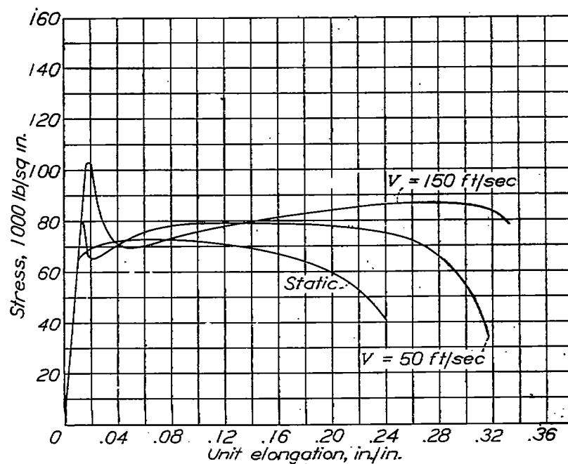
Figure 23.- Stress strain curves, silicon bronze.
