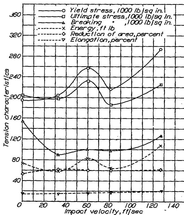
Figure 53.- Tension characteristics against impact velocity. 16-2 stainless steel, oil quenched, drawn 700°F.
