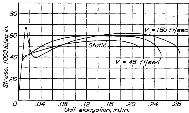
Figure 16.- Stress strain curves, 17ST duralumin.
