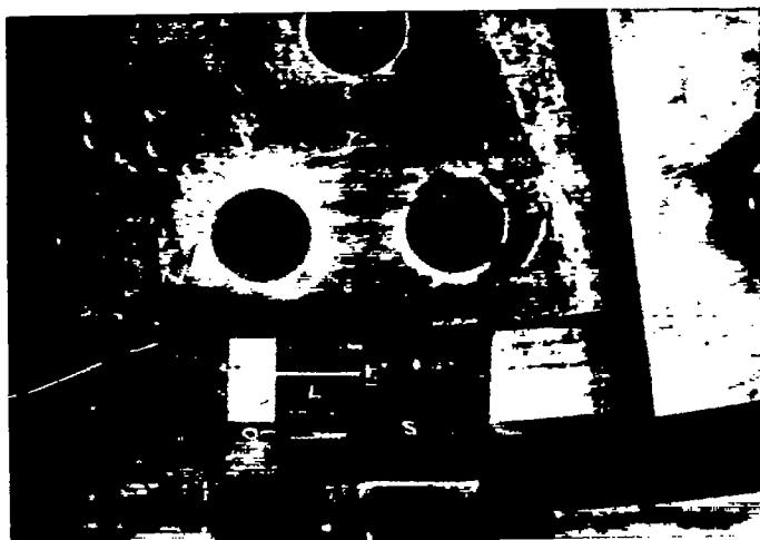
Figure 6.- Specimen, tup, and extensometer before impact.
