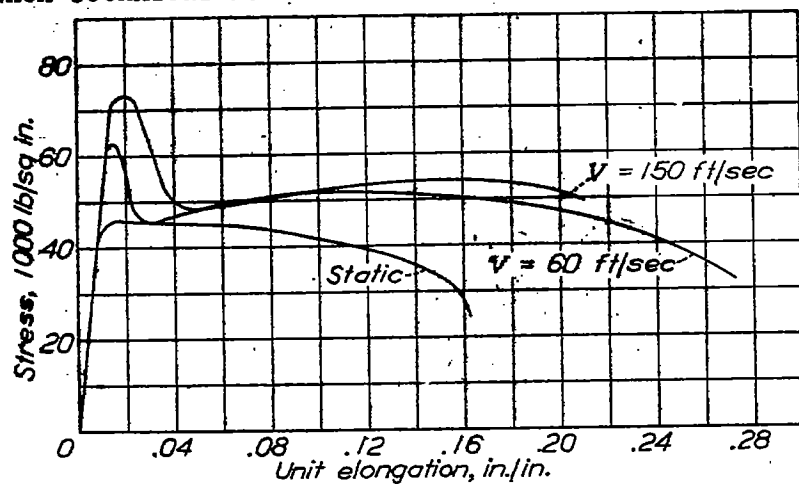
Figure 21.- Stress strain curves, copper.
