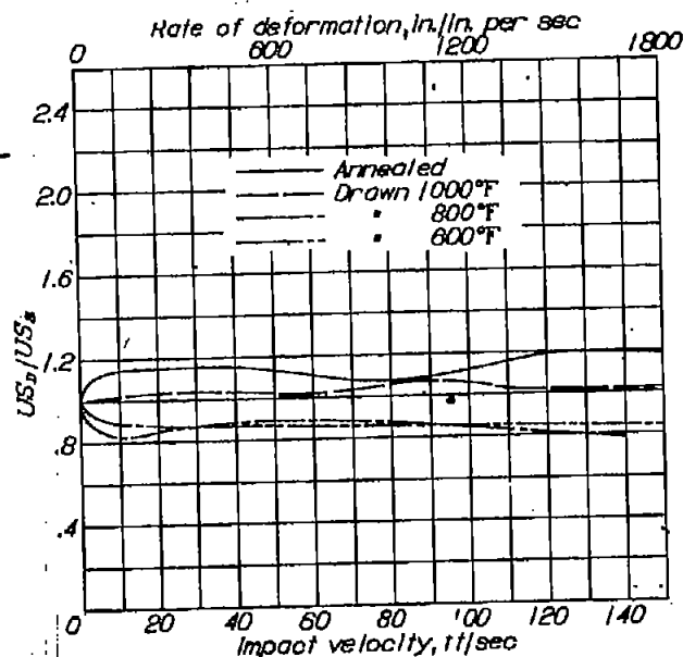
Figure 58c.- Ratio of dynamic to static ultimate stress against impact velocity. SAE X4130.
