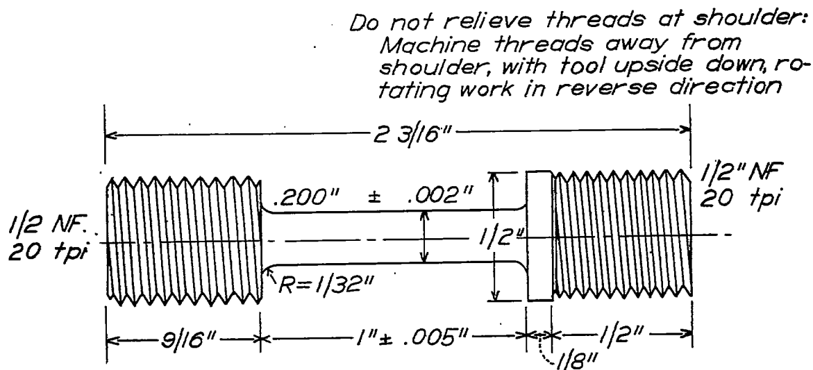
Figure 13.- Tension Specimens. Scale: twice full size.
