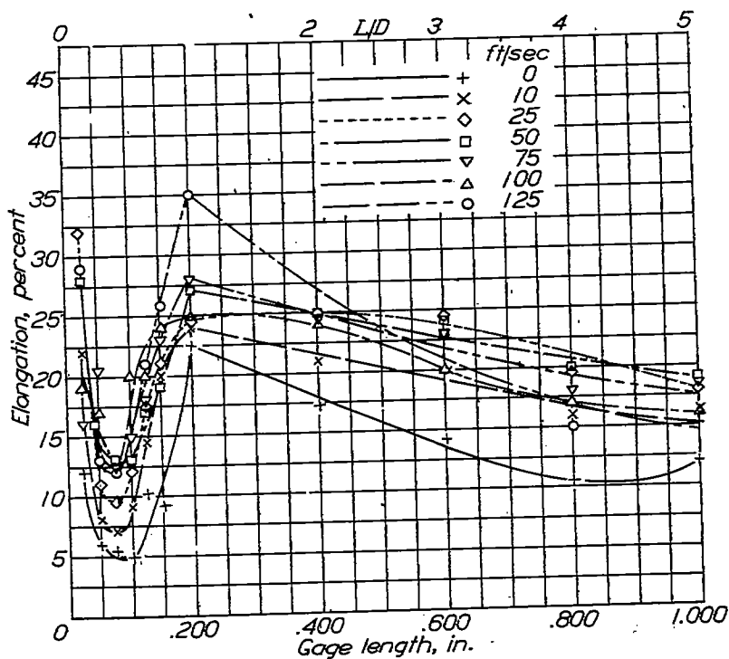
Figure 61.- Elongation against gage length.
