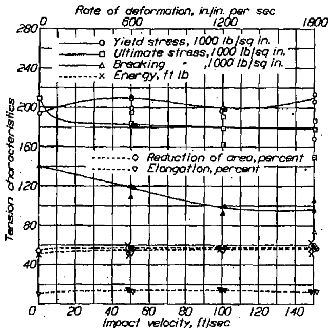
Figure 48.- Tension character- istics against impact velocity. SAE X4130 drawn 600°F
