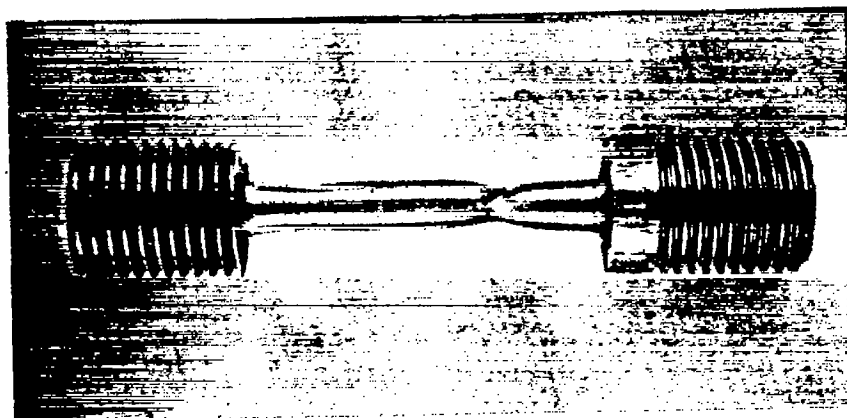
Figure 14.- Double necked specimen.
