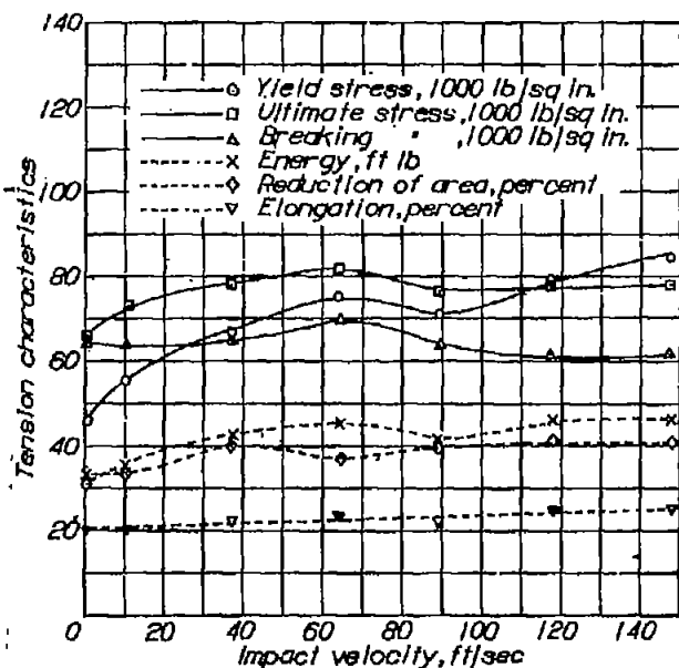
Figure 38.- Tension character- istics against impact velocity. 24ST aluminum alloy.
