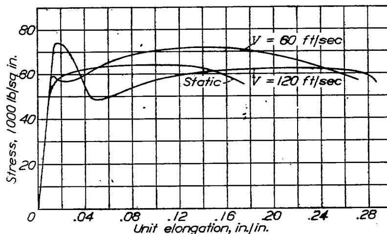
Figure 22.- Stress strain curves, brass.
