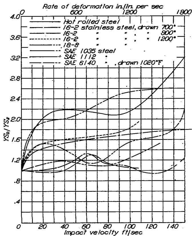
Figure 57d.- Ratio of dynamic to static yield stress against impact velocity. Miscellaneous steels.
