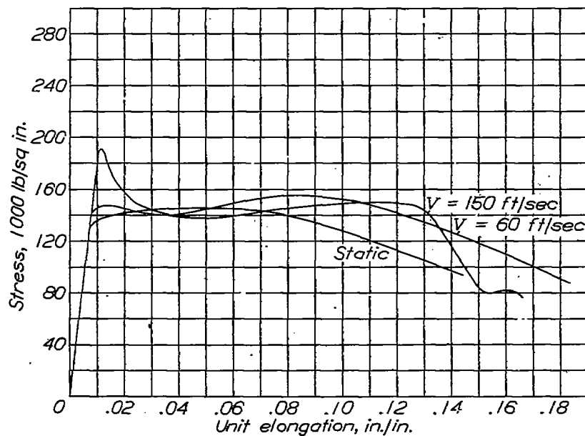
Figure 29.- Stress strain curves, SAE X4130, drawn 1000°F.
