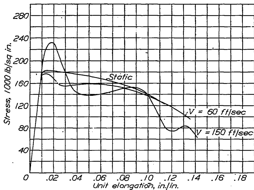
Figure 28.- Stress strain curves, SAE X4130, drawn 800°F.
