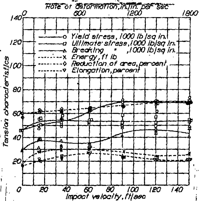
Figure 42.- Tension character- istics against impact velocity. Copper.
