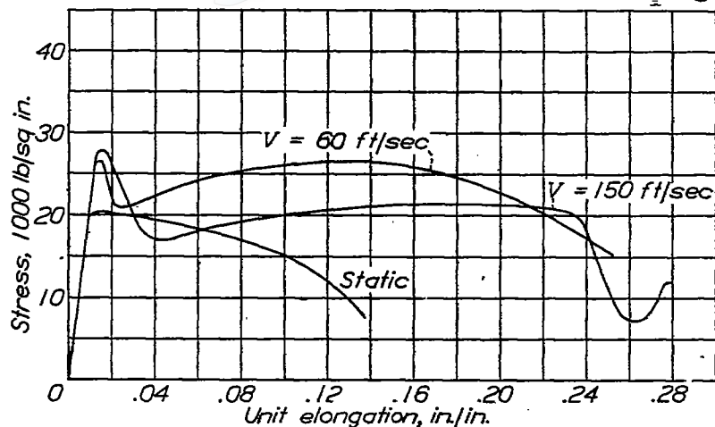
Figure 15.- Stress strain curves, aluminum.
