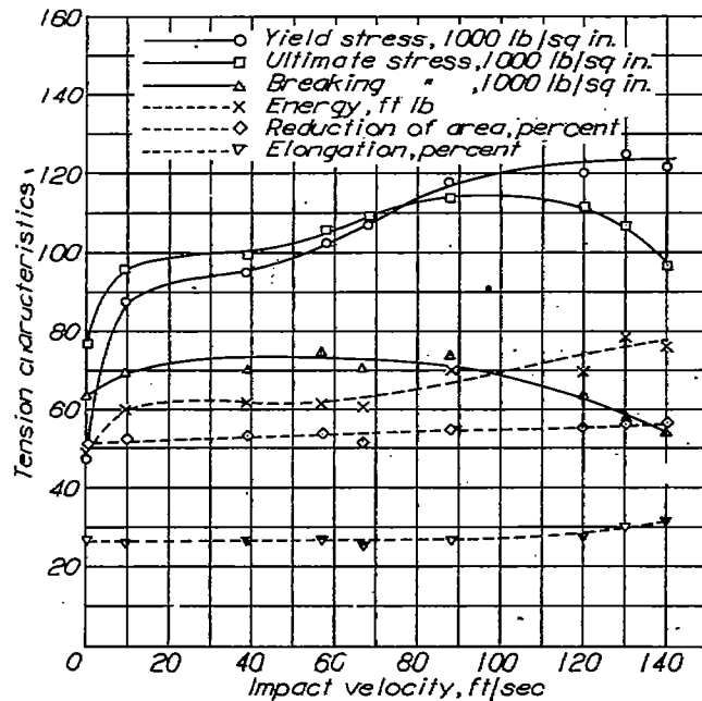
Figure 47.- Tension characteristics against impact velocity. SAE 1035 steel, fully annealed.
