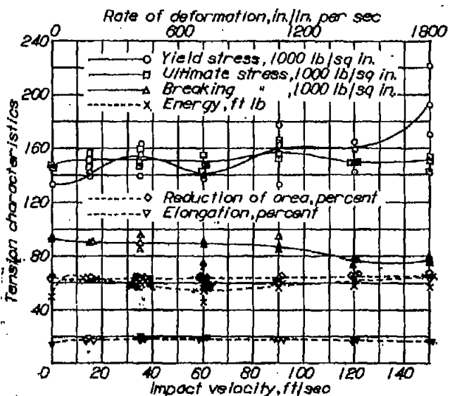
Figure 50.- Tension character- istics against impact velocity. SAE X4130 drawn 1000°F.
