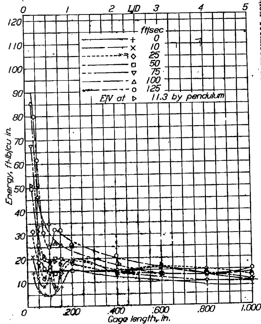
Figure 63.- Energy per unit volume against gage length.
