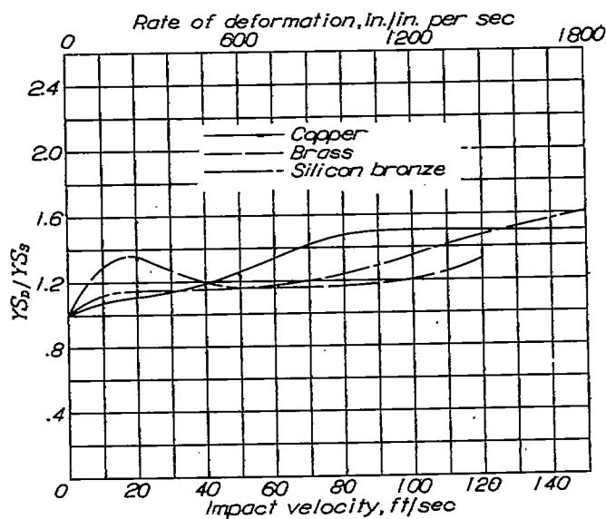
Figure 57b.- Ratio of dynamic to static yield stress against impact velocity. Copper and its alloys.
