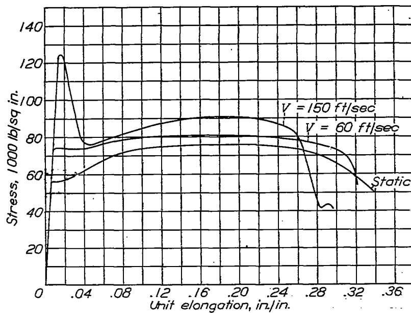
Figure 30.- Stress strain curves, SAE X4130 annealed.
