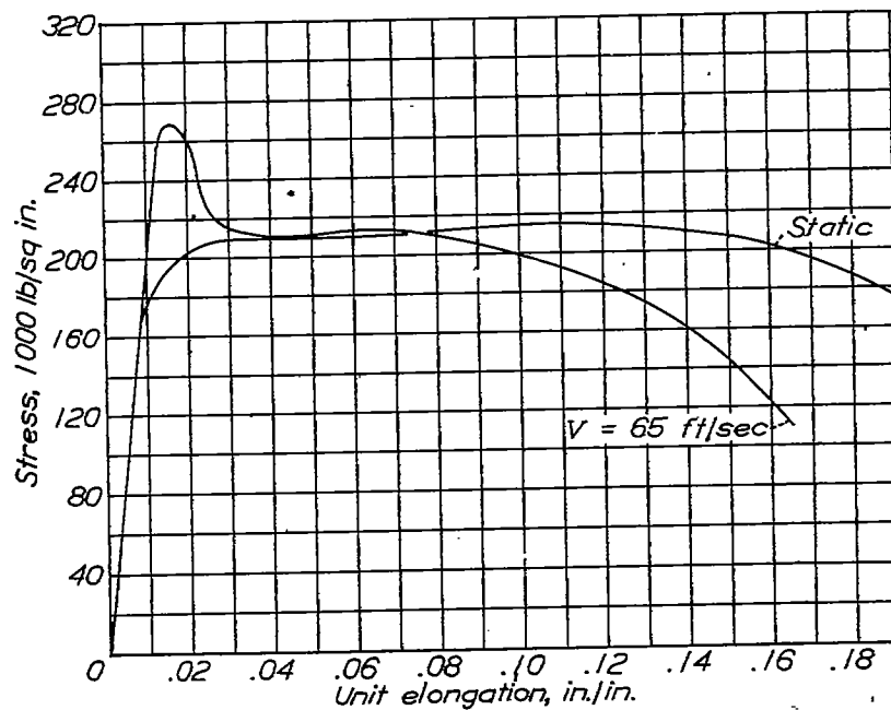
Figure 33.- Stress strain curves, 16-2 stainless steel, drawn 9000°.
