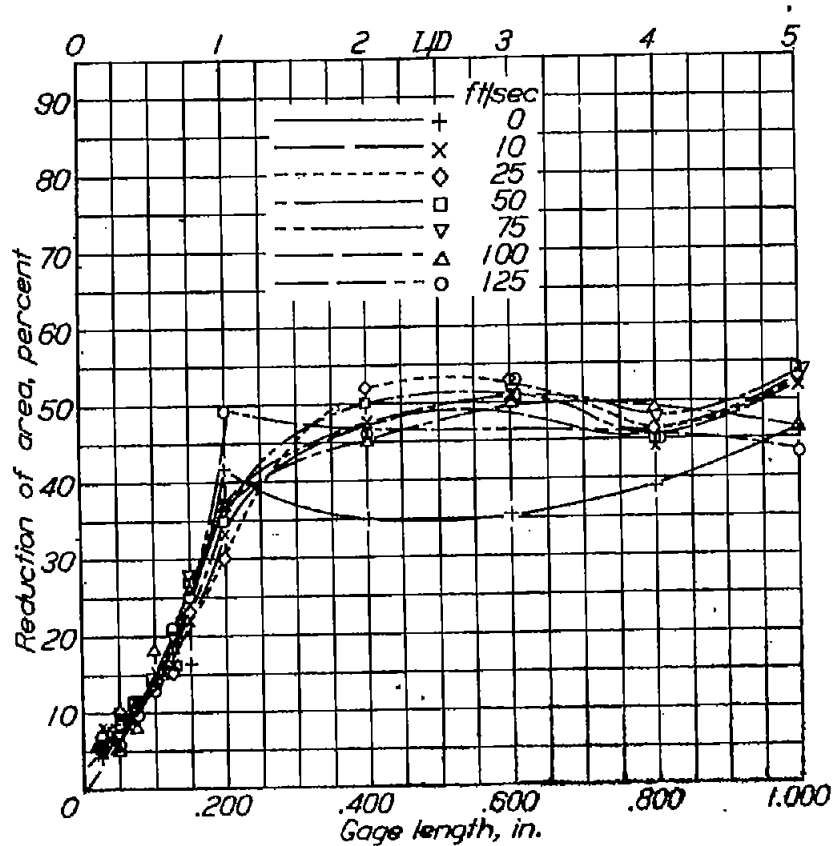
Figure 62.- Reduction of area against gage length.
