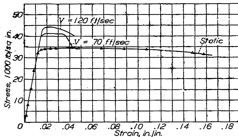
Figure 19.- Stress strain curves, Dow metal M.
