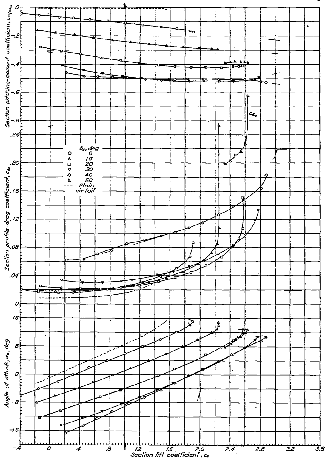
Figure 8.- Aerodynamic section characteristics of an NACA 23012 airfoil with a 0.30c slotted flap 1-b. Slot gap = 0.03c.
