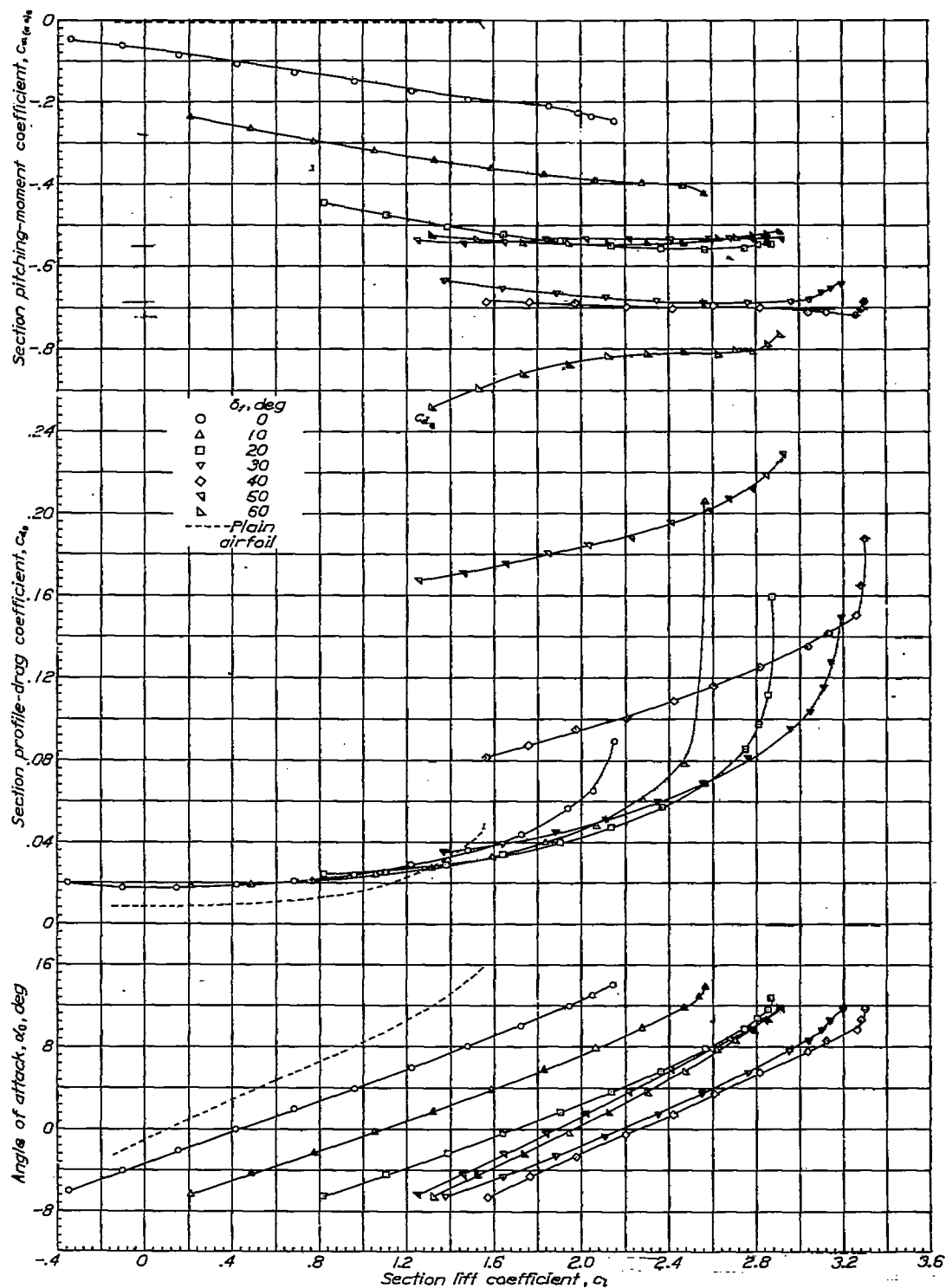
Figure 3.- Aerodynamic section characteristics of an NACA 23012 airfoil with a 0.30c Fowler flap. Slot gap = 0.015c.
