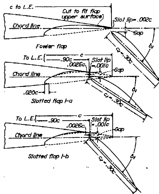
Figure 1.- Sections of NACA 23012 airfoil with arrangements of 0.30c slotted flaps.
