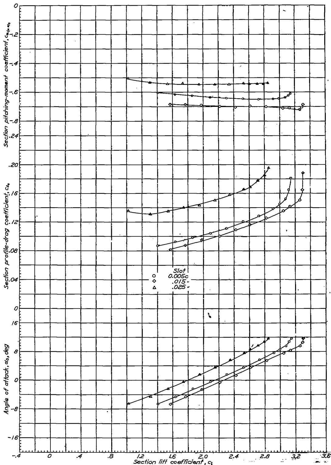
Figure 4.- Comparison of aerodynamic section characteristics of an NACA 23018 airfoil with a 0.30c Fowler flap at three slot gaps. \delta f = 40^\circ .
