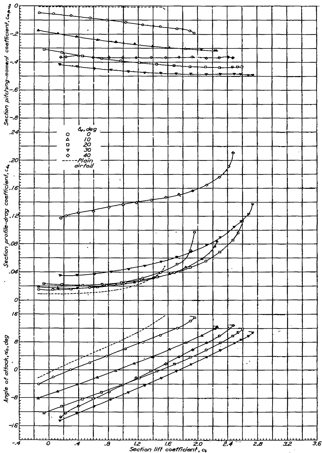
Figure 7.- Aerodynamic section characteristics of an NACA 23012 airfoil with a 0.30c slotted flap 1-a. Slot gap = 0.03c.
