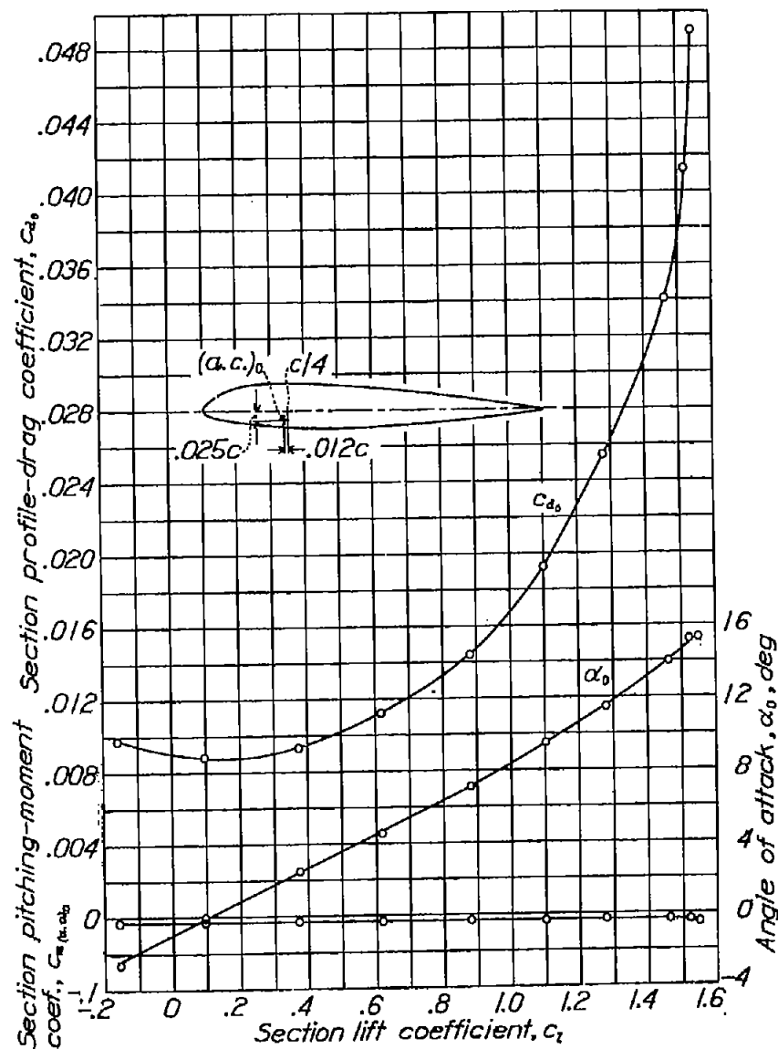
Figure 2.- Aerodynamic section characteristics of NACA 23012 plain airfoil.
