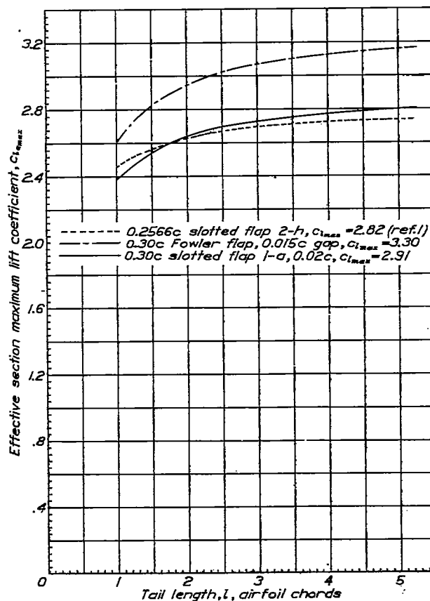
Figure 13.- Comparison of three slotted flaps on an NACA 23012 airfoil.
