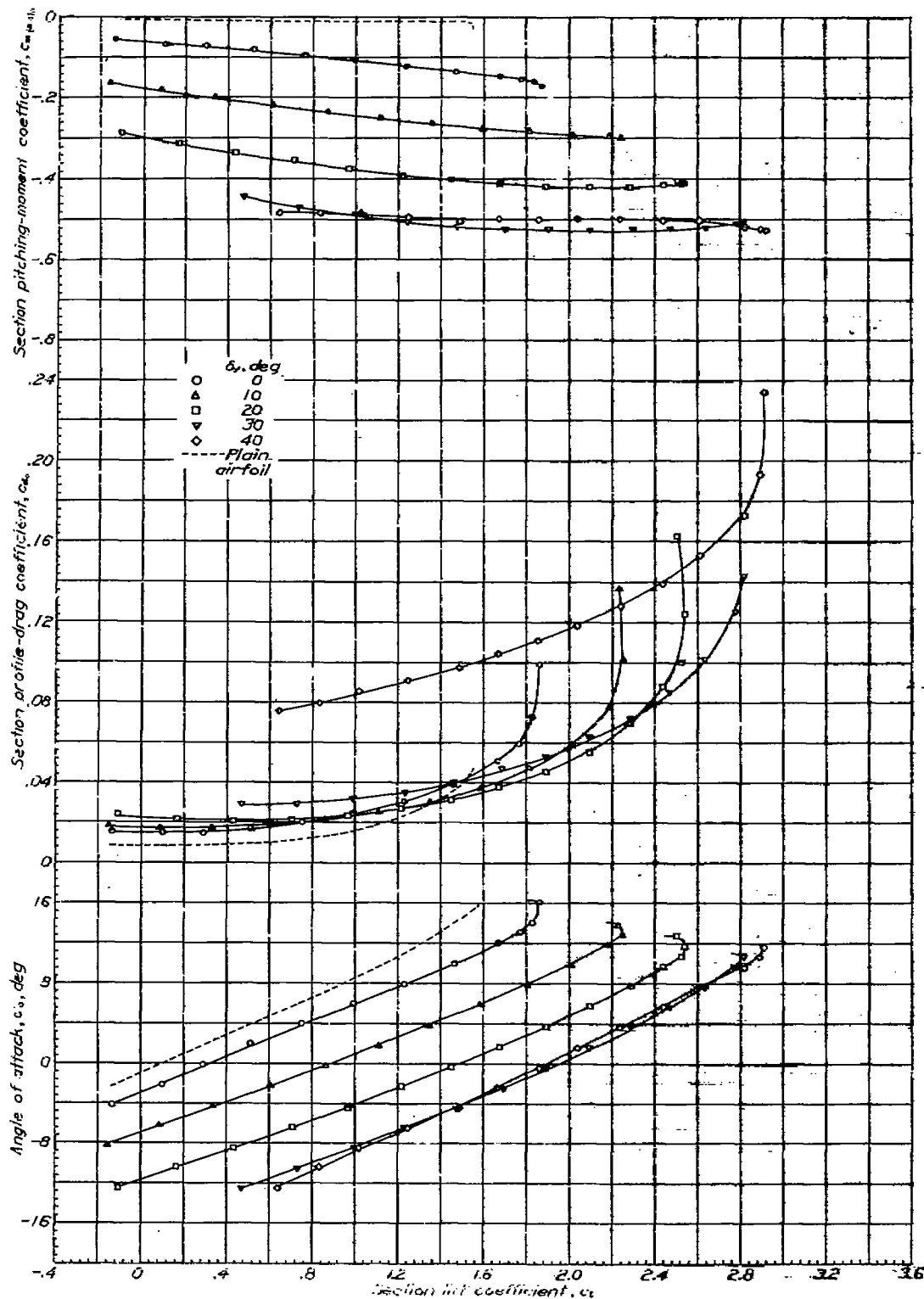
Figure 6.- Aerodynamic section characteristics of an NACA 23012 airfoil with a 0.30c slotted flap 1-a. Slot gap = 0.02c.
