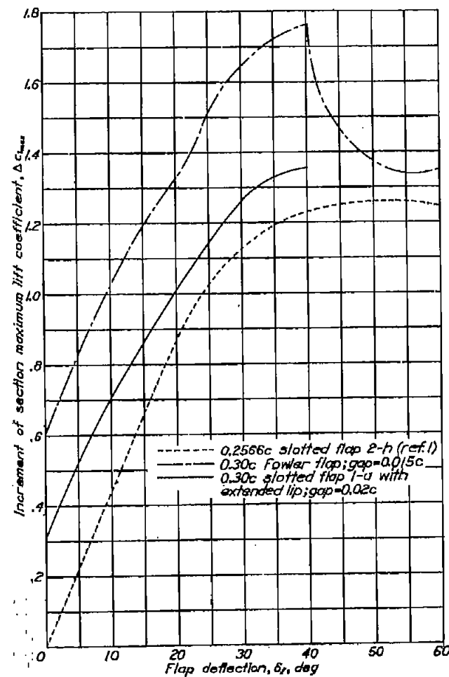
Figure 11.- Comparison of increments of section maximum lift coefficient for three flaps on an NACA 23012 airfoil.
