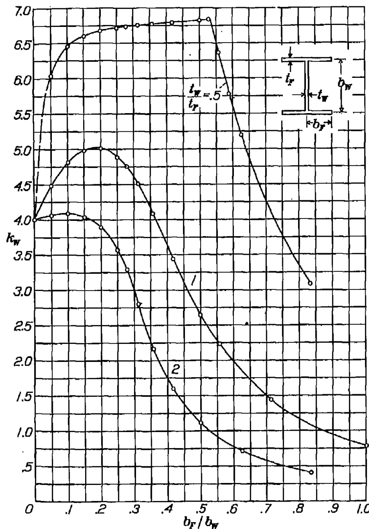
Figure 4.- Minimum values of k_y for centrally loaded columns of I-section ( \mu=0.5 )
