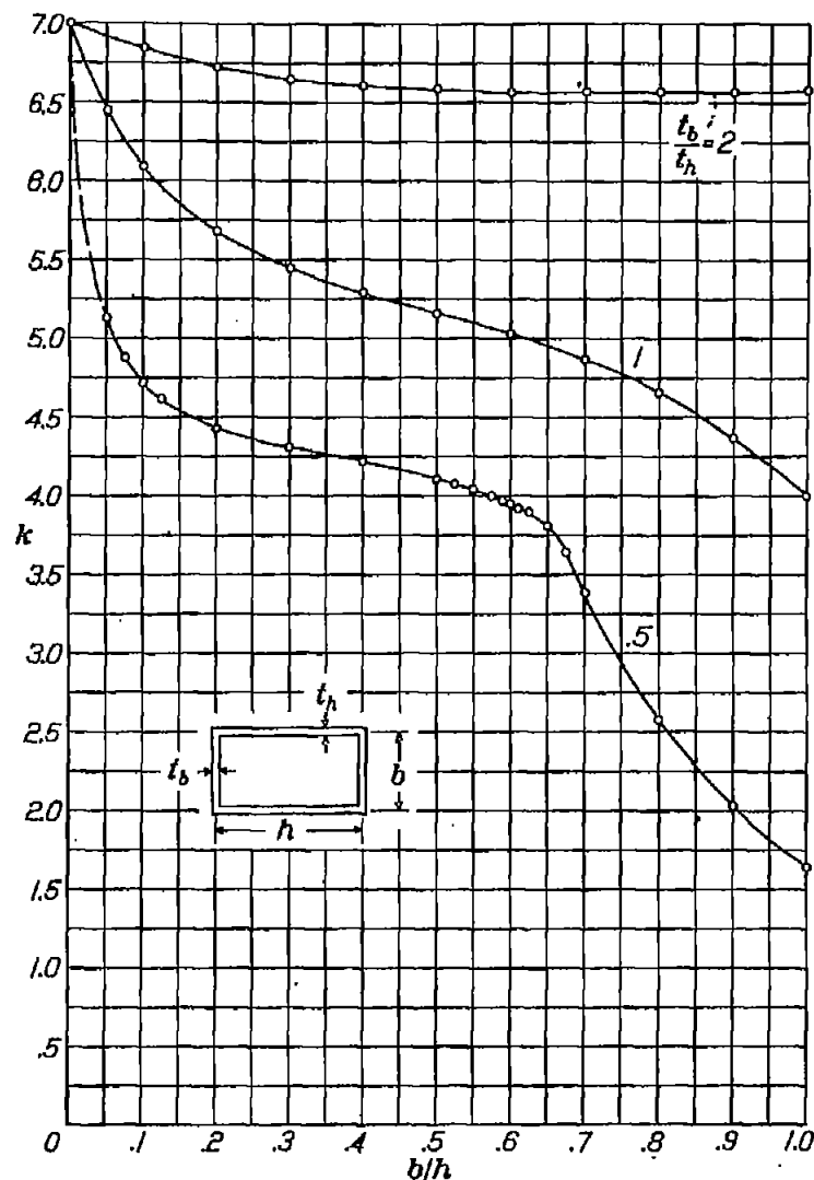
Figure 7.- Minimum values of k for a centrally loaded symmetrical rectangular tube ( \mu = 0.3 ). \frac{f_{cr}}{\eta} = \frac{k \pi^2 E t_h^2}{12(1 - \mu^2) h^2}
