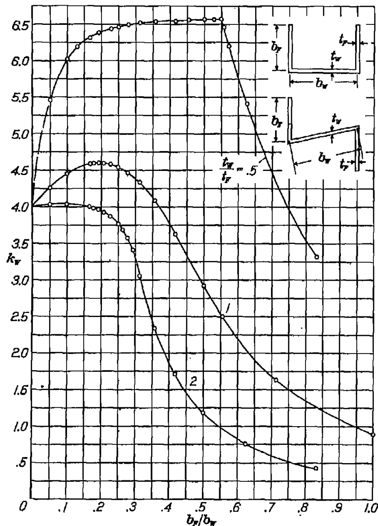
Figure 6.- Minimum values of k_w for centrally loaded columns of channel section and Z-section ( \mu = 0.3 ). \frac{f_{cr}}{\eta} = \frac{k_w \pi^2 E t_w^2}{12(1 - \mu^2) b_w^2}
