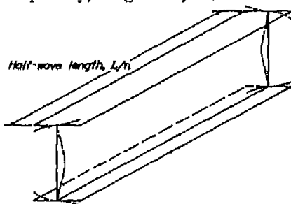
Figure 2.- Displacements of the cross section in secondary, or local, failure of a column.
