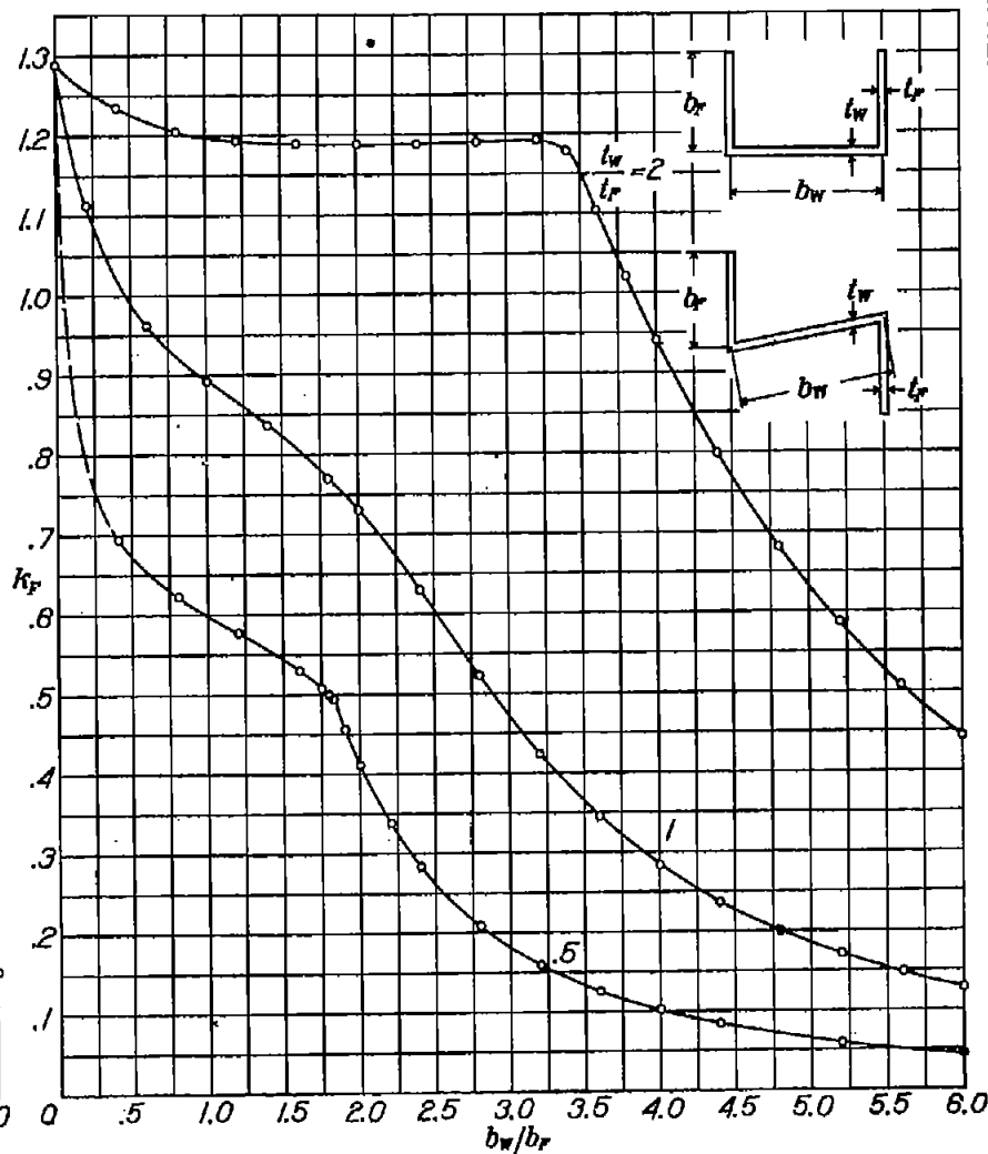
Figure 5.- Minimum values of k_p for centrally loaded columns of channel section and Z-section ( \mu=0.3 )
