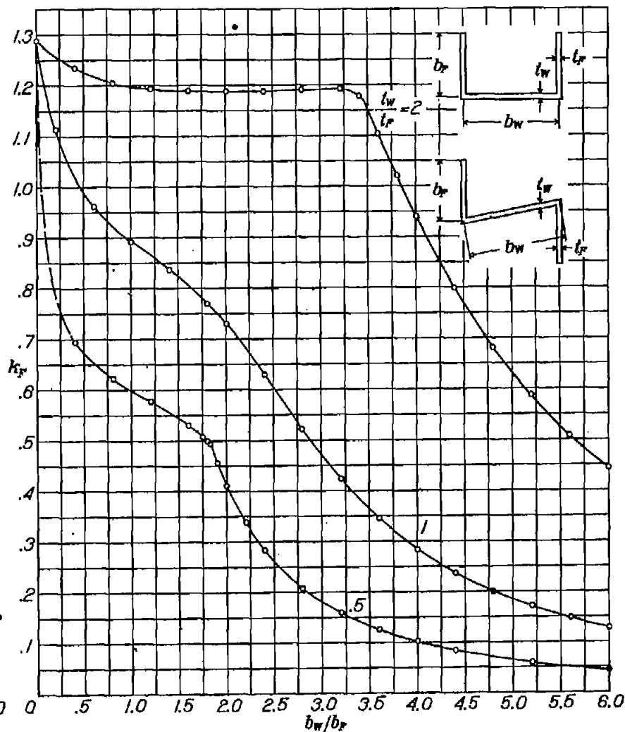
Figure 5.- Minimum values of k_r for centrally loaded columns of channel section and Z-section ( \mu=0.3 )
