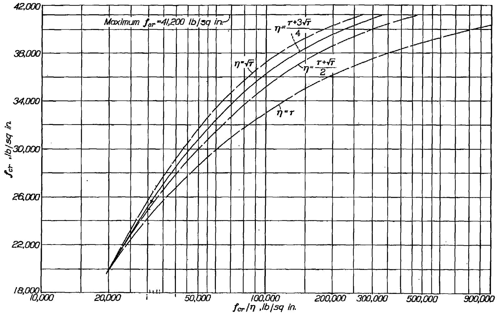
Figure 8.- Variation of f_{cr} with f_{cr}/\eta for 24ST aluminum alloy. When f_{cr} < 19,600 lb/sq in., \eta=1 and f_{or} = f_{cr}/\eta .
