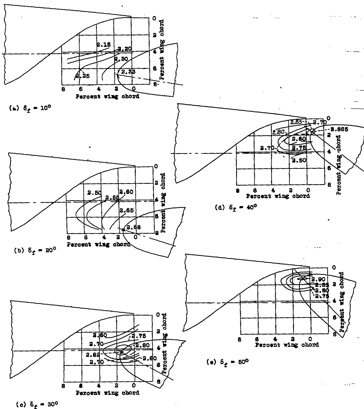
Figure 5.- Contours of flap location for c_{l_{max}} . The 0.40 c_{l_{max}} slotted flap l-b.
