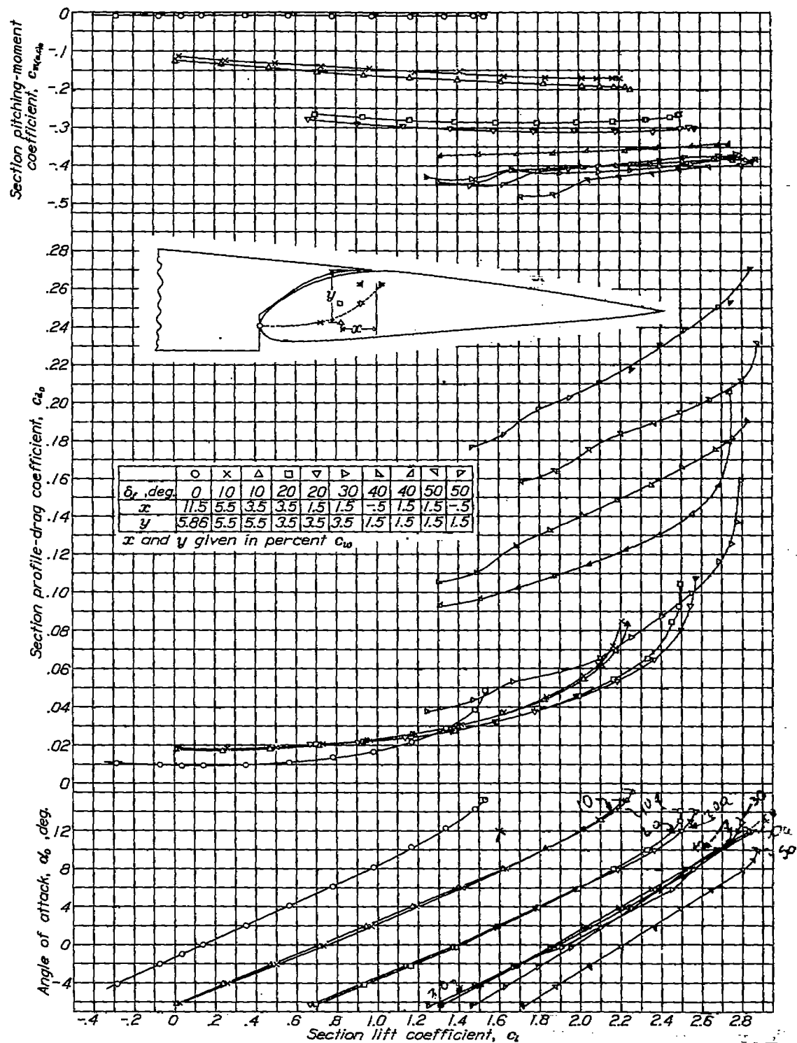
Figure 8.- Section aerodynamic characteristics of N.A.C.A. 23012 airfoil with 0.40 c_w slotted flap 1-a.
