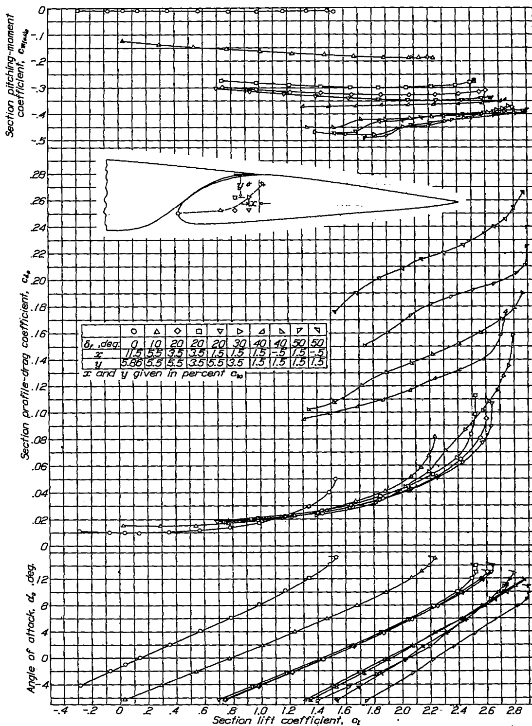
Figure 9.- Section aerodynamic characteristics of N.A.C.A. 23012 airfoil with 0.40 c_u slotted flap l-b.
