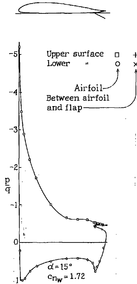
Figure 3. - Pressure distribution on the Clark Y-H airfoil at various angles of attack. 0.15 c_w split flap deflected 30^\circ .
