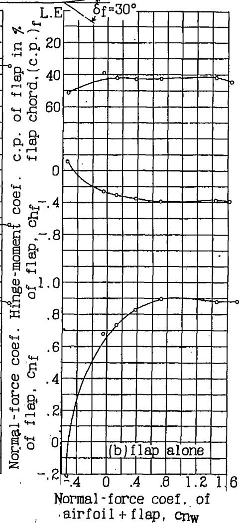
Figure 6.- Characteristics of Clark Y-H airfoil with 0.15 c_w split flap deflected 30°.
