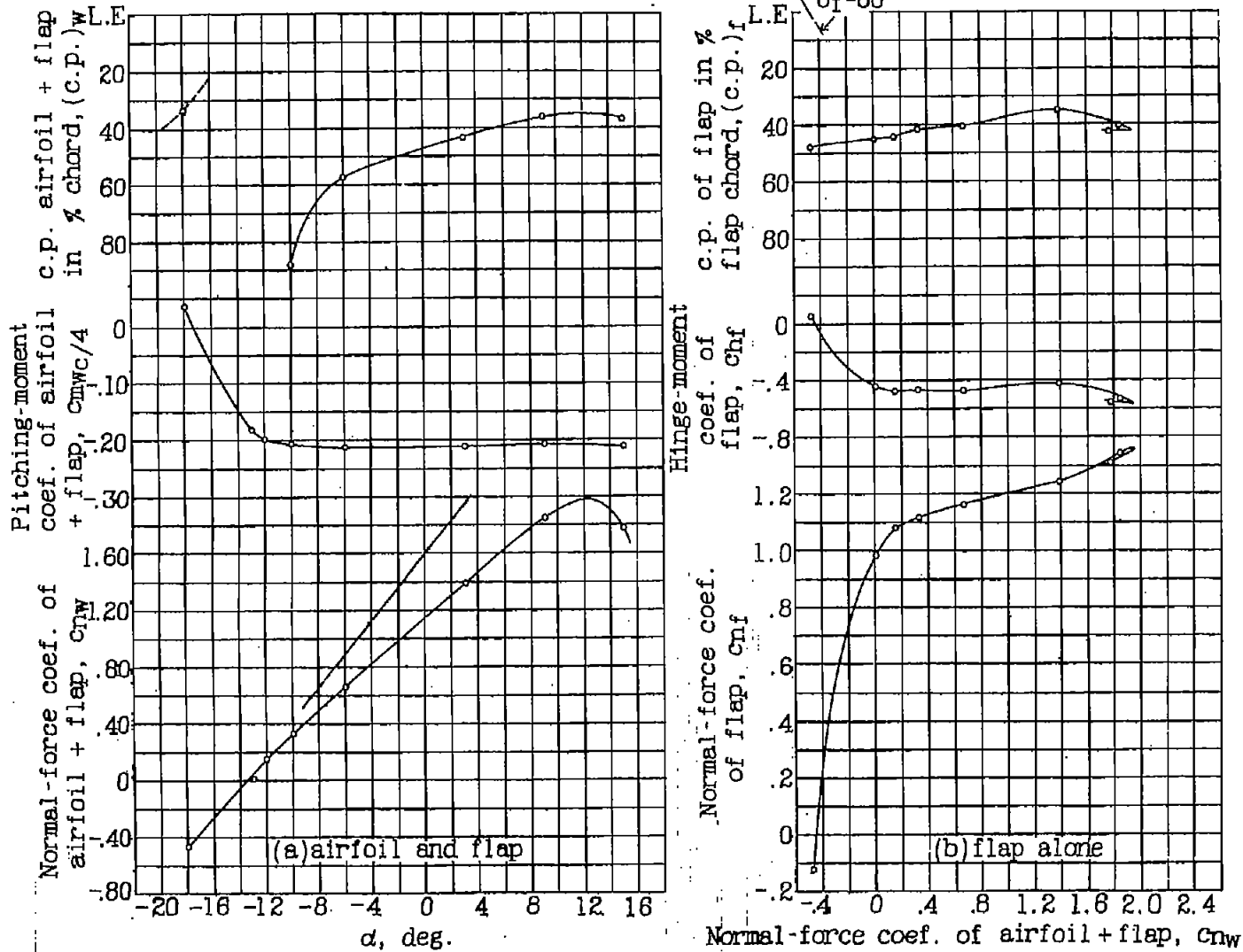
Figure 7.- Characteristics of Clark Y-H airfoil with 0.15 cw split flap deflected 60°.
