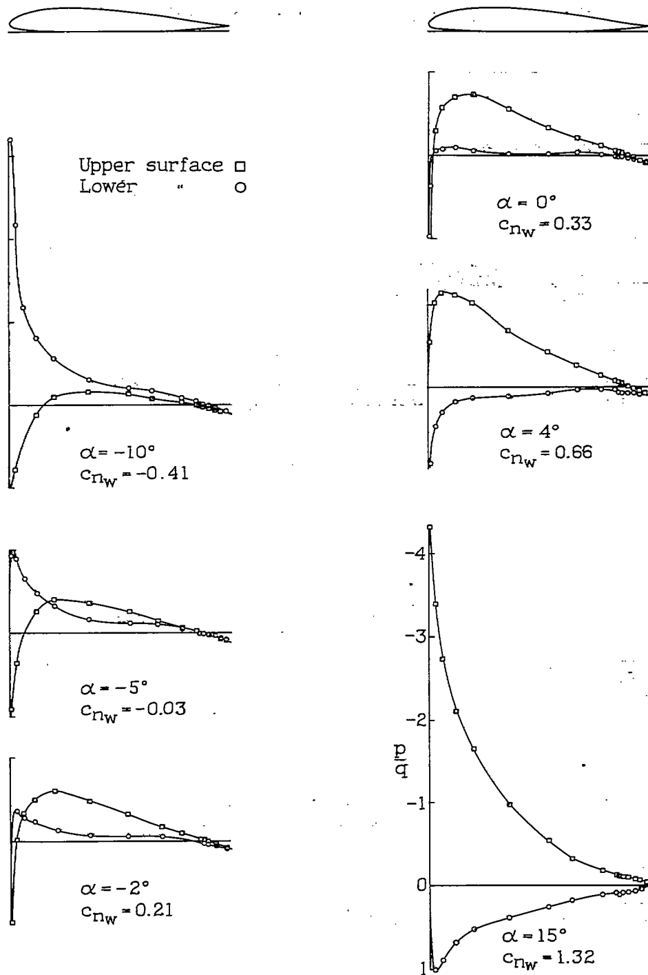
Figure 2.- Pressure distribution on the Clark Y-H airfoil at various angles of attack. Split flap neutral.
