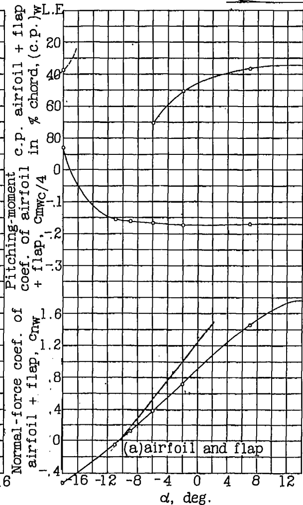
Figure 6.- Characteristics of Clark Y-H airfoil with 0.15 c_w split flap deflected 30°.
