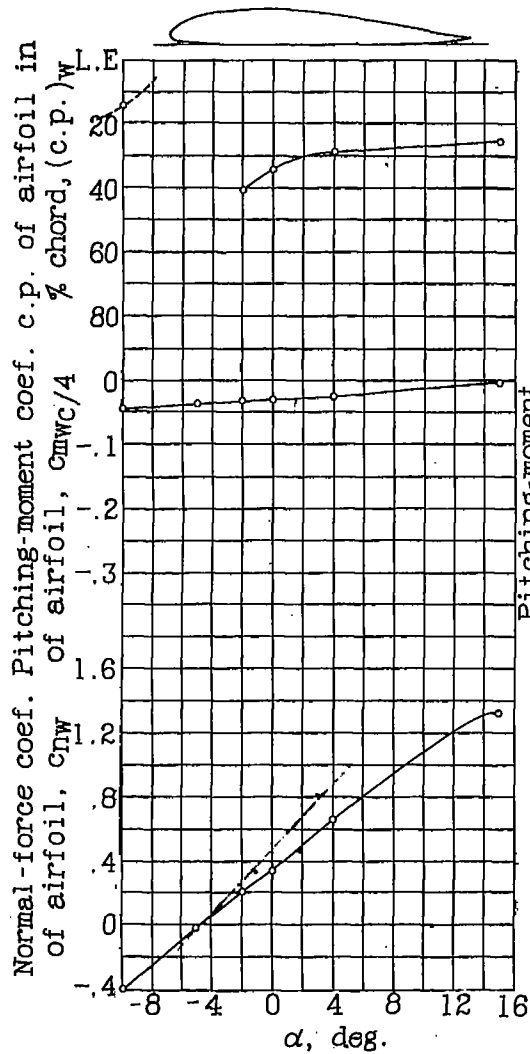
Figure 5.- Characteristics of Clark Y-H airfoil with flap neutral.
