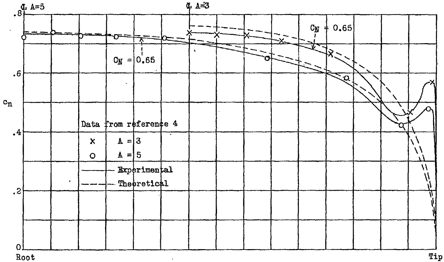
Figure 2.- Influence of aspect ratio on tip c_n distribution.
