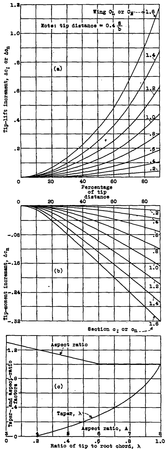
Figure 3.- Tip corrections.
