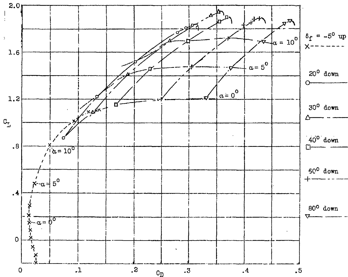
Figure 3.- Polar curves for wing with flap at position 0 1. Slot 5 D.
