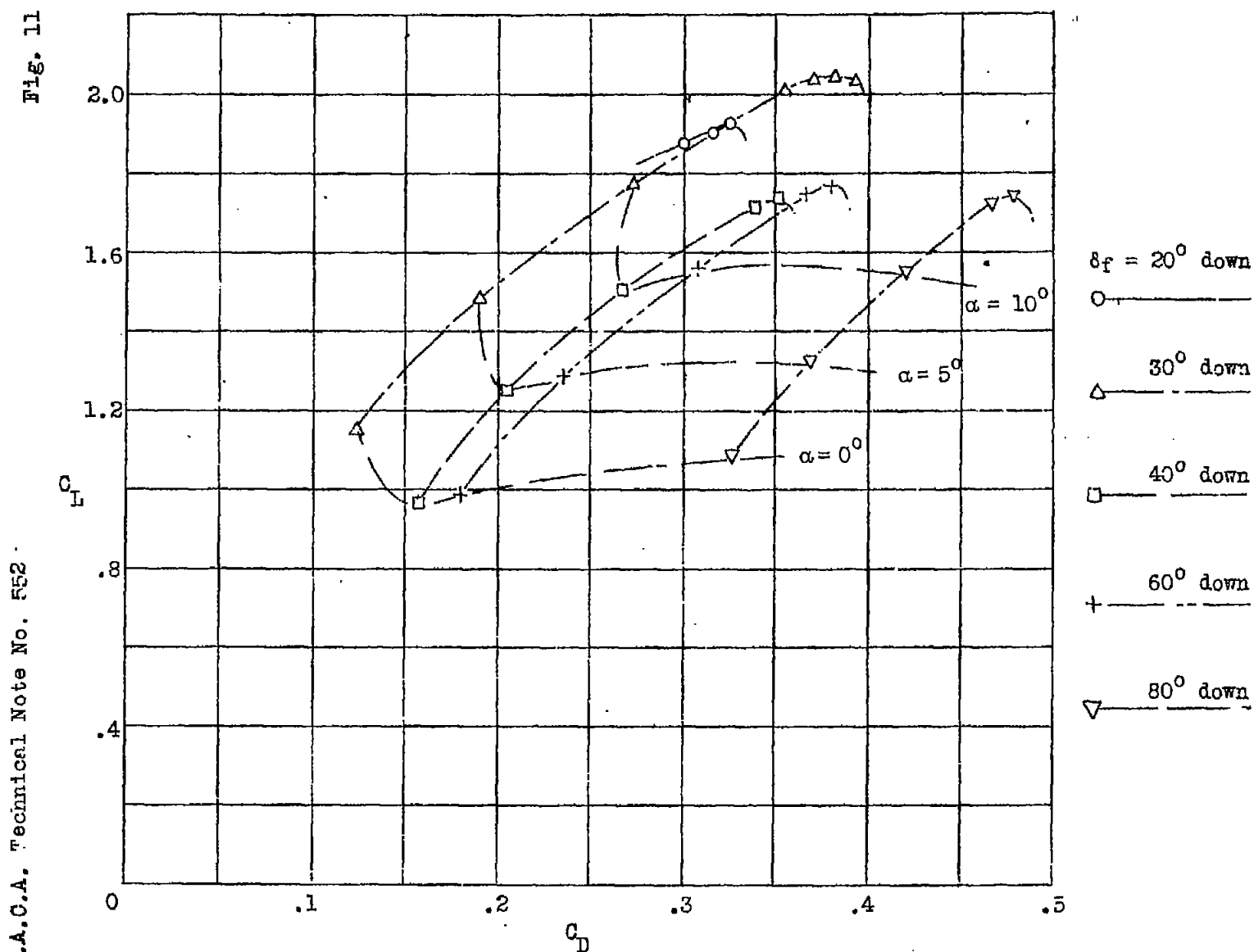
Figure 11.-Polar curves for wing with flap at position A1. Slot 6.
