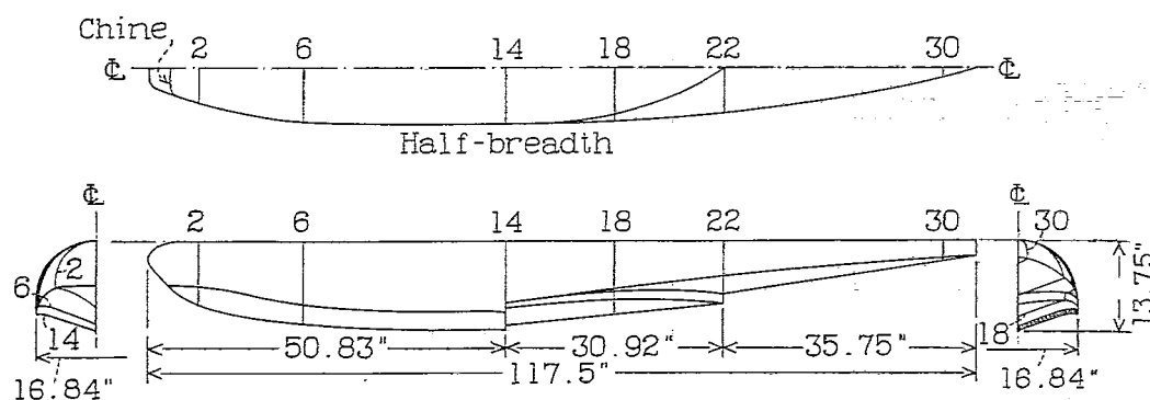
Figure 6.- Lines of N.A.C.A. Model 18.
