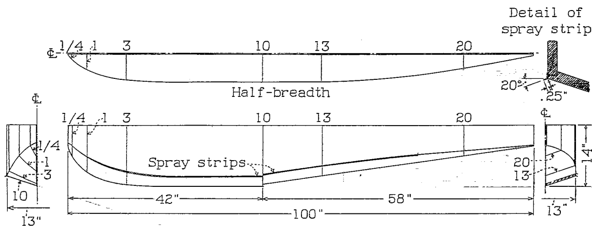
Figure 10.- Lines of N.A.C.A. Model 36.
