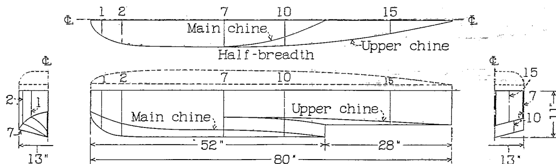
Figure 9.- Lines of N.A.C.A. Model 35.
