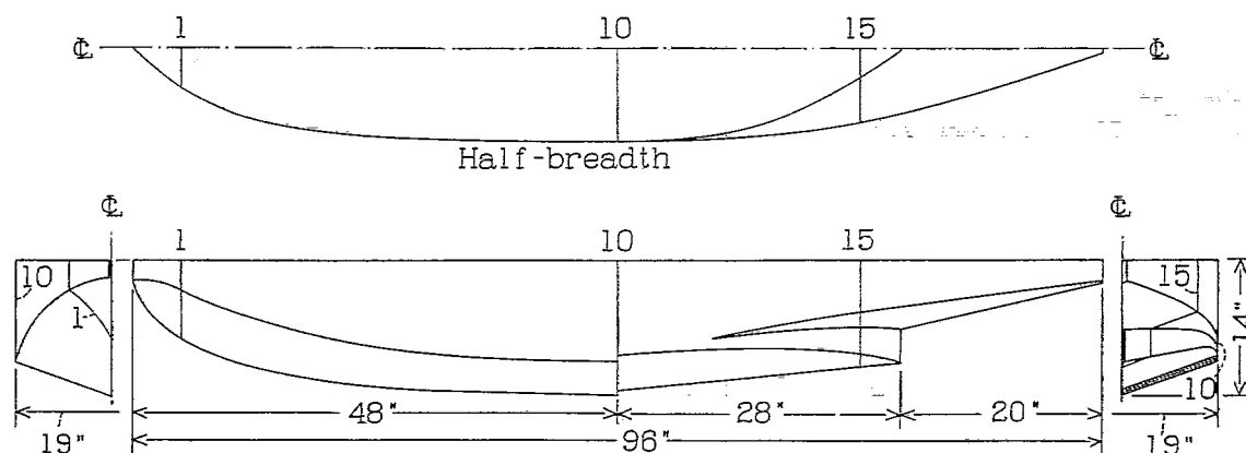
Figure 4.- Lines of N.A.C.A. Model 14.
