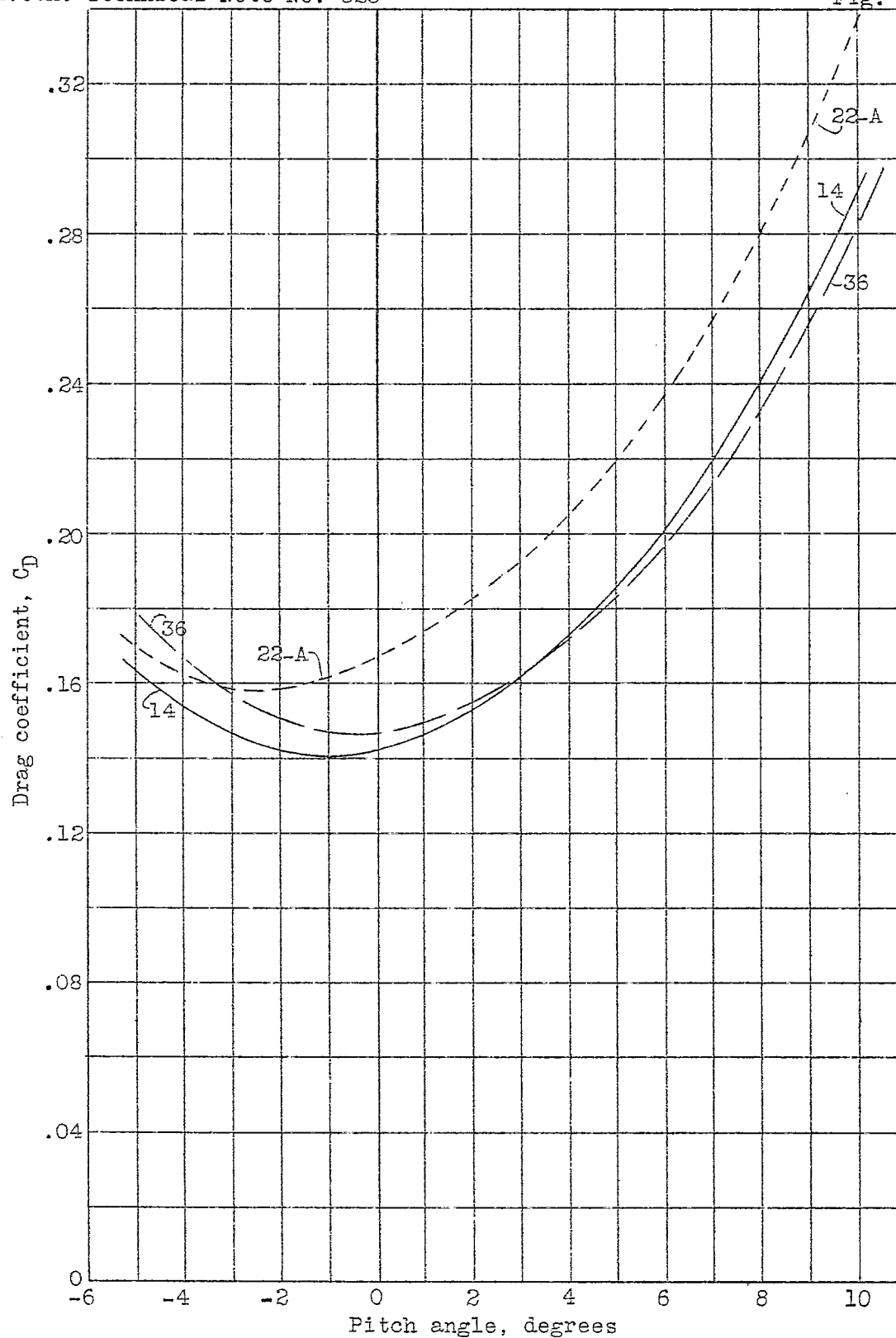
Figure 14.--The drag coefficients of hulls with flat decks.
