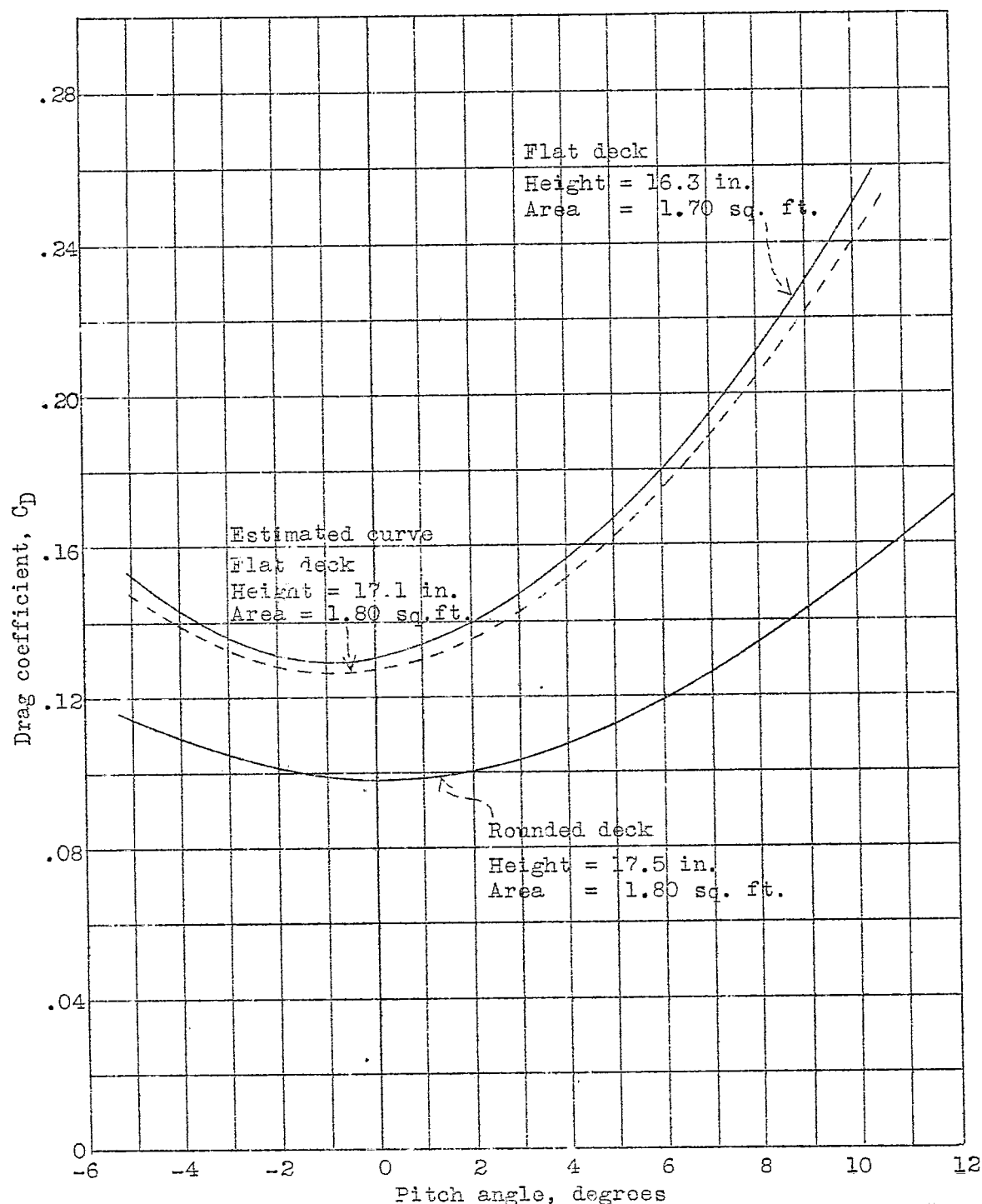
Figure 18.-The variation of drag coefficient of model 11-A with flat and rounded decks.
