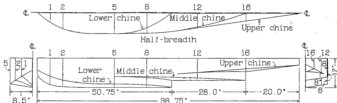
Figure 7.- Lines of N.A.C.A. Model 22-A
