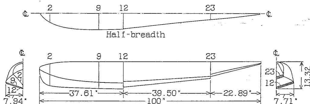
Figure 5.- Lines of N.A.C.A. Model 16.
