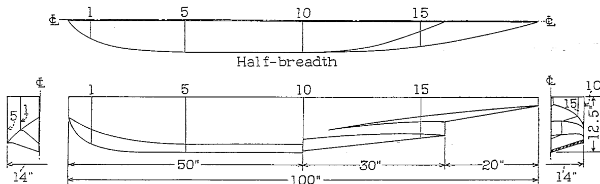
Figure 10.- Lines of N.A.C.A. Model 36.
