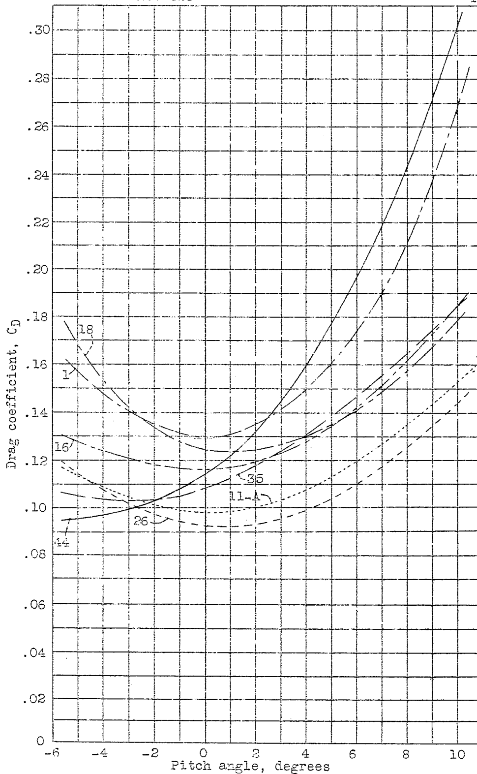
Figure 13.-The drag coefficients of hulls with rounded decks.
