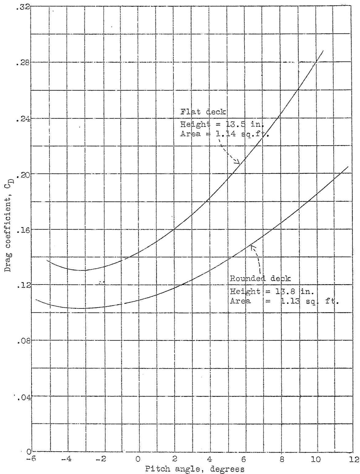
Figure 17.-The variation of drag coefficient of model 35 with flat and rounded decks.
