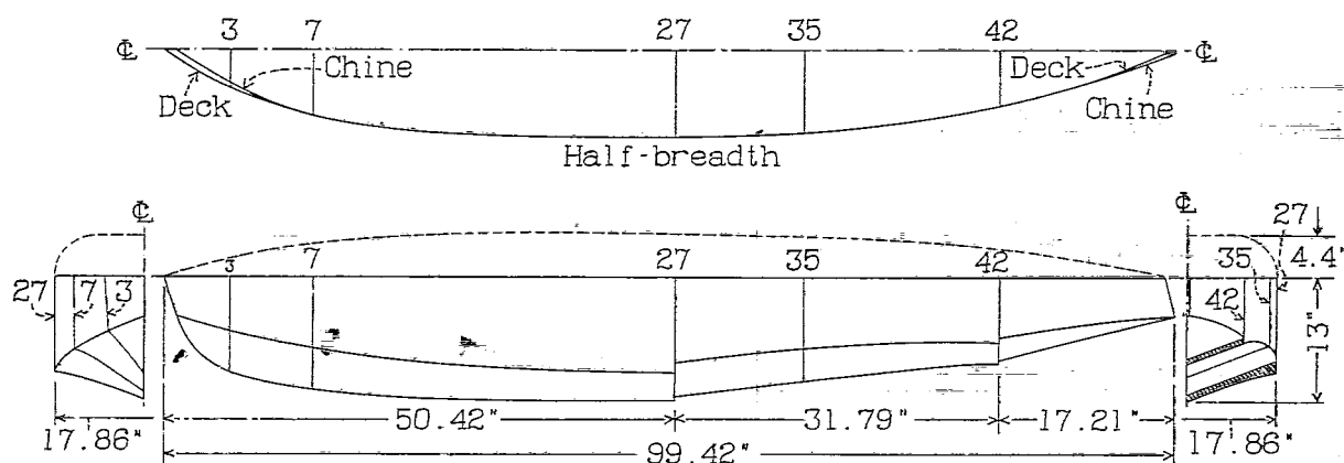
Figure 8.- Lines of N.A.C.A. Model 26.
