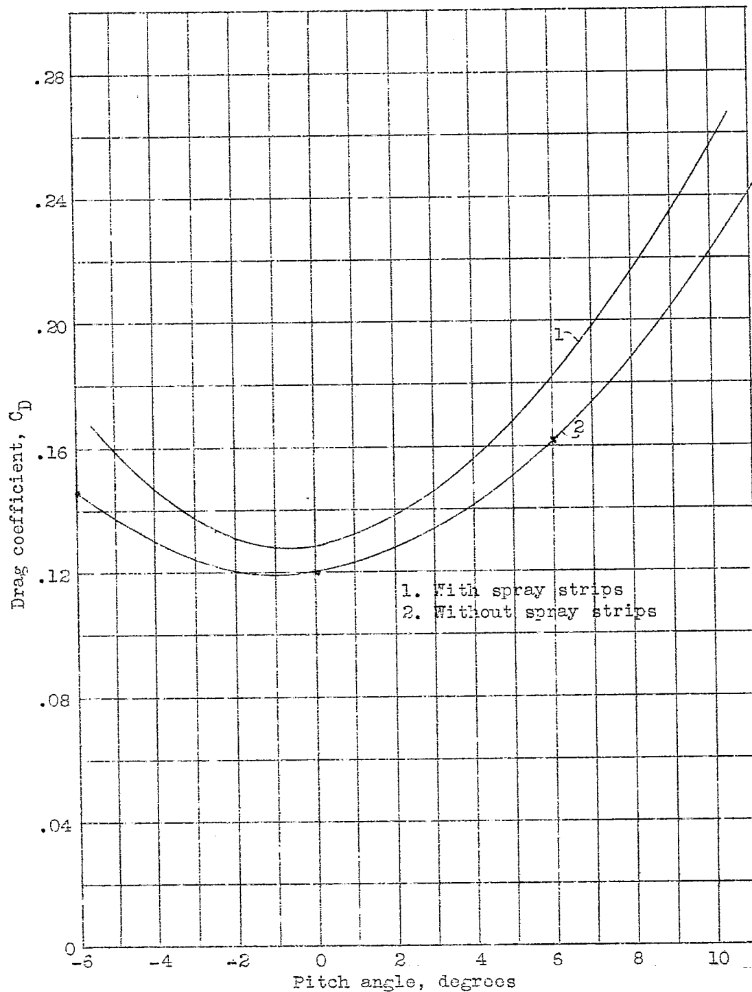
Figure 21.--The variation of the drag coefficient of model 40 with the addition of spray strips.
