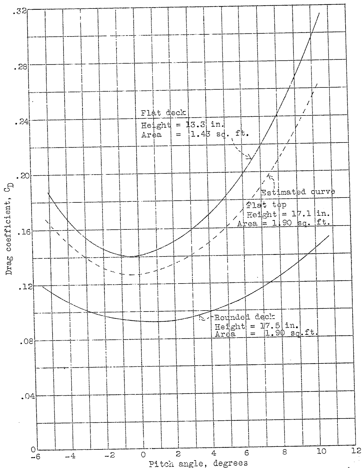
Figure 19.-The variation of drag coefficient of model 26 with flat and rounded decks.
