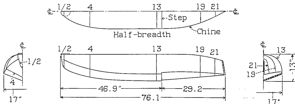
Figure 12.- Lines of N.A.C.A. Model 44.
