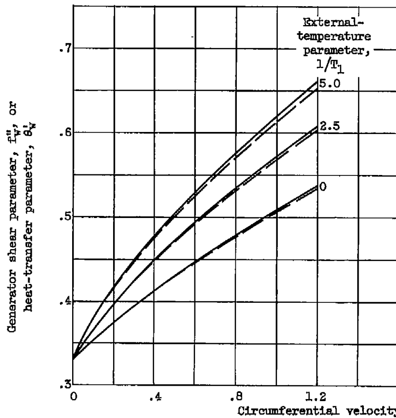
Figure 2. - Continued. Shear and heat-transfer parameters from exact and approximate solutions in plane of symmetry.
