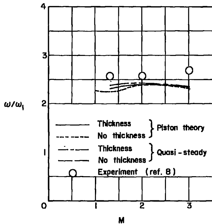
Figure 5.- Calculated flutter frequency ratio and stiffness-altitude parameter compared with experiment for a flat-plate 60^\circ delta wing.
