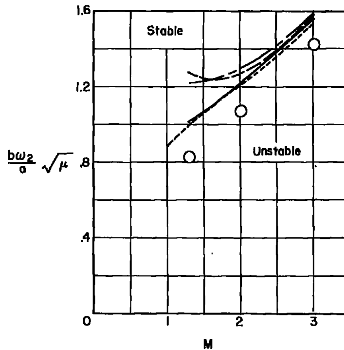
Figure 5.- Calculated flutter frequency ratio and stiffness-altitude parameter compared with experiment for a flat-plate 60^\circ delta wing.
