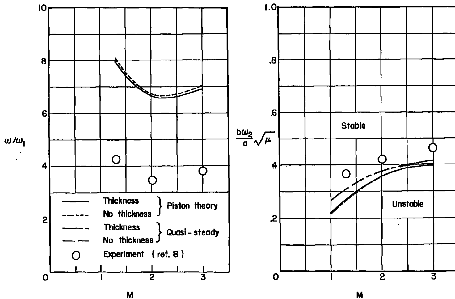
Figure 7.- Calculated flutter frequency ratio and stiffness-altitude parameter compared with experiment for a flat-plate 45° swept wing.
