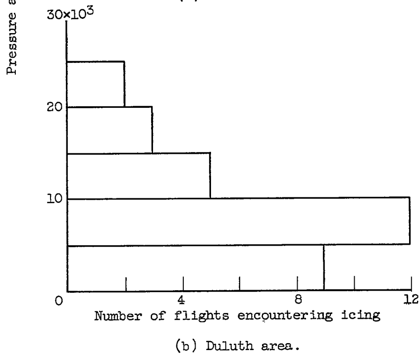
Figure 3. - Histogram of altitude distribution of icing encountered during climb and descent.
