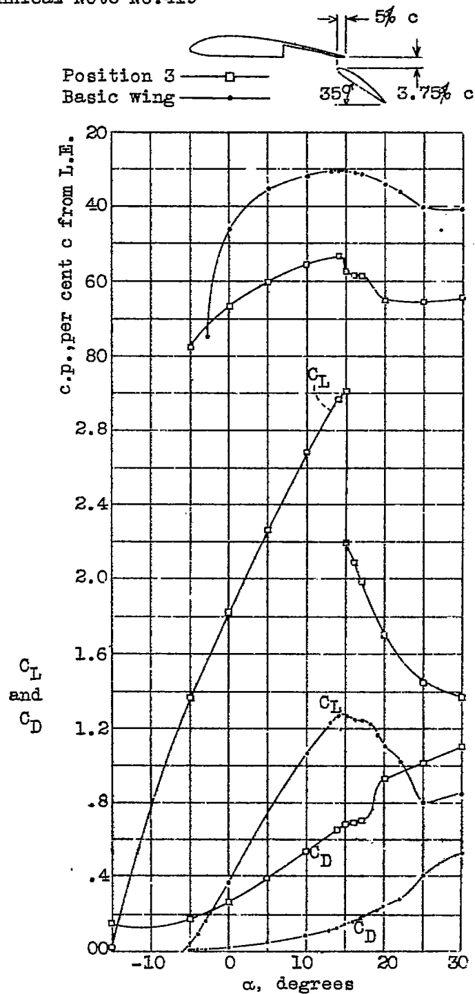
Fig.9 C_L , C_D and c.p. curves for position 3.
