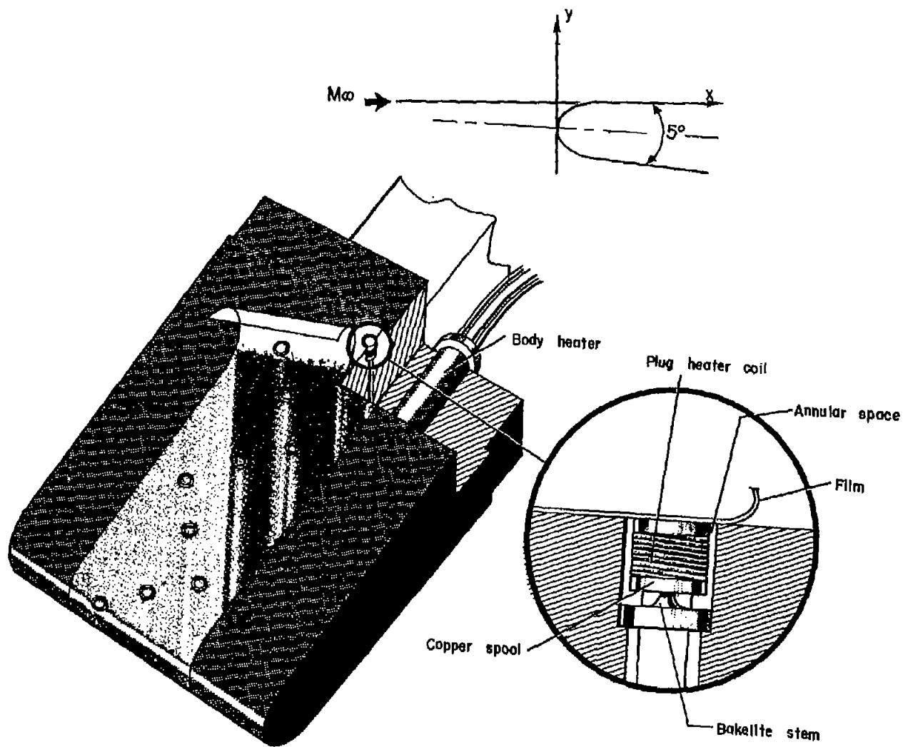
Figure 3.- Heat-transfer body.
