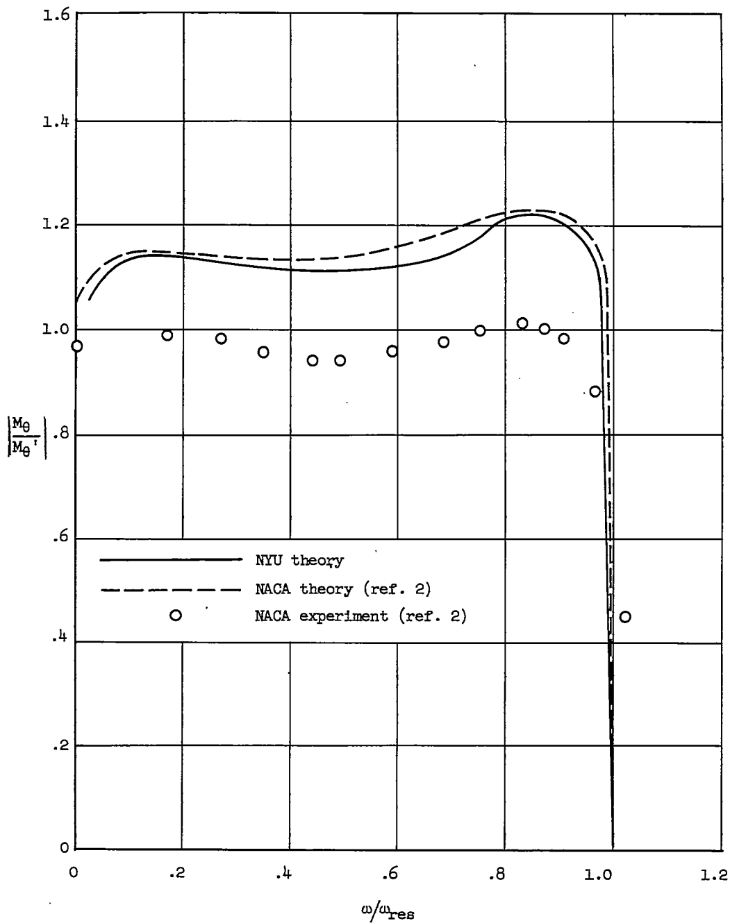
Figure 5.- Effect of cascade or of tunnel walls on moment amplitude for pure pitching about midchord (moment is about midchord). |M_\theta| = Moment amplitude in cascade; |M_\theta^i| = Moment amplitude of isolated blade; \sigma = 180^\circ ; M = 0.5 ; s/b = 7.60 ; s^* = 0 .
