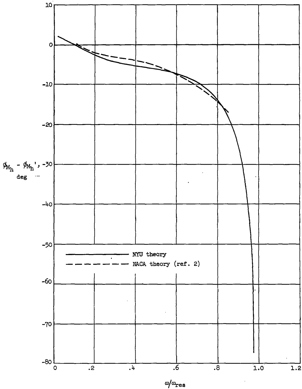
Figure 10.- Effect of cascading or of tunnel walls on moment (about midchord) phase angle for pure translatory motion. \phi_{M_{12}} = Cascade moment phase angle; \phi_{M_{12}}' = Single-wing moment phase angle; \sigma = 180^\circ ; M = 0.5 ; s/b = 7.60 ; s^* = 0 .
