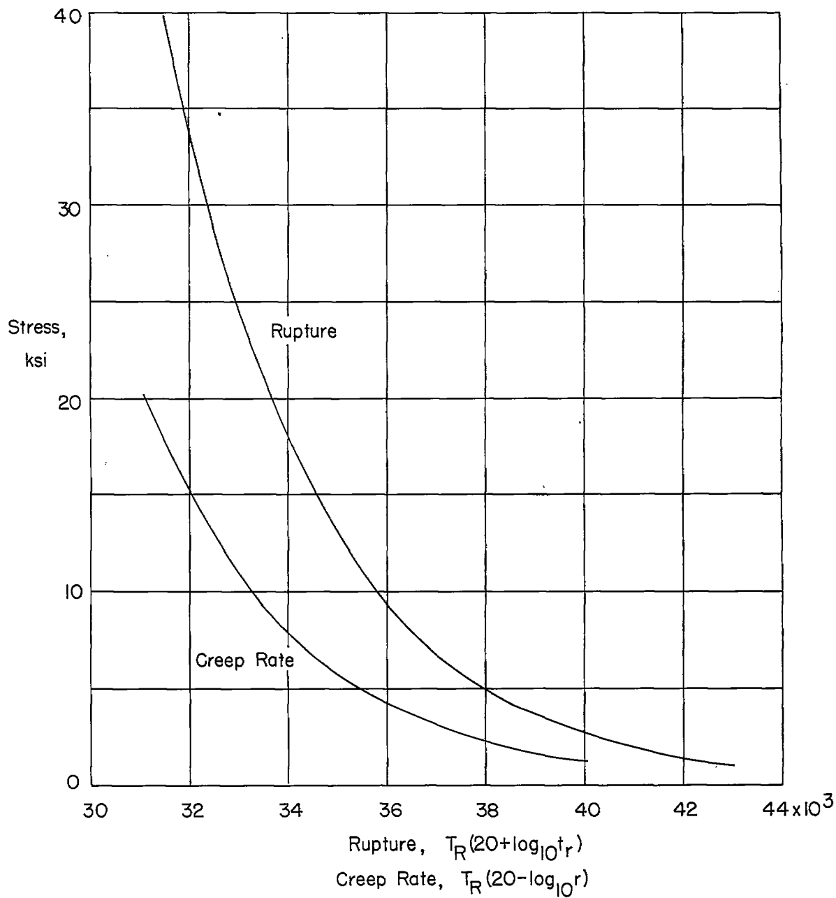
(d) Carbon-molybdenum steel (temperature range of data from 900° to 1200° F; data from ref. 1).
