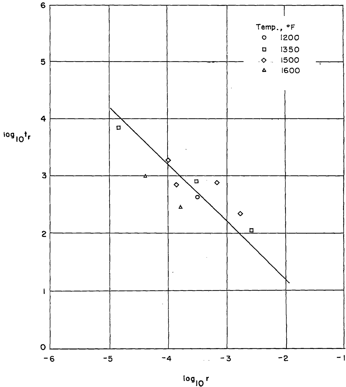
(g) Inconel X (data from ref. 15).
