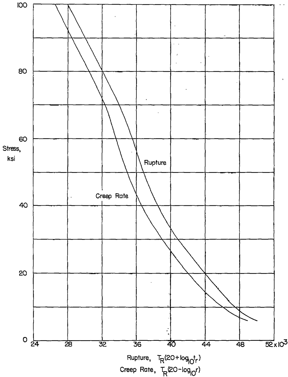
(f) S-590 alloy (temperature range of data from 1200° to 1900° F; curves from ref. 1).
