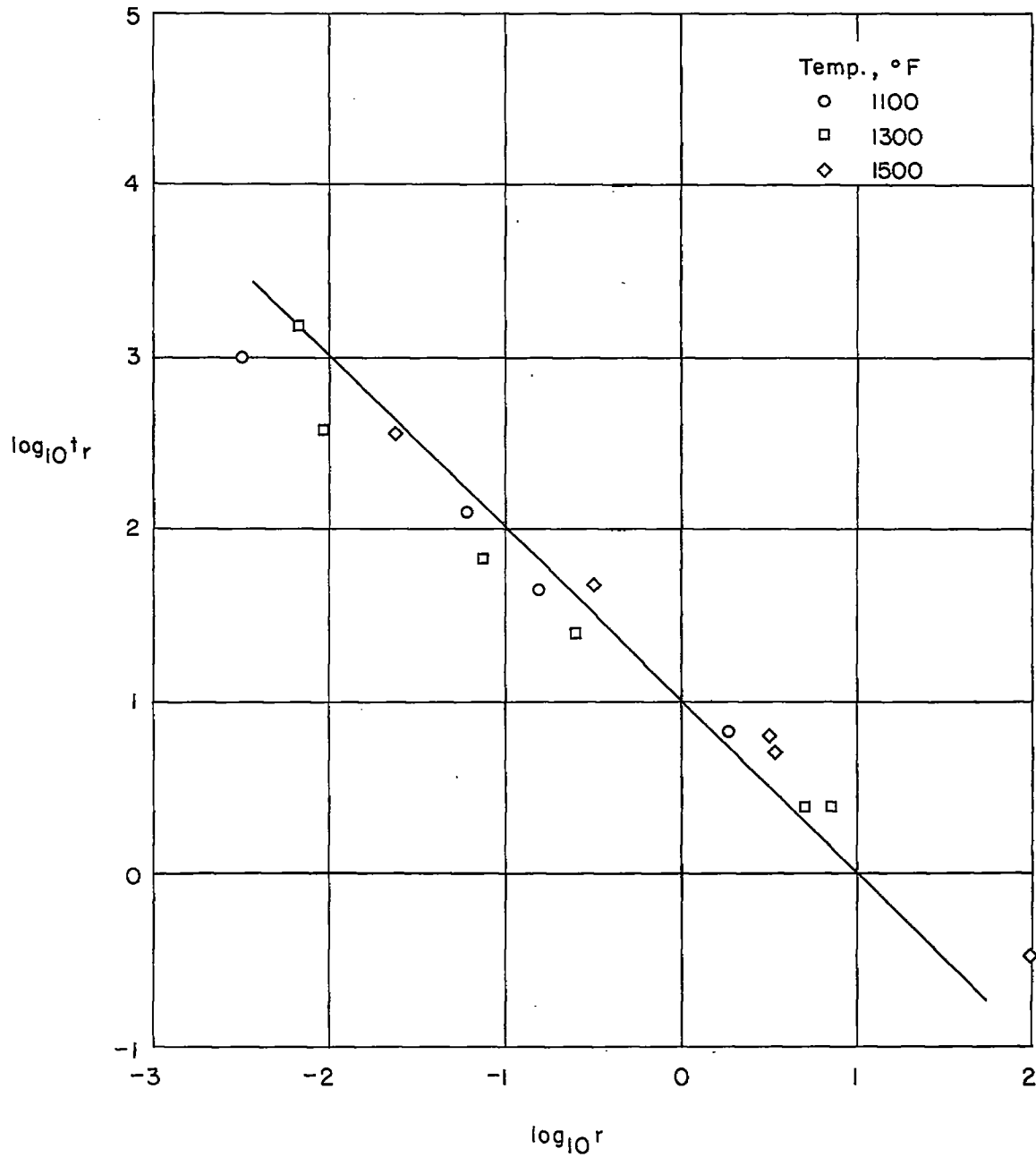
(e) 18-8 Cb stainless steel (data from ref. 14).
