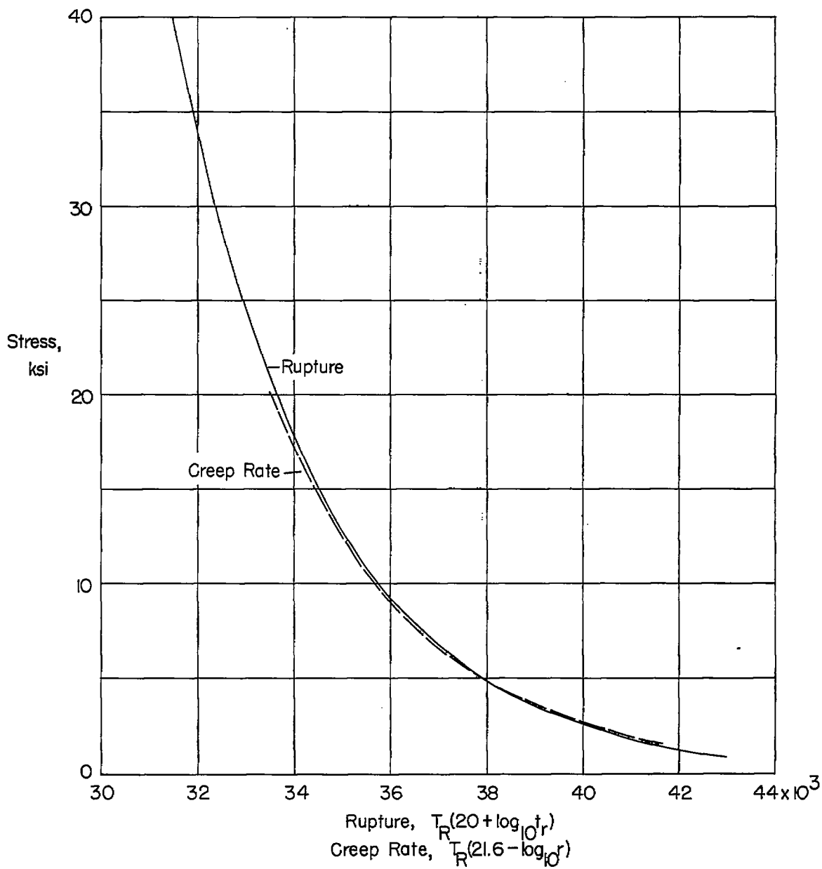
(d) Carbon-molybdenum steel (temperature range of data from 900° to 1200° F).
