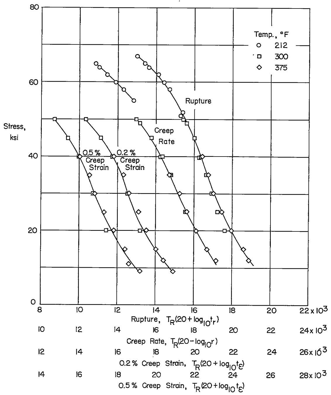
(c) 7075-T6 clad aluminum-alloy sheet (data from ref. 13).
