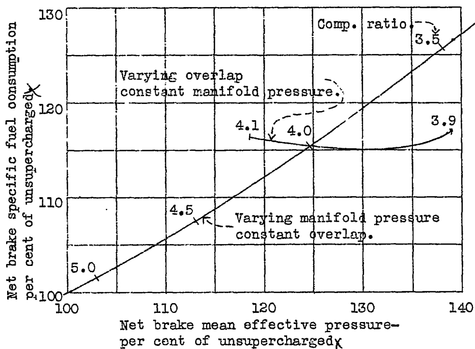
Fig. 9 Variation in net brake specific fuel consumption as supercharger pressure is increased at highest useful compression ratio for each pressure. (40° overlap)
