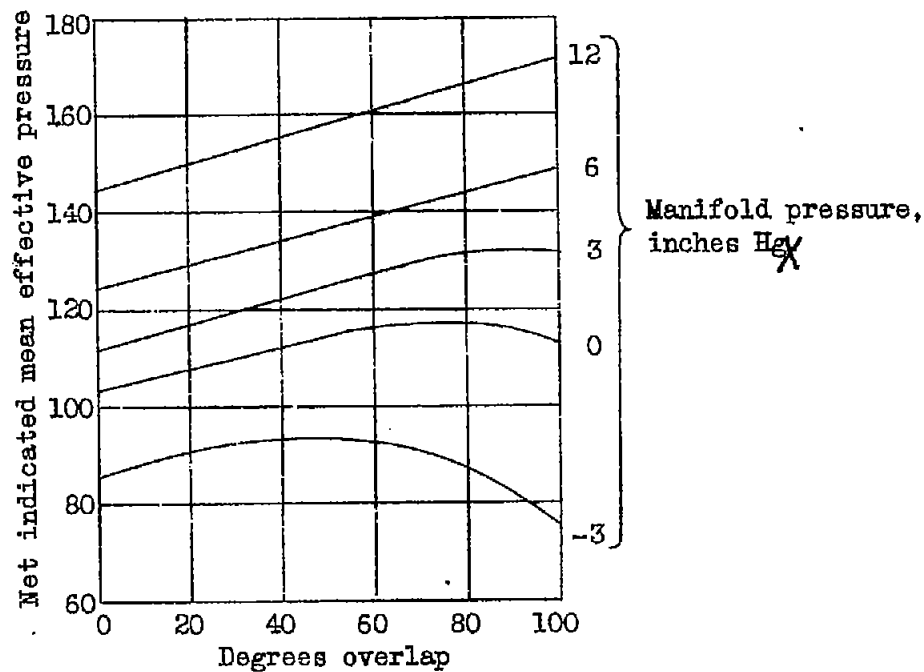
Fig. 3 Variation of net indicated mean effective pressure with overlap
