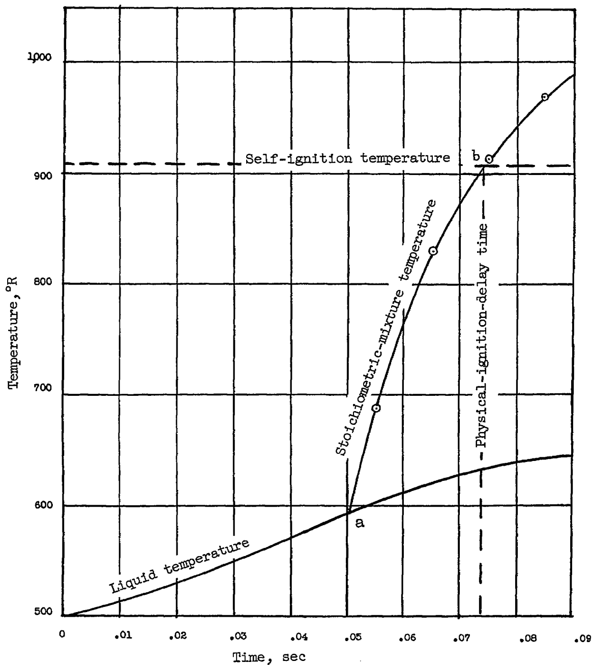
Figure 19.- Stoichiometric-mixture temperature against time for n-decane; self-ignition temperature, 909° R. Air temperature, 1,200°; air velocity, 100 inches per second; initial drop radius, 500 microns.
