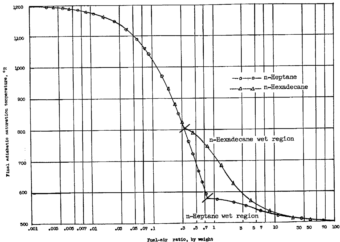
Figure 16.- Overall fuel-air ratio versus final adiabatic saturation temperature for n-heptane and n-hexadecane. Air temperature, 1,200° R; initial fuel temperature, 500° R.
