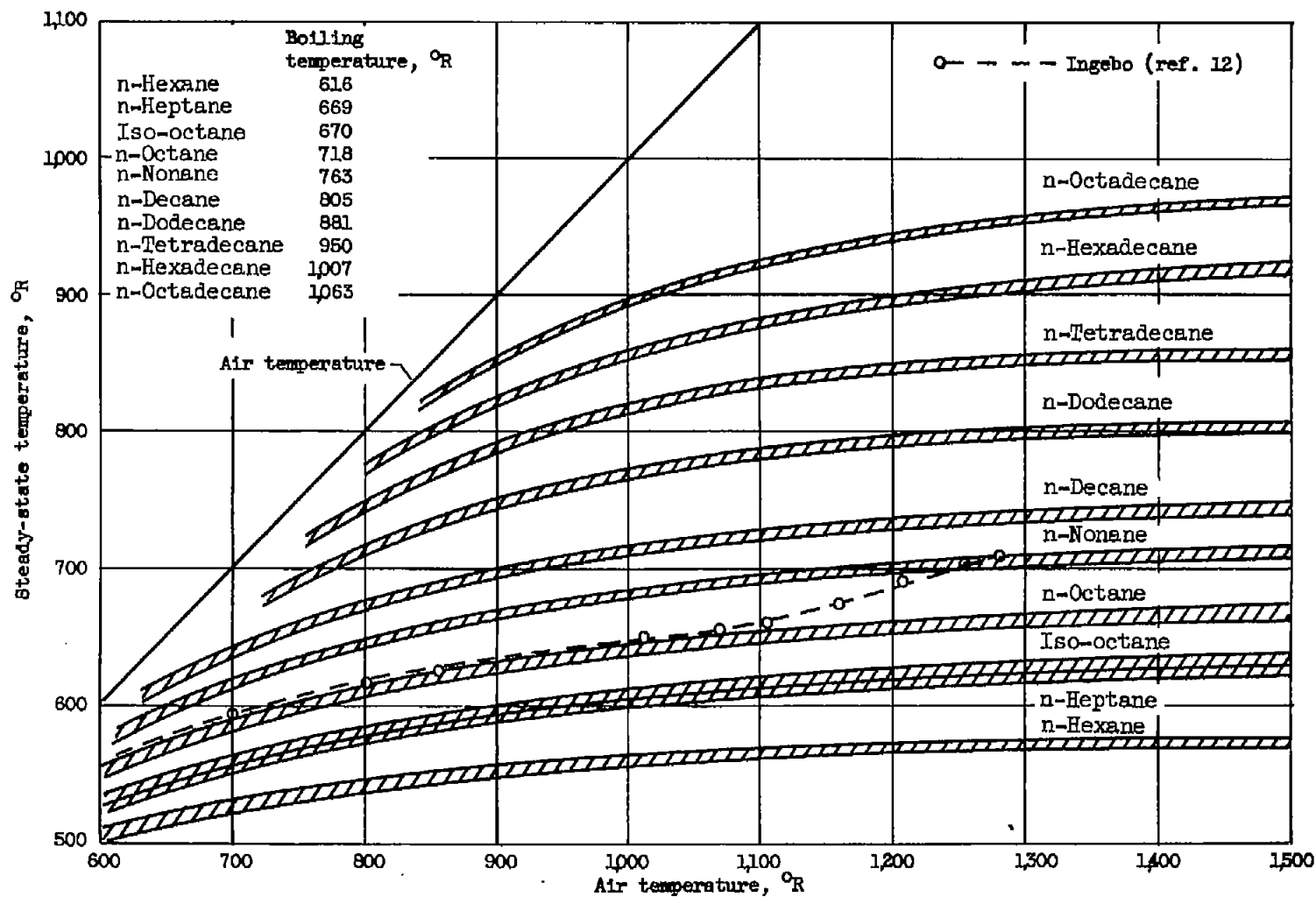
Figure 7.- Experimental steady-state temperature as a function of air temperature for various fuels.
