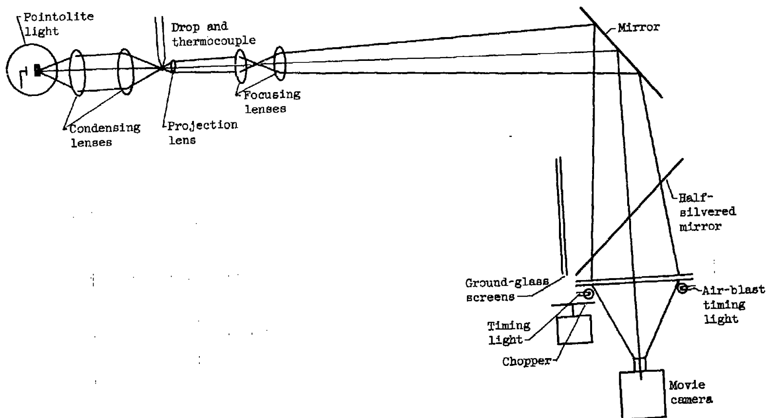
Figure 2.- Schematic diagram of optical system.
