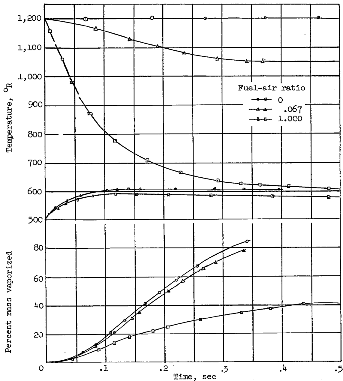
(a) n-heptane.
