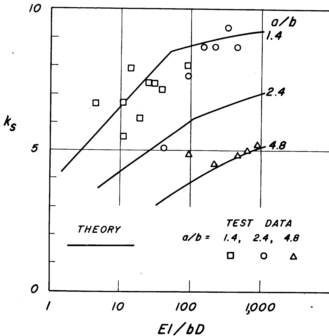
(b) Simply supported plates; transverse stiffeners.
