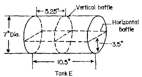
(b) Circular-cylinder tank. Fineness ratio, 1.5.
