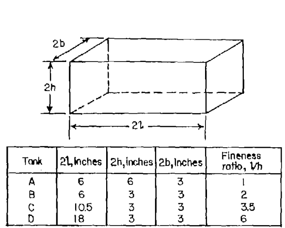
(a) Rectangular tanks.
