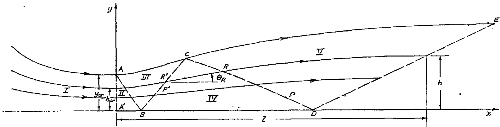
(a) Streamlines and flow regions for some typical nozzles.
