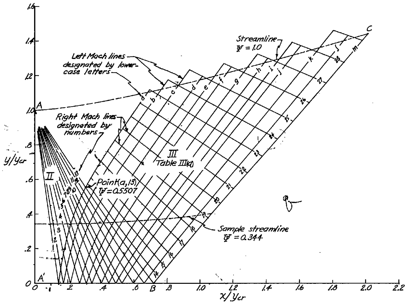
(a) \nu_B = 6^\circ .
