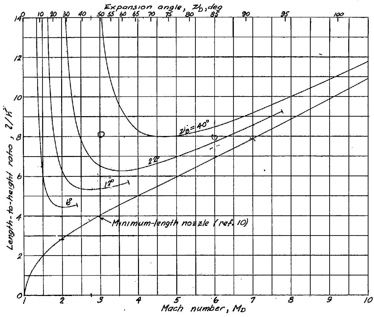
Figure 3.- Nozzle design parameters, where for given values of M_D and v_B the four upper curves give the shortest possible nozzle by the present method.
