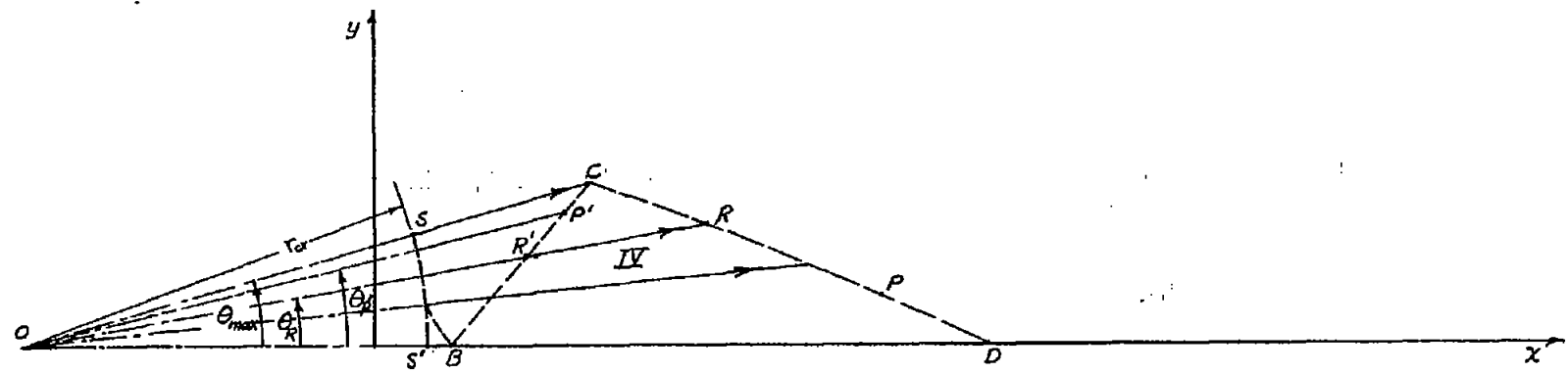
(b) Sonic arc and other radial-flow parameters, shown to the same scale as that of figure 1(a).
