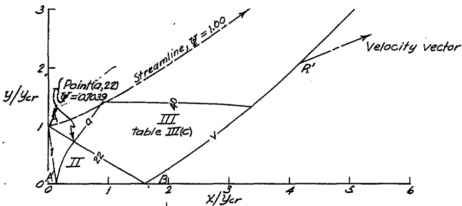
(c) v_B = 22^\circ .
