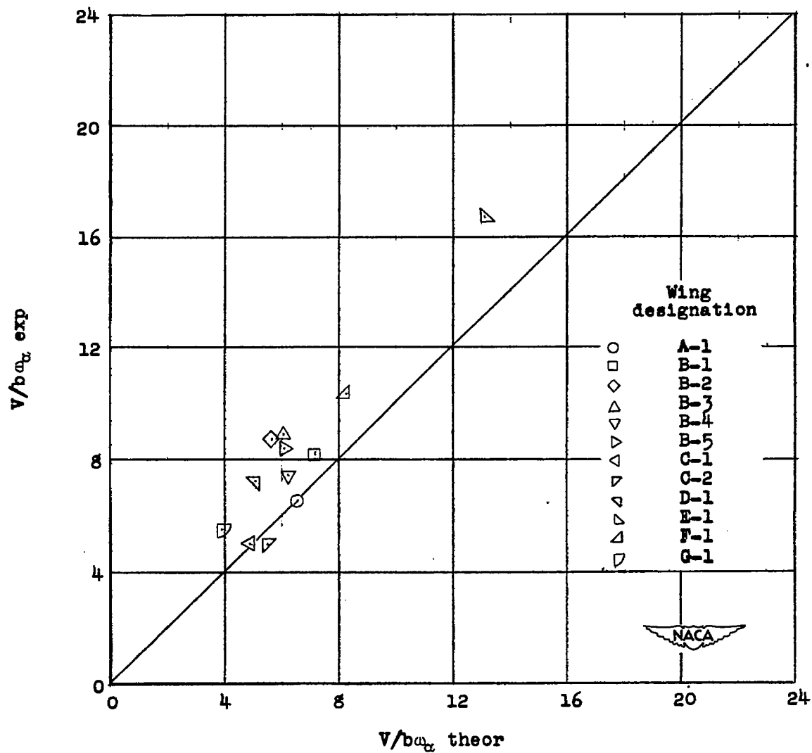
Figure 6.- Comparison of experimental values of V/b\alpha_x to theoretical values of V/b\alpha_x at M = 1.3 .
