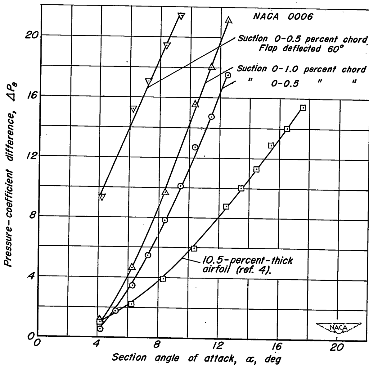
Figure 22.-Comparison of the pressure-coefficient difference between the leading and trailing edges of the porous area on the NACA 0006 and the symmetrical 10.5-percent-thick airfoils; c_D=0.0016 ; V_0=162 fps.
