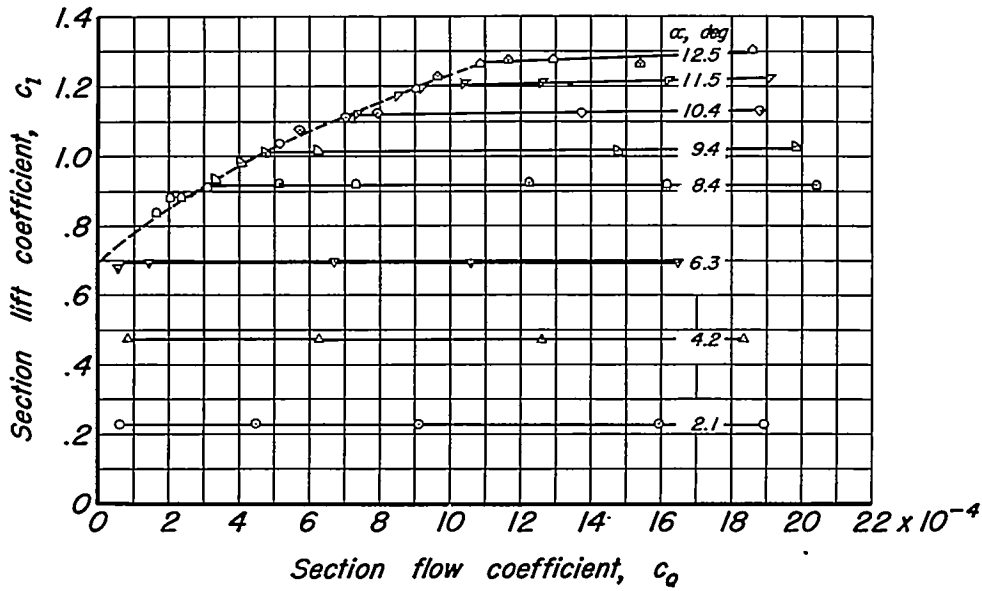
(a) Constant angle of attack.
