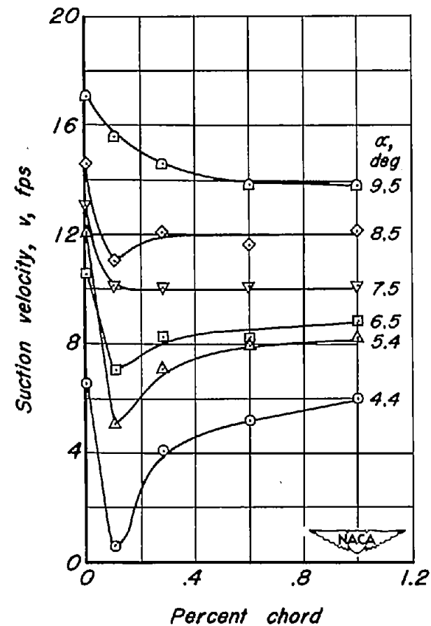
Figure 18.-Flow requirements and stall-point suction-velocity distributions for the model with tapered permeability from 0- to 1-percent chord and a 0.2-chord split flap deflected 60^\circ ; V_0 = 133 fps.
