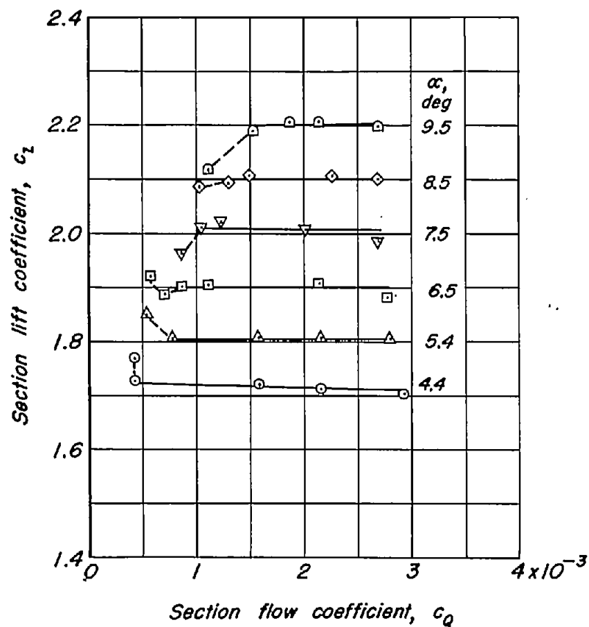
Figure 18.-Flow requirements and stall-point suction-velocity distributions for the model with tapered permeability from 0- to 1-percent chord and a 0.2-chord split flap deflected 60^\circ ; V_0 = 133 fps.
