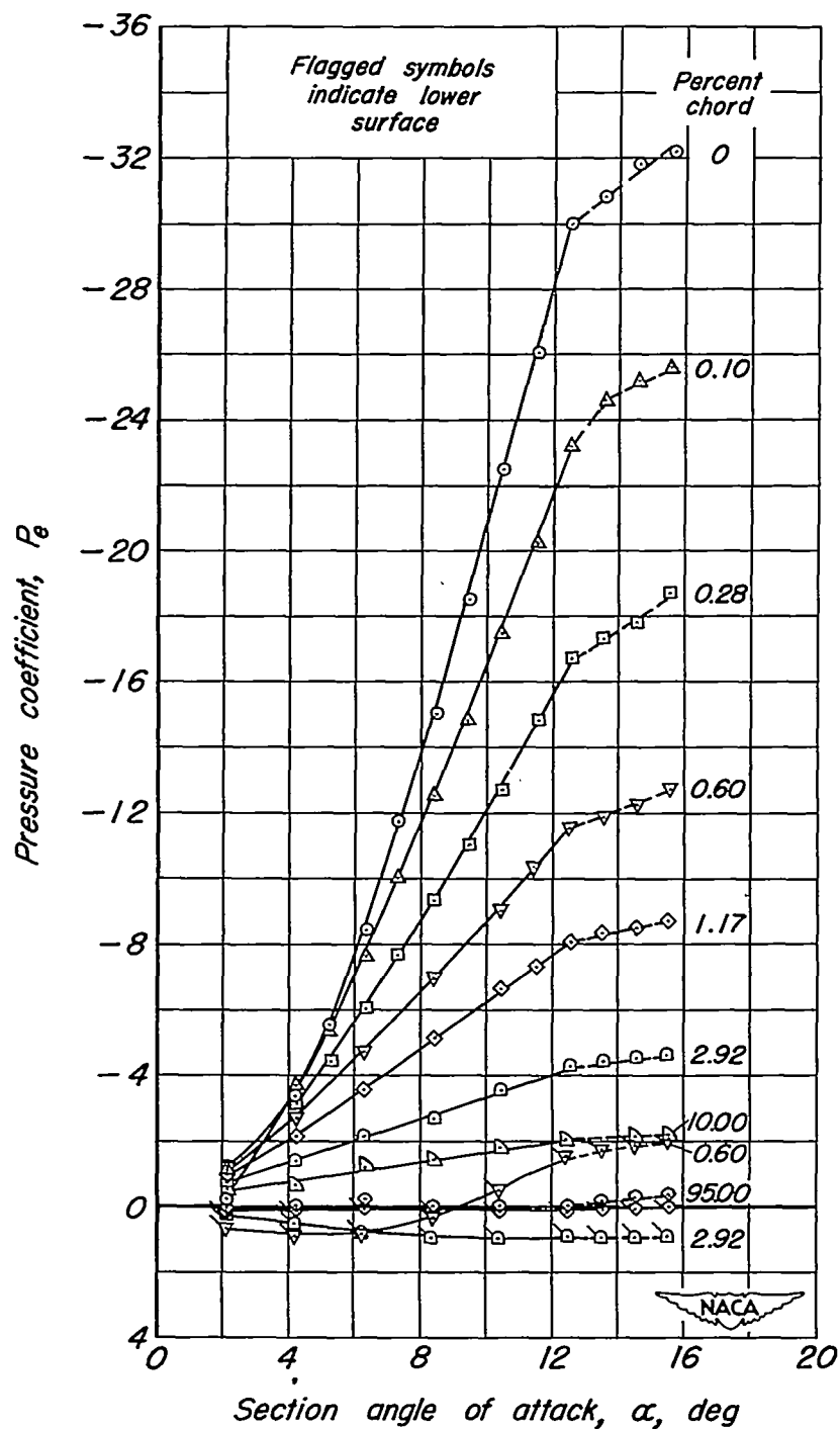
Figure 12.-Variation of the pressure coefficients at particular chordwise stations with angle of attack for the model with tapered permeability from 0- to 1-percent chord; c_Q=0.0016 ; V_0=162 fps.
