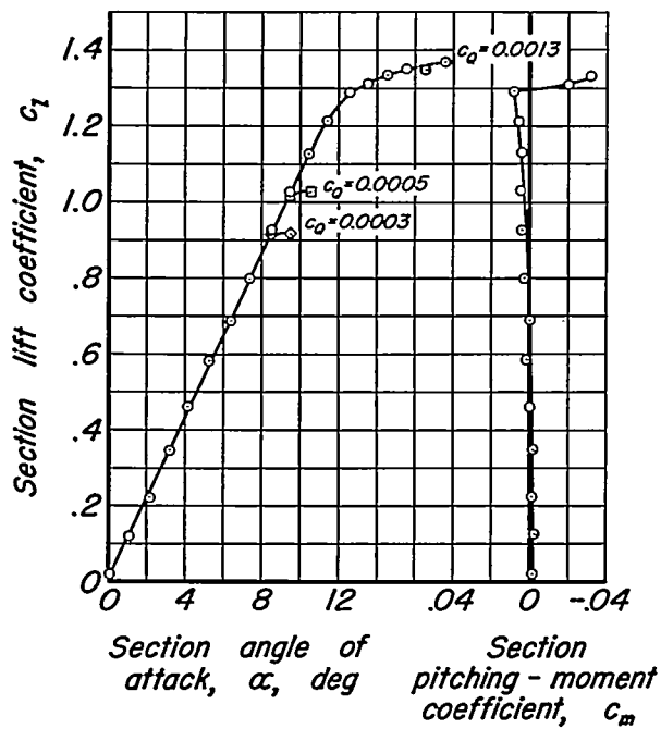
(b) Constant section flow coefficient.
