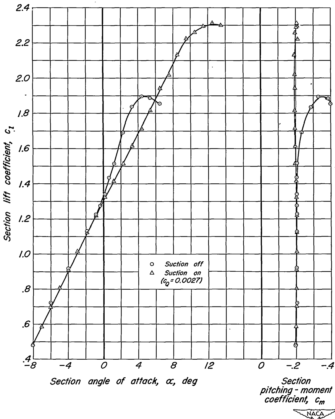
Figure 17.- Lift and moment characteristics of the model with tapered permeability from 0-to 1-percent chord and a 0.2-chord split flap deflected 60^\circ ; V_0 = 133 fps.
