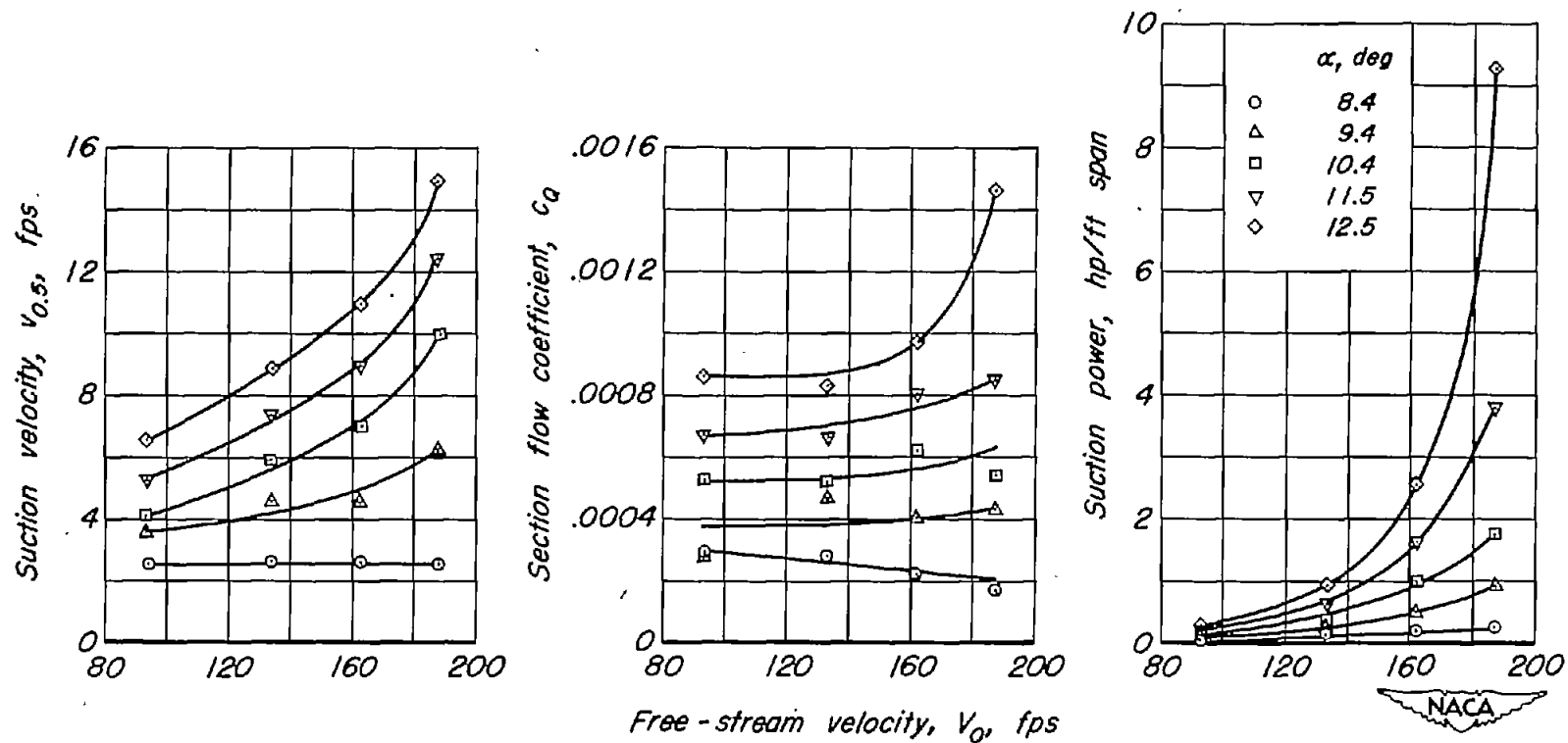
Figure 15.-Effect of free-stream velocity on the stall-point suction requirements of the model with tapered permeability from 0-to 1-percent chord.
