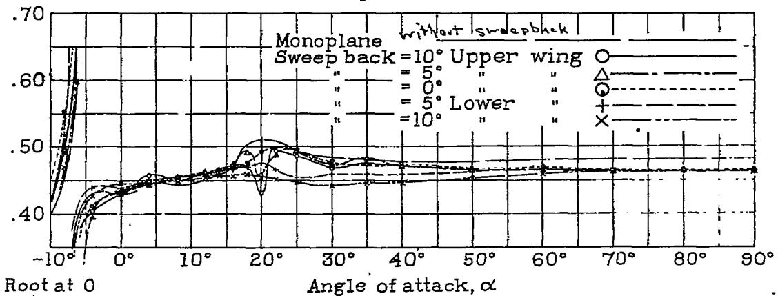
Fig. 28 Effect of sweep back on lower wing lateral center of pressure.
