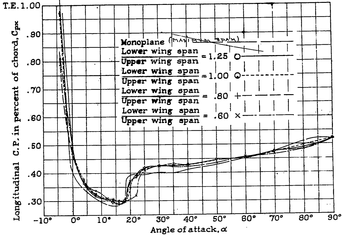
Fig.35 Effect of overhang on lower wing longitudinal center of pressure.
