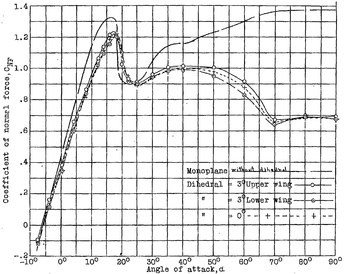
Fig. 12 Effect of dihedral on cellule coefficient of normal force.
