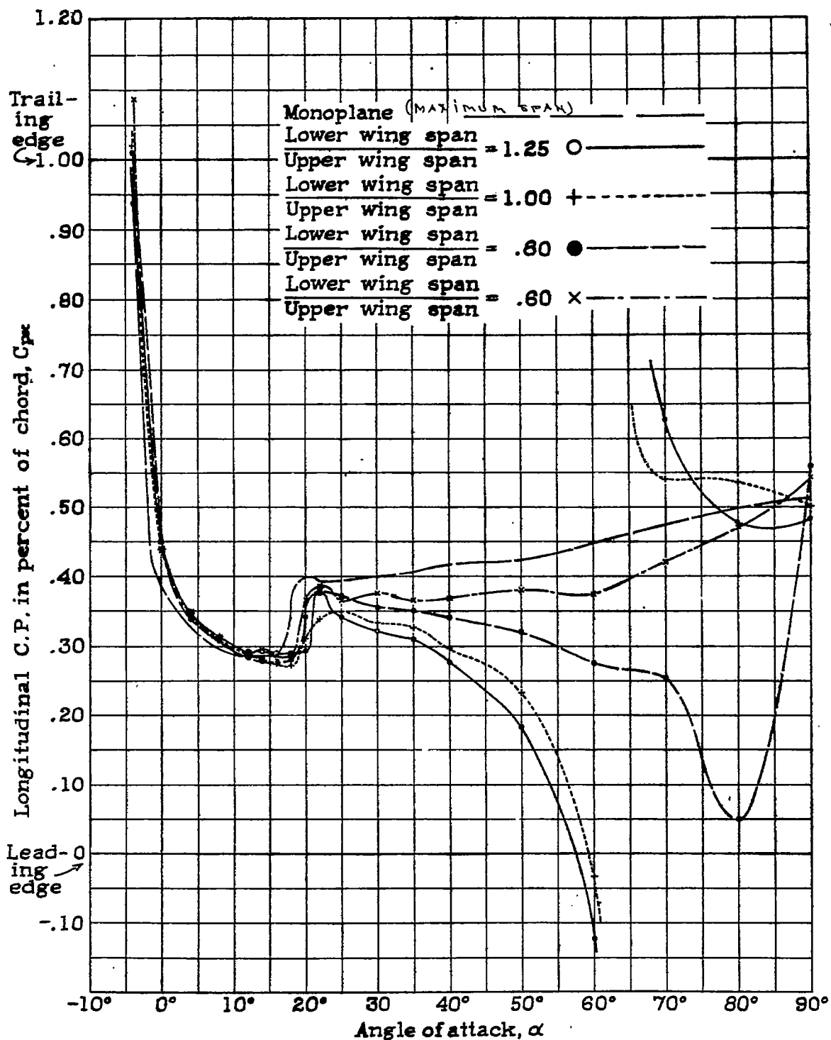
Fig. 34 Effect of overhang on upper wing longitudinal center of pressure.
