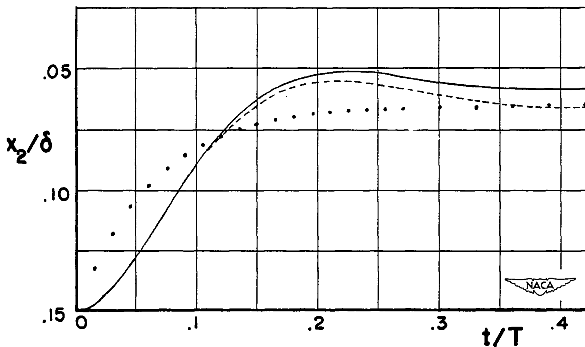
Figure 8.- Displacement of wheel when obstacle is encountered during taxiing.
