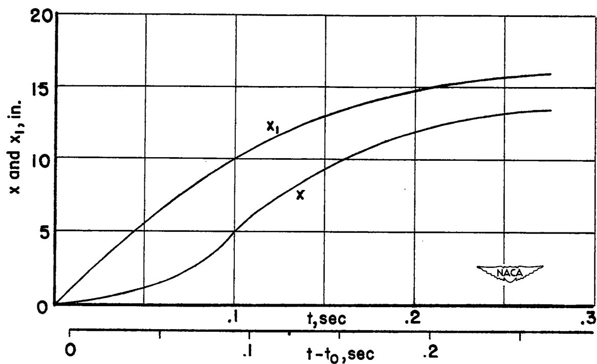
Figure 14.- Displacement x_1 and stroke x against time.
