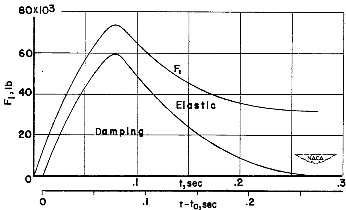
Figure 15.- Force-time history of shock strut.
