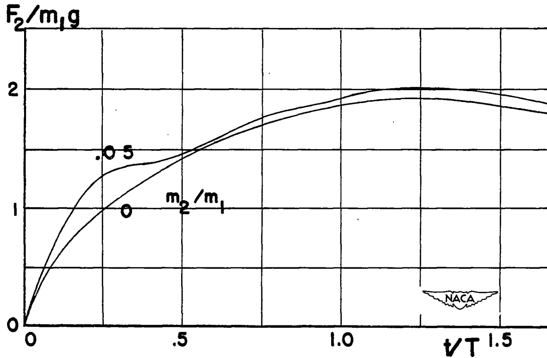
(b) On impact force.
