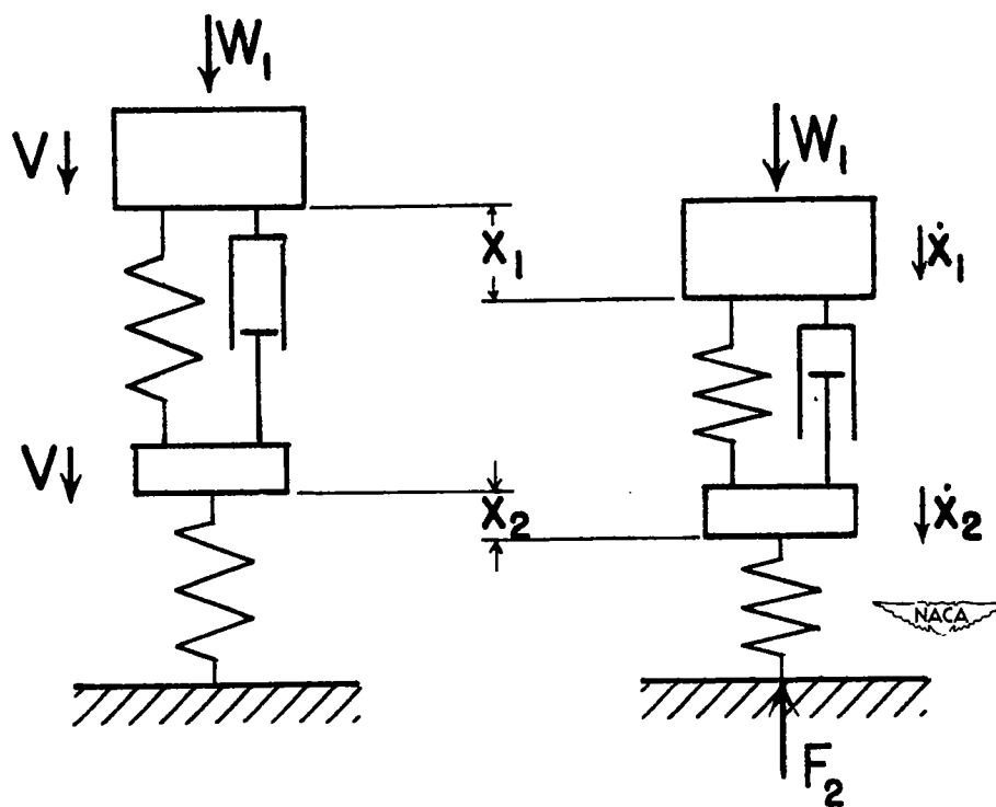
Figure 1.- Representation of shock strut by spring and damper arranged in parallel.
