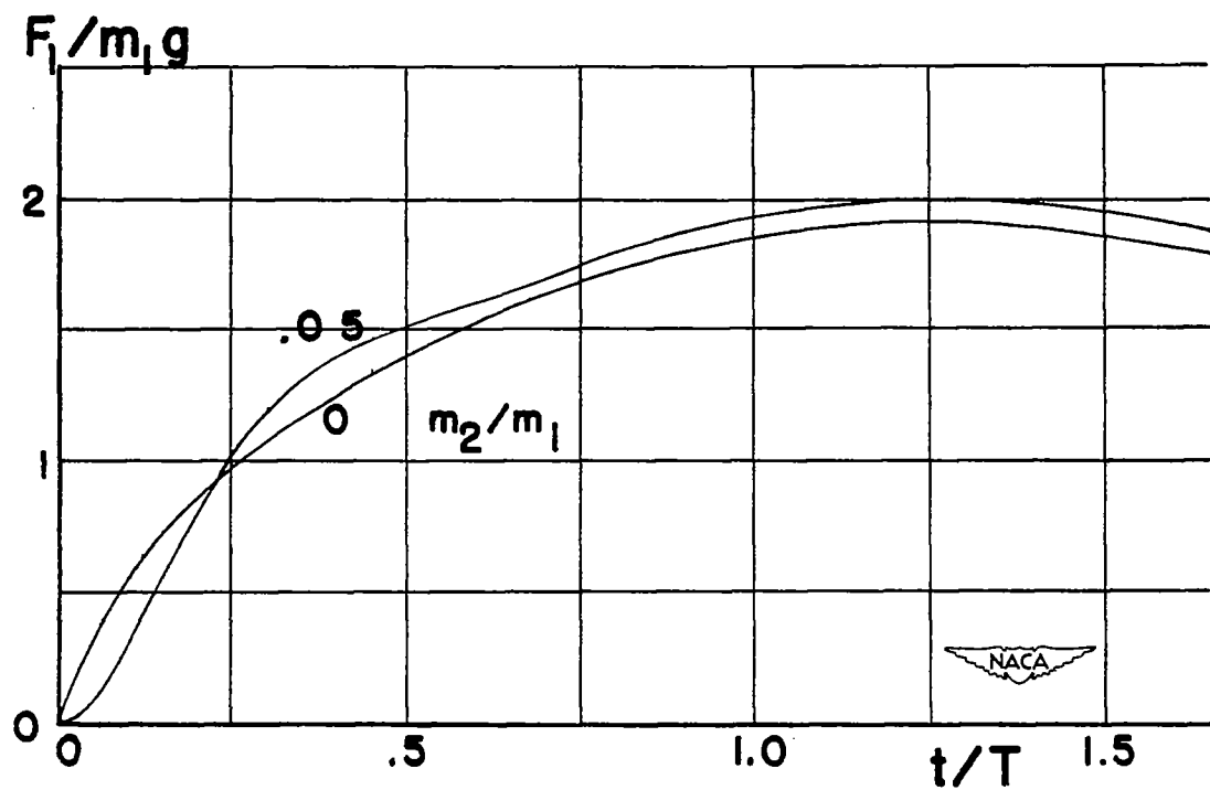
(a) On shock-strut force.
