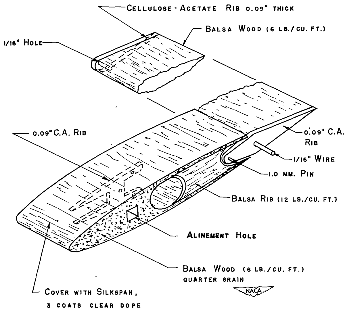
Figure 7.- Wing-section detail.
