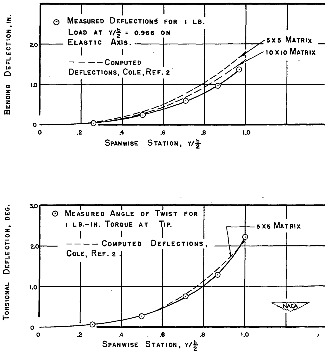
Figure 11.- Static deflections of straight wing.
