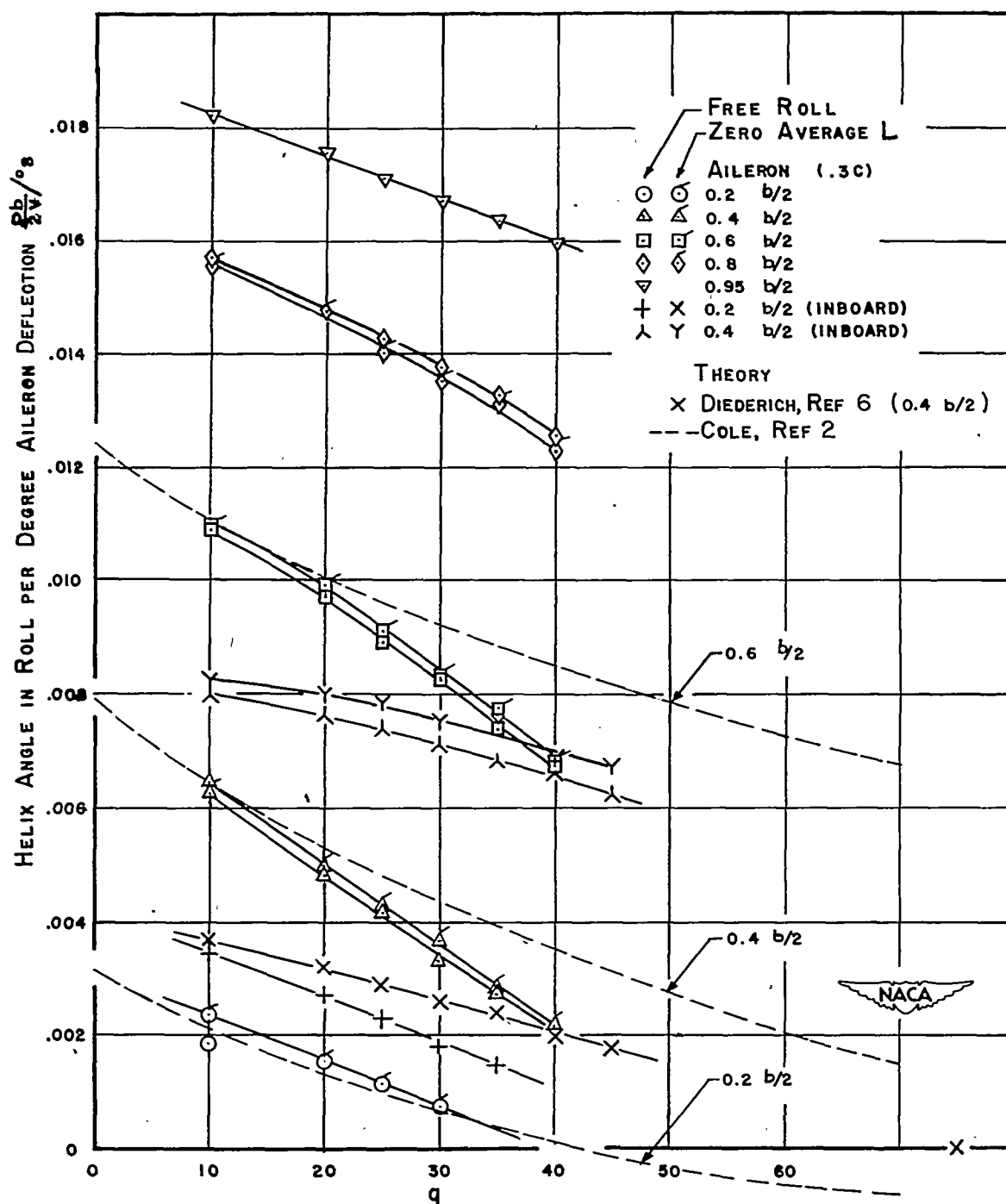
Figure 25.- Variation of helix angle in roll due to aileron deflection with q . Swept wing.
