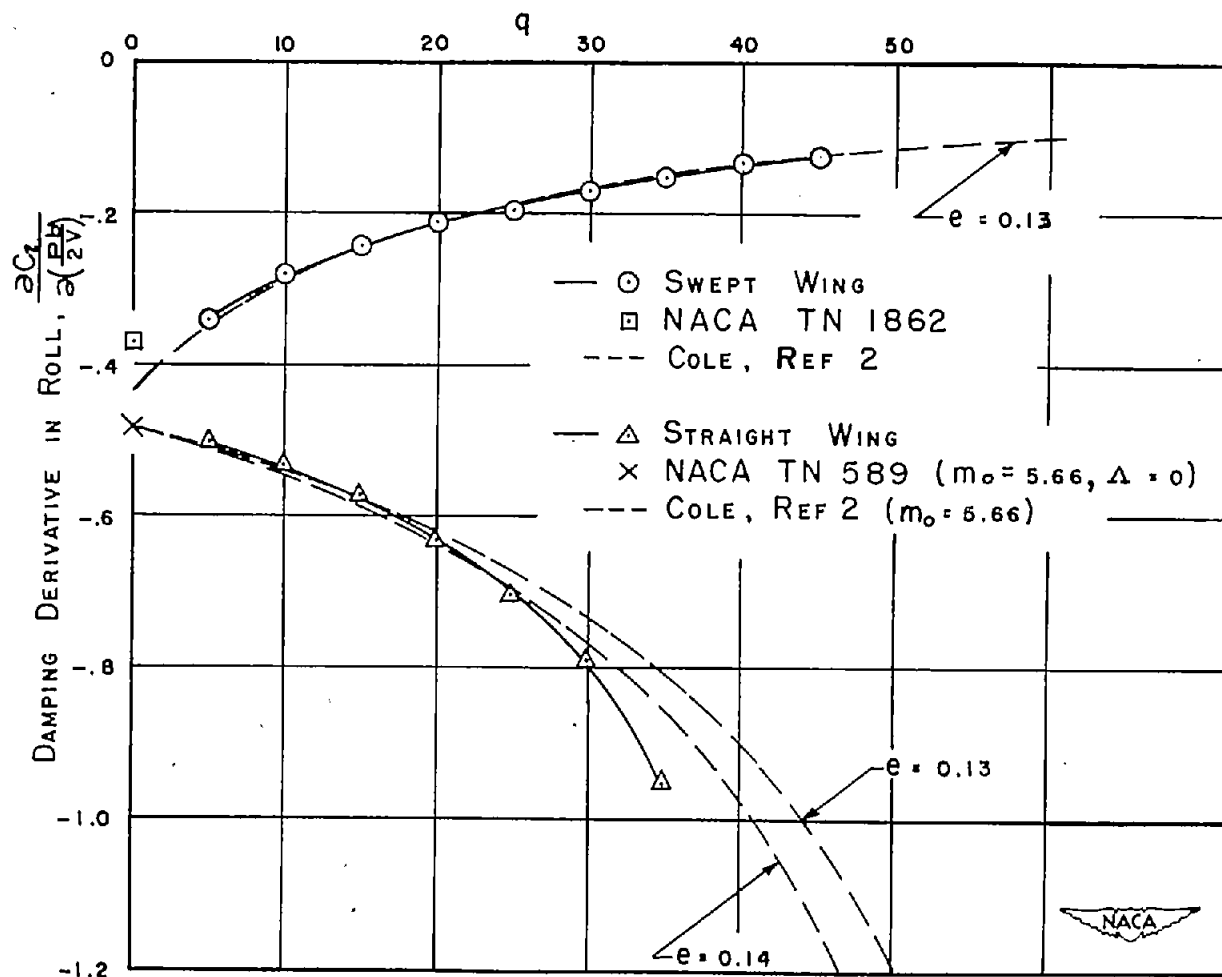
Figure 22.- Variation of damping derivative in roll with q . Straight and swept wings.
