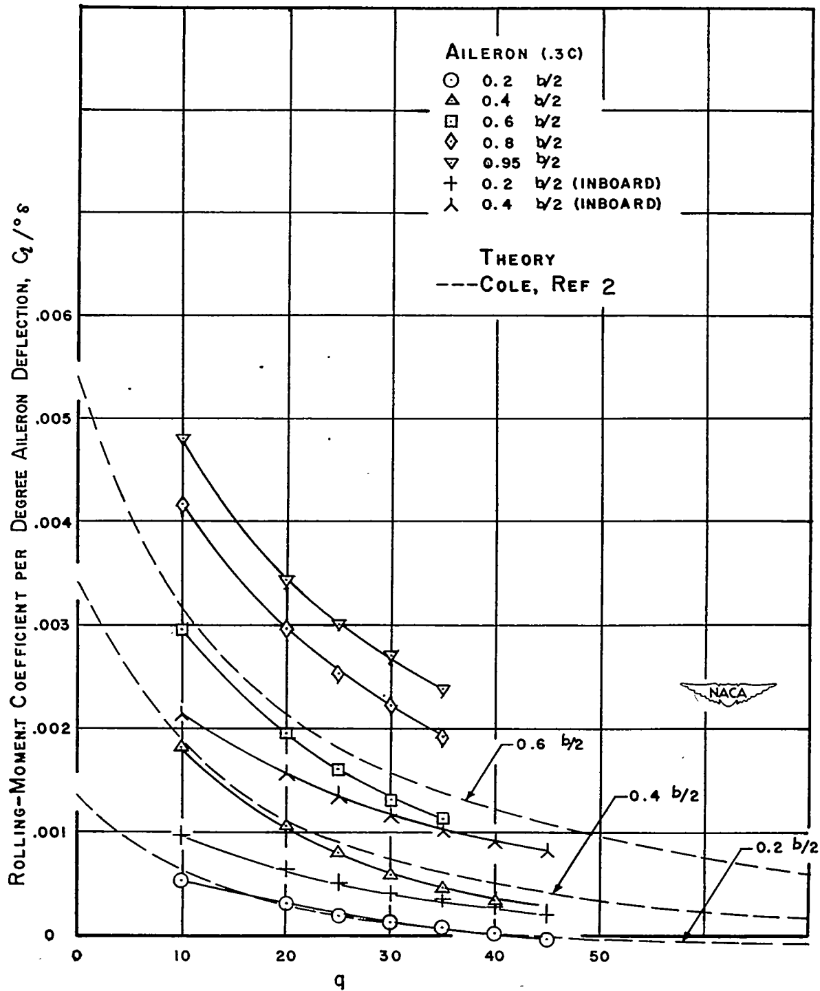
Figure 19.- Variation of rolling-moment coefficient due to aileron deflection with q . Swept wing.
