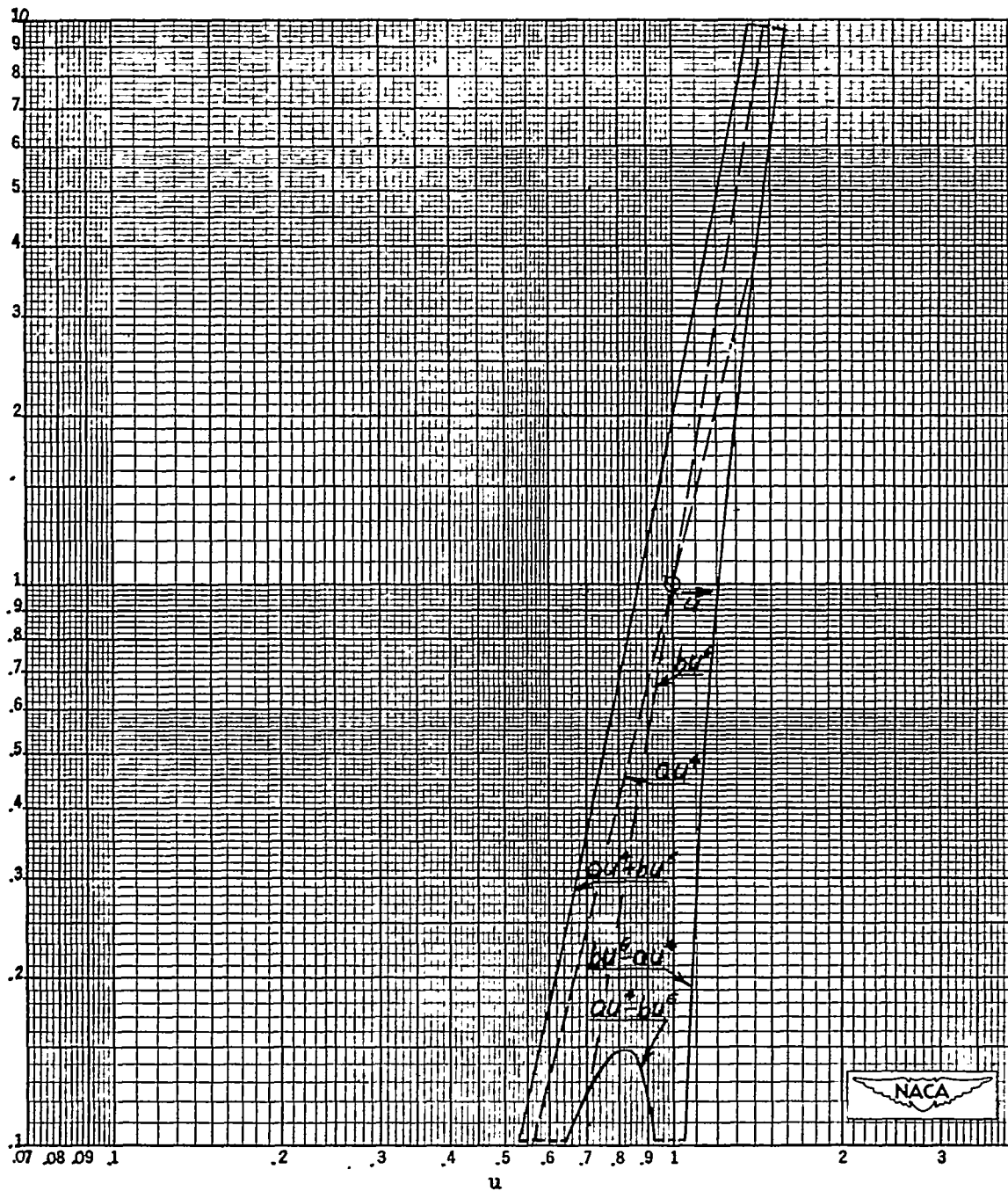
(c) Contours of term-pair templets representing logarithmic plots of \pm au^4 \pm bu^6 , shown oriented for a = b = 1 .
