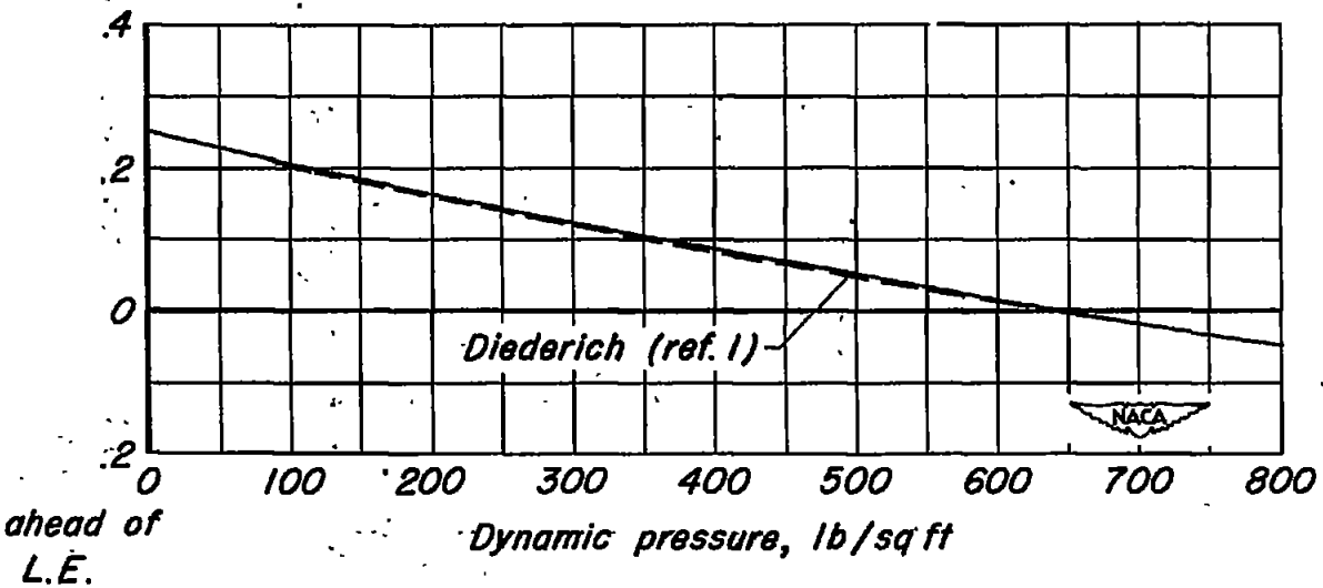
Figure 7.- Variation in spanwise and chordwise positions of aerodynamic center with dynamic pressure for example wing.
