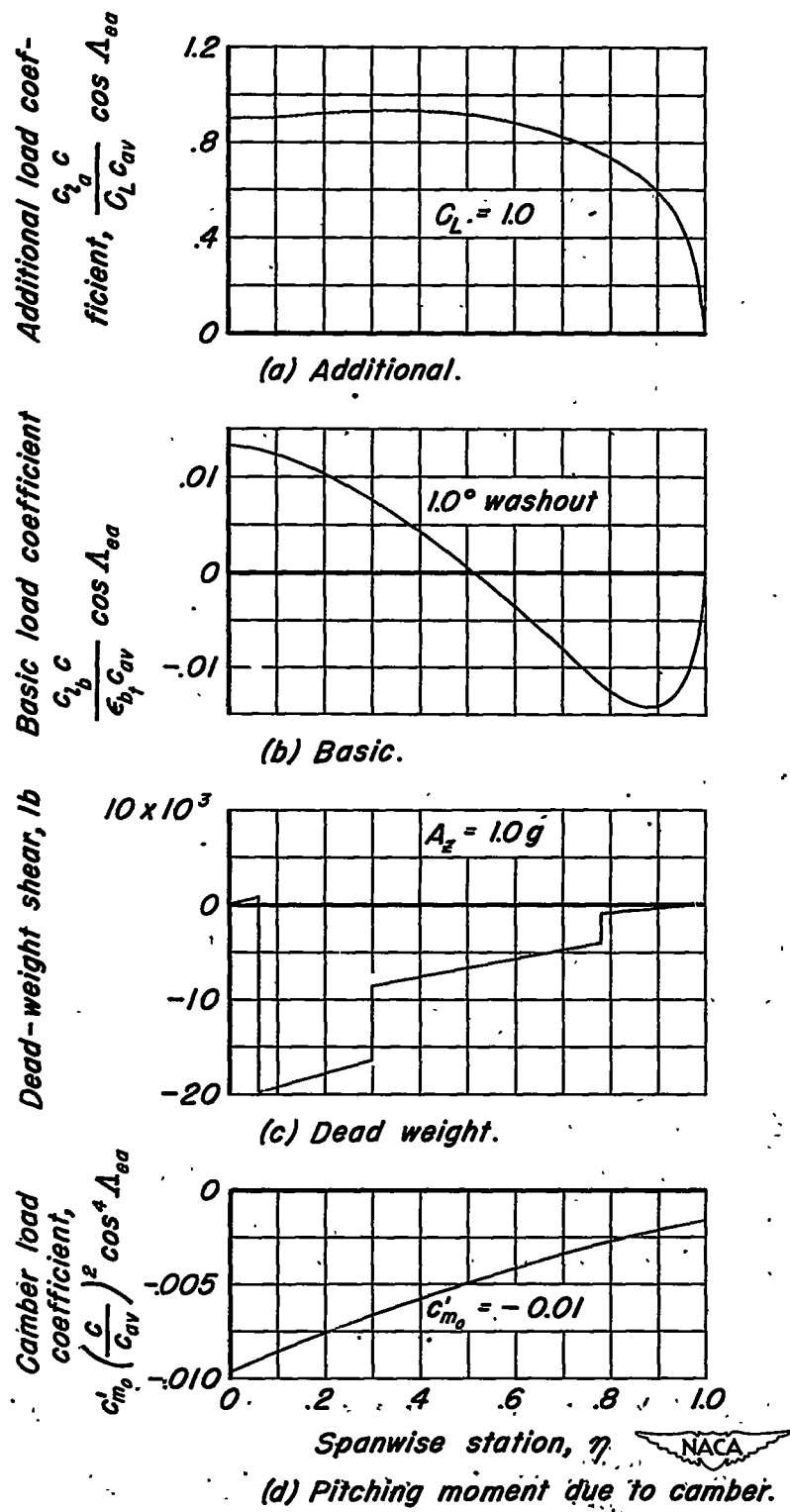
Figure 3.- Rigid-wing loadings for the example wing.
