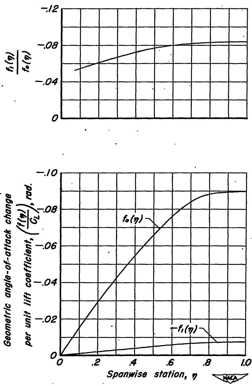
Figure 4.- The twist distributions f_0(\eta) and f_1(\eta) and the ratio \frac{f_1(\eta)}{f_0(\eta)} for the example wing as calculated for the additional loading.
