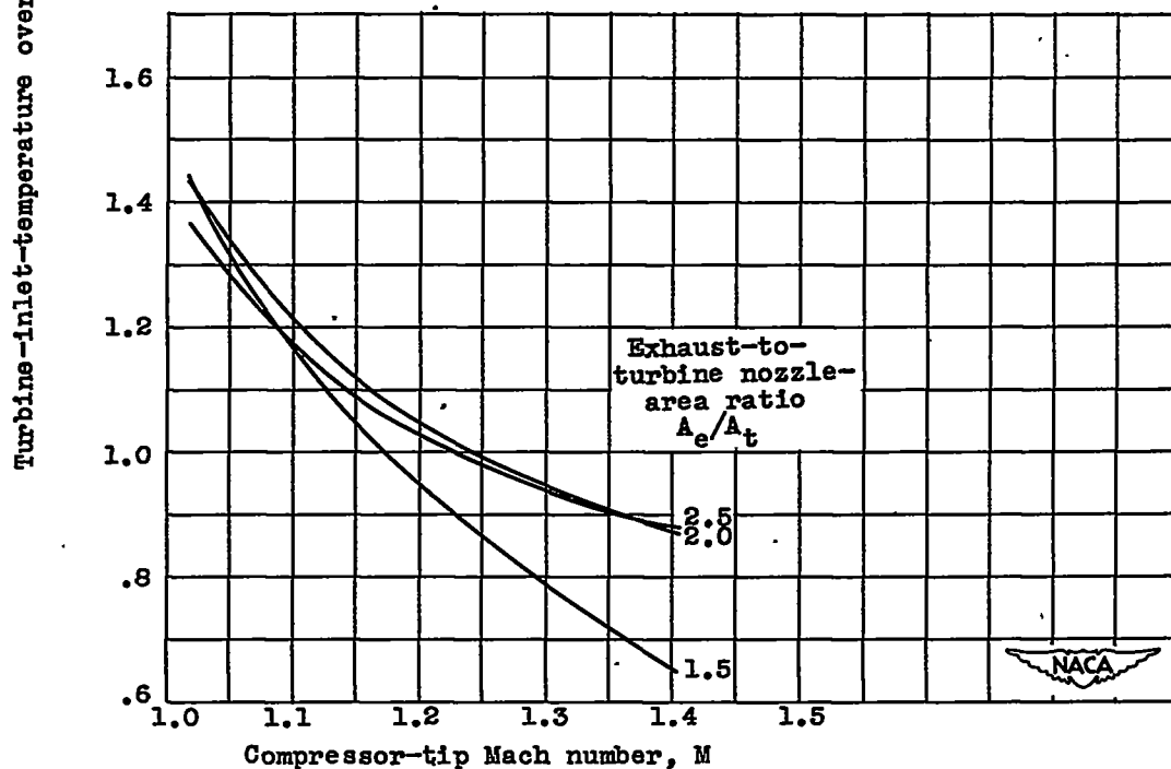
(c) Variation of exhaust-to-turbine nozzle-area ratio.
