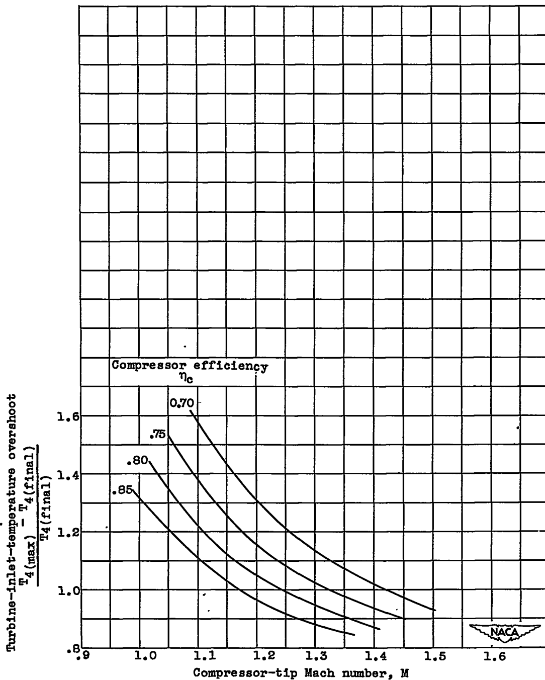
(a) Variation of compressor efficiency.
