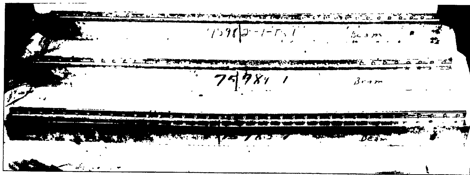
Figure 7.- Typical failures of spot-welded static beam specimens.
