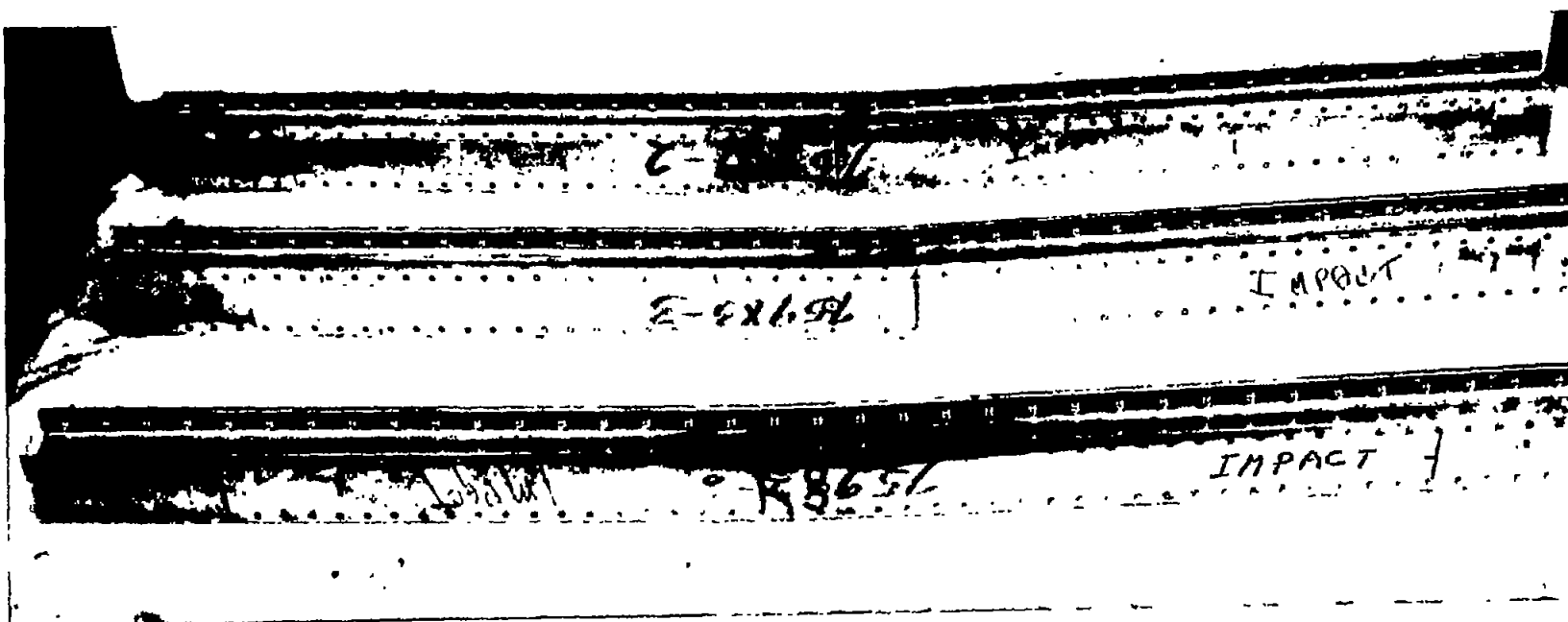
Figure 11.- Typical failures of riveted impact beam specimens.
