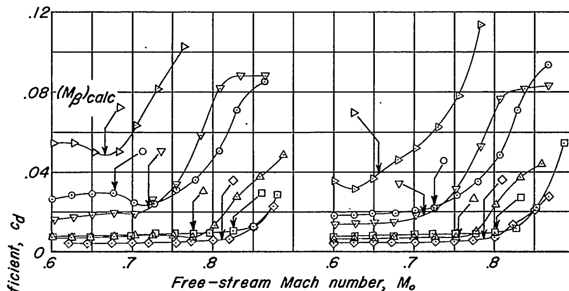
(i) NACA 66,-206.
