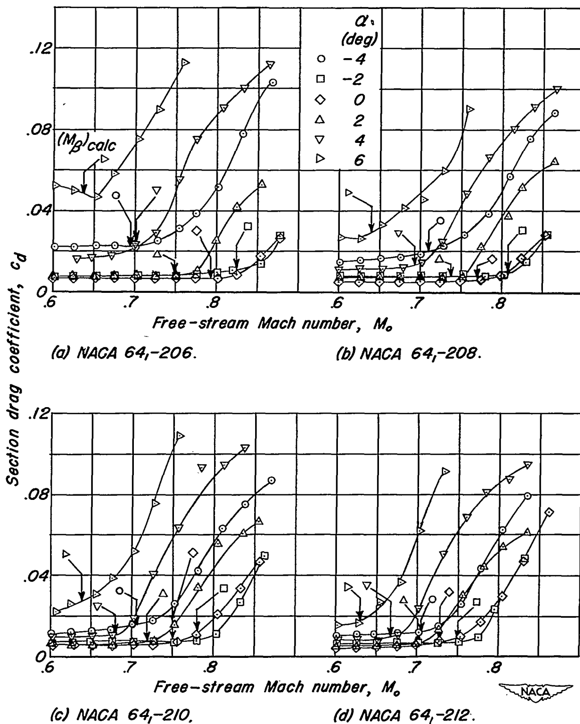
Figure 7.- Calculated Mach number for occurrence of sonic velocity at airfoil crest and variation of section drag coefficient with Mach number for a variety of airfoil sections.
