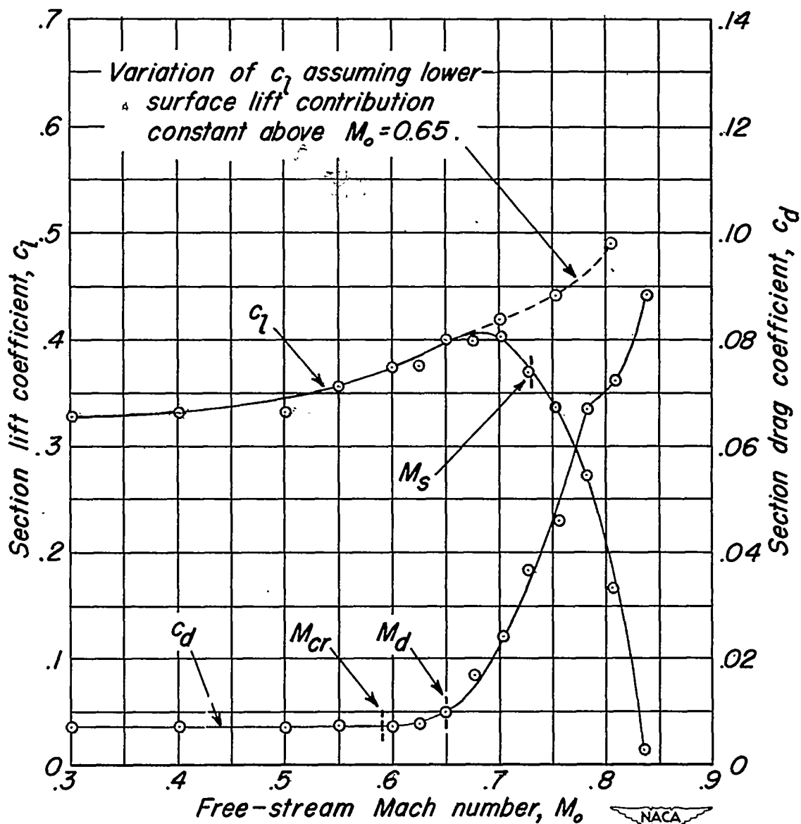
Figure 1.— Section lift and drag coefficients as functions of free-stream Mach number for NACA 23015 airfoil section at 2^\circ angle of attack.
