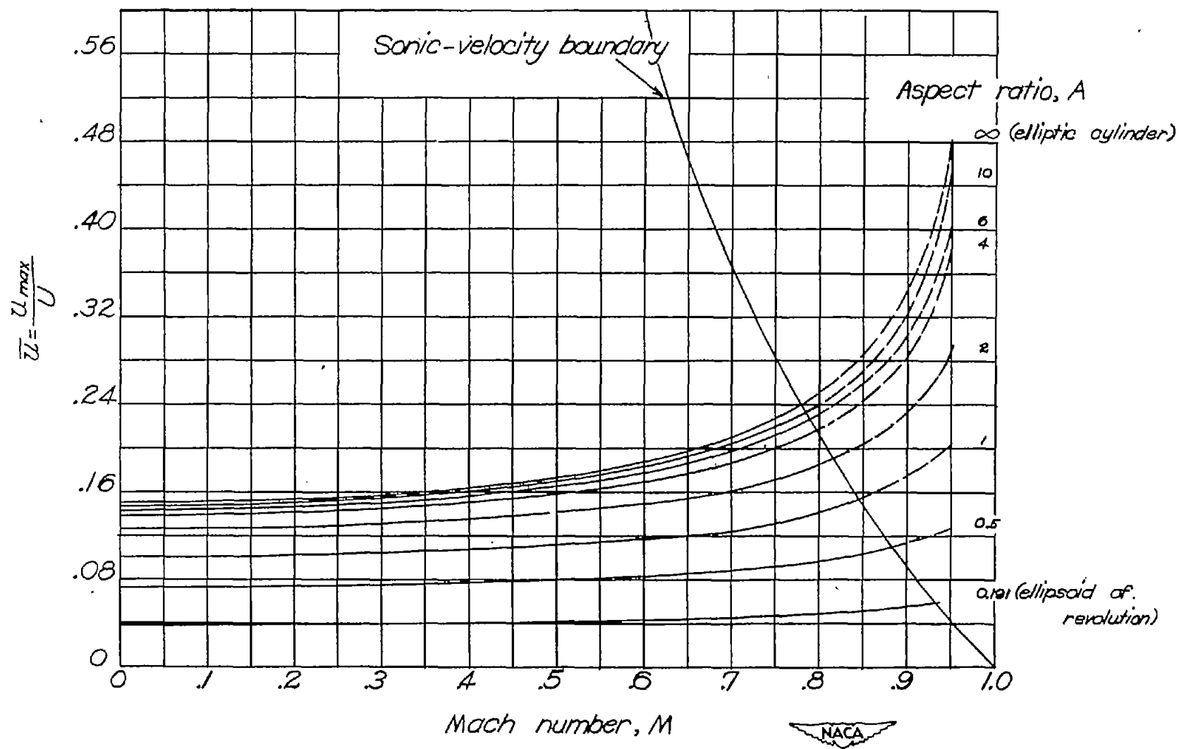
Figure 2.- Variation with Mach number of maximum incremental velocity for ellipsoids having various aspect ratios. Thickness ratio, 0.15.
