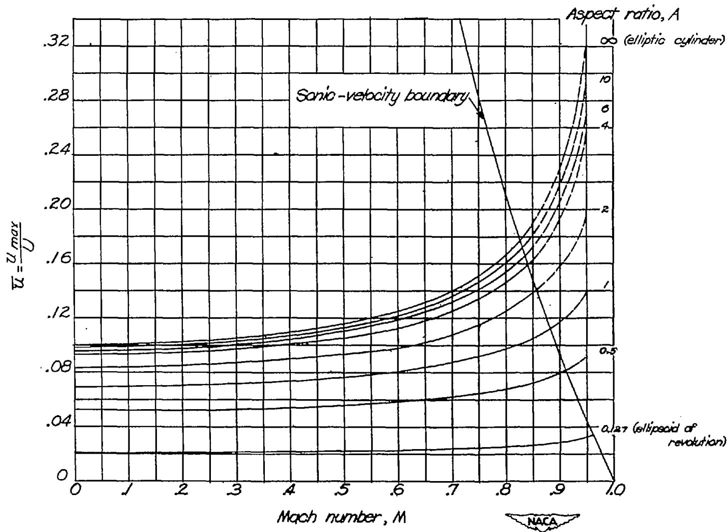
Figure 1.- Variation with Mach number of maximum incremental velocity for ellipsoids having various aspect ratios. Thickness ratio, 0.10.
