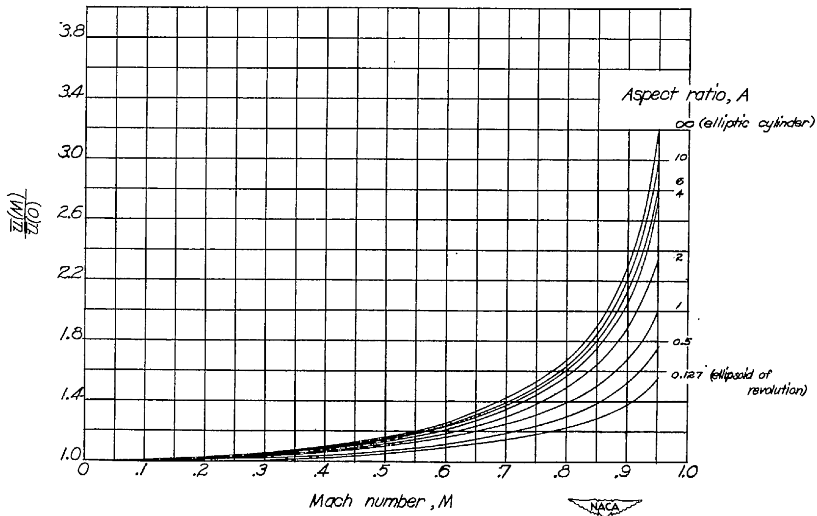
Figure 4.— Variation of compressibility effect with Mach number for ellipsoids having various aspect ratios. Thickness ratio, 0.10.
