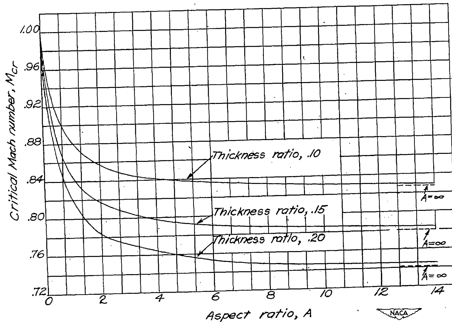
Figure 7.- Variation of critical Mach number with aspect ratio for ellipsoids having thickness ratios of 0.10, 0.15 and 0.20.
