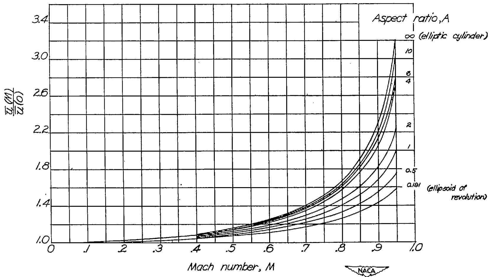
Figure 5.- Variation of compressibility effect with Mach number for ellipsoids having various aspect ratios, Thickness ratio, 0.15.
