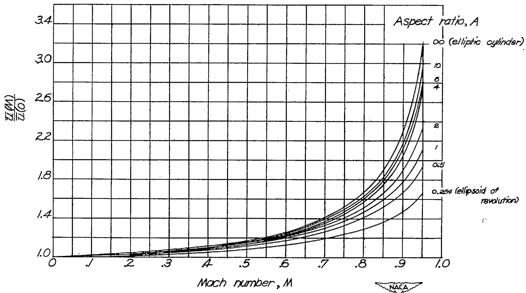
Figure 6.- Variation of compressibility effect with Mach number for ellipsoids having various aspect ratios. Thickness ratio, 0.20.
