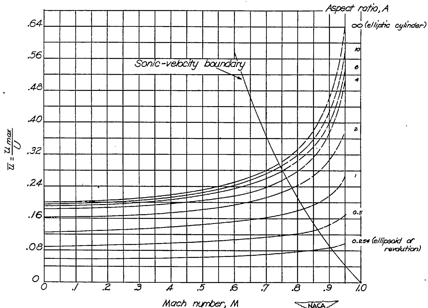
Figure 3.- Variation with Mach number of maximum incremental velocity for ellipsoids having various aspect ratios. Thickness ratio, 0.20.
