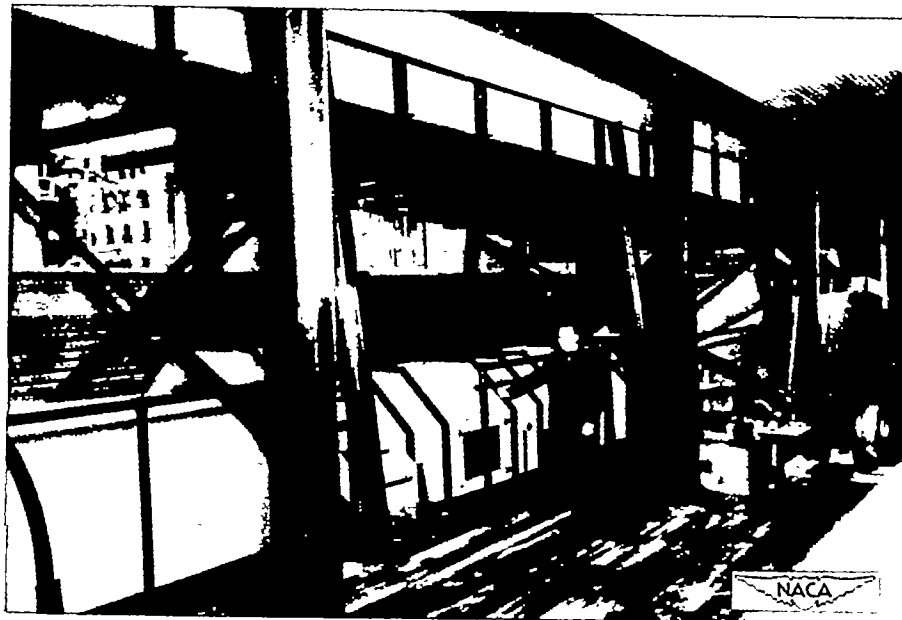
Figure 4.- The 4\frac{1}{2} -foot wind tunnel of the National Bureau of Standards.
