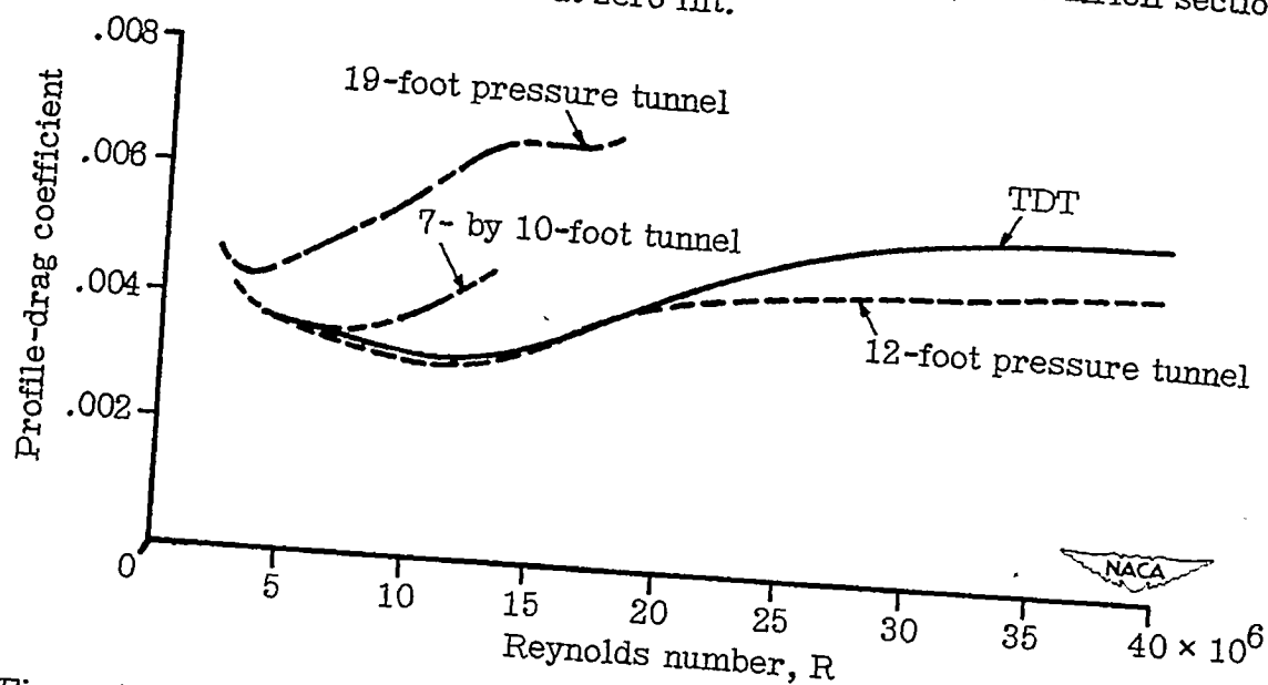
Figure 2.- Comparative drag measurements of NACA 66,1-015 airfoil in four NACA low-speed wind tunnels.
