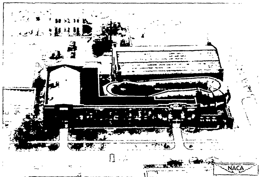
Figure 6.- The Langley two-dimensional low-turbulence pressure tunnel.
