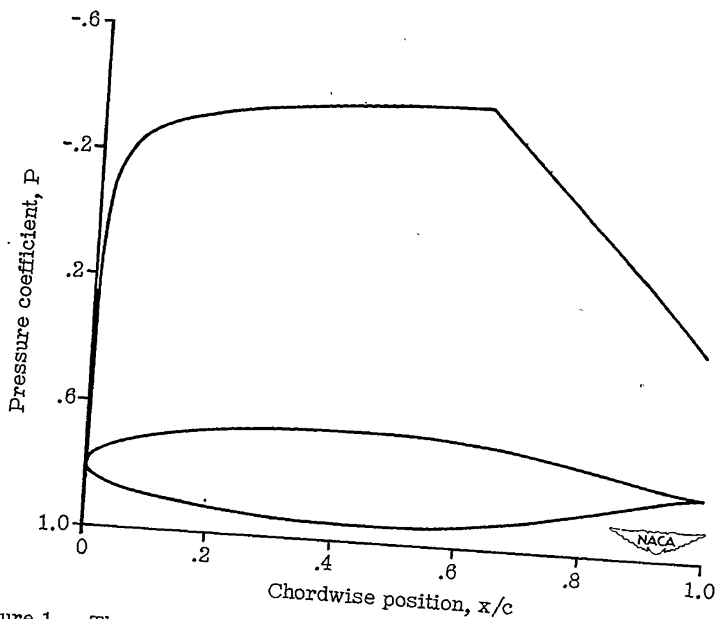
Figure 1.- Theoretical pressure distribution for NACA 66,1-015 airfoil section at zero lift.
