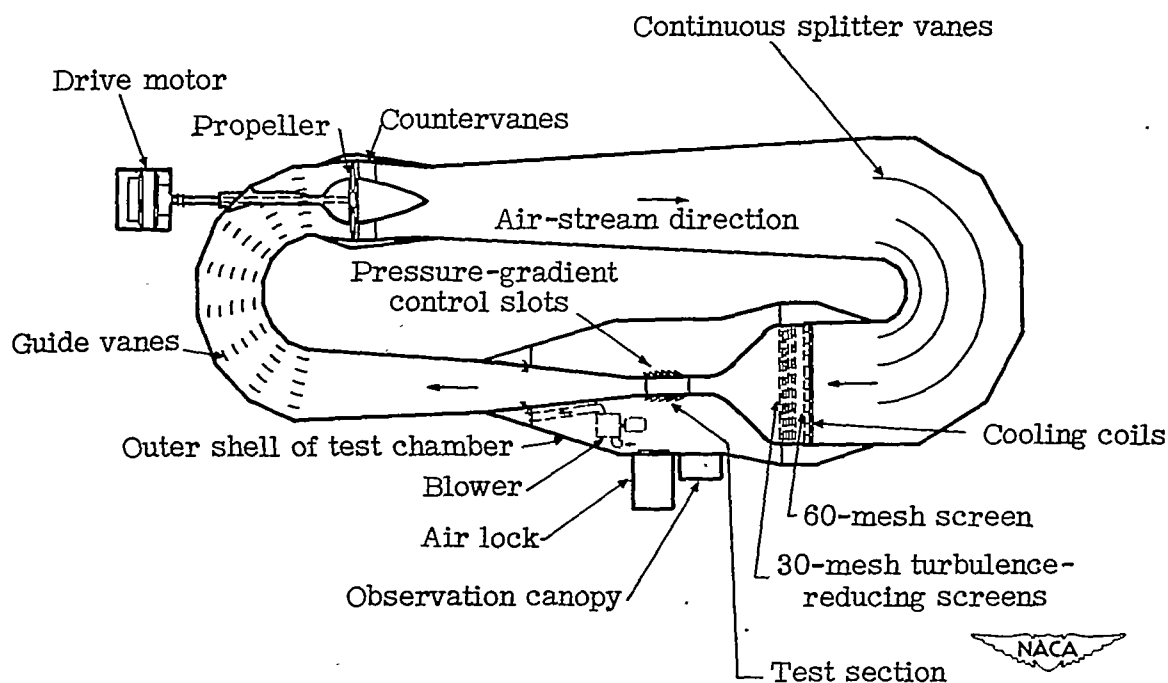
Figure 7.- The Langley two-dimensional low-turbulence pressure tunnel.
