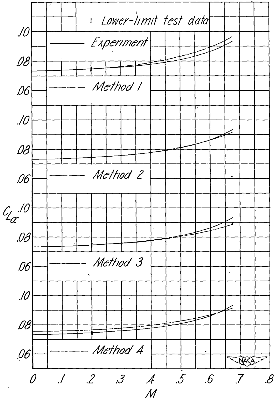
Figure 8.- Variation of lift-curve slope with Mach number. \Lambda = 3.2^\circ . Model 7.
