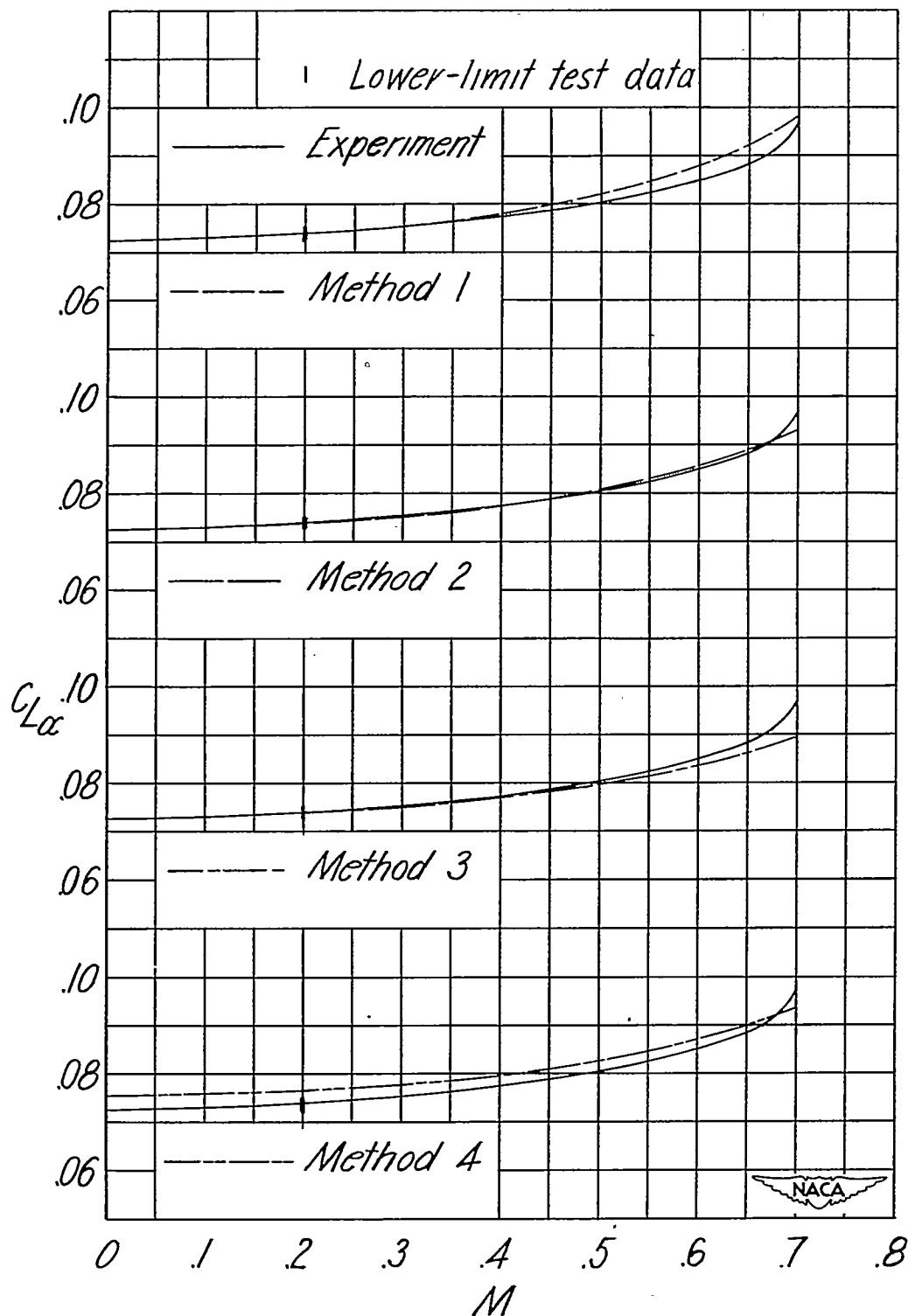
Figure 9.- Variation of lift-curve slope with Mach number. \Lambda = 3.2^\circ . Model 8.
