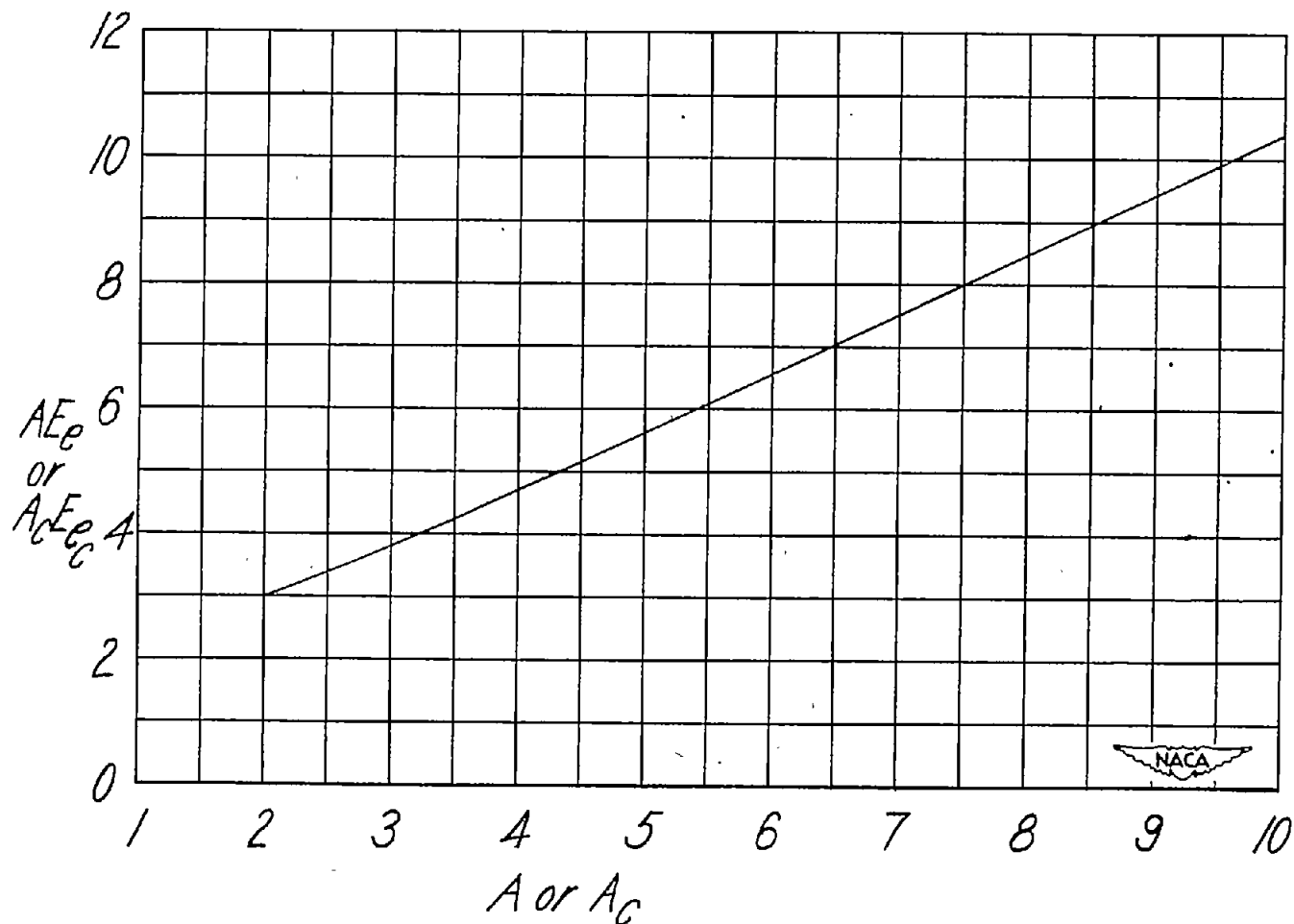
Figure 4.- Quantity useful for evaluation of the lift-curve slope by lifting-surface theory (reference 6).
