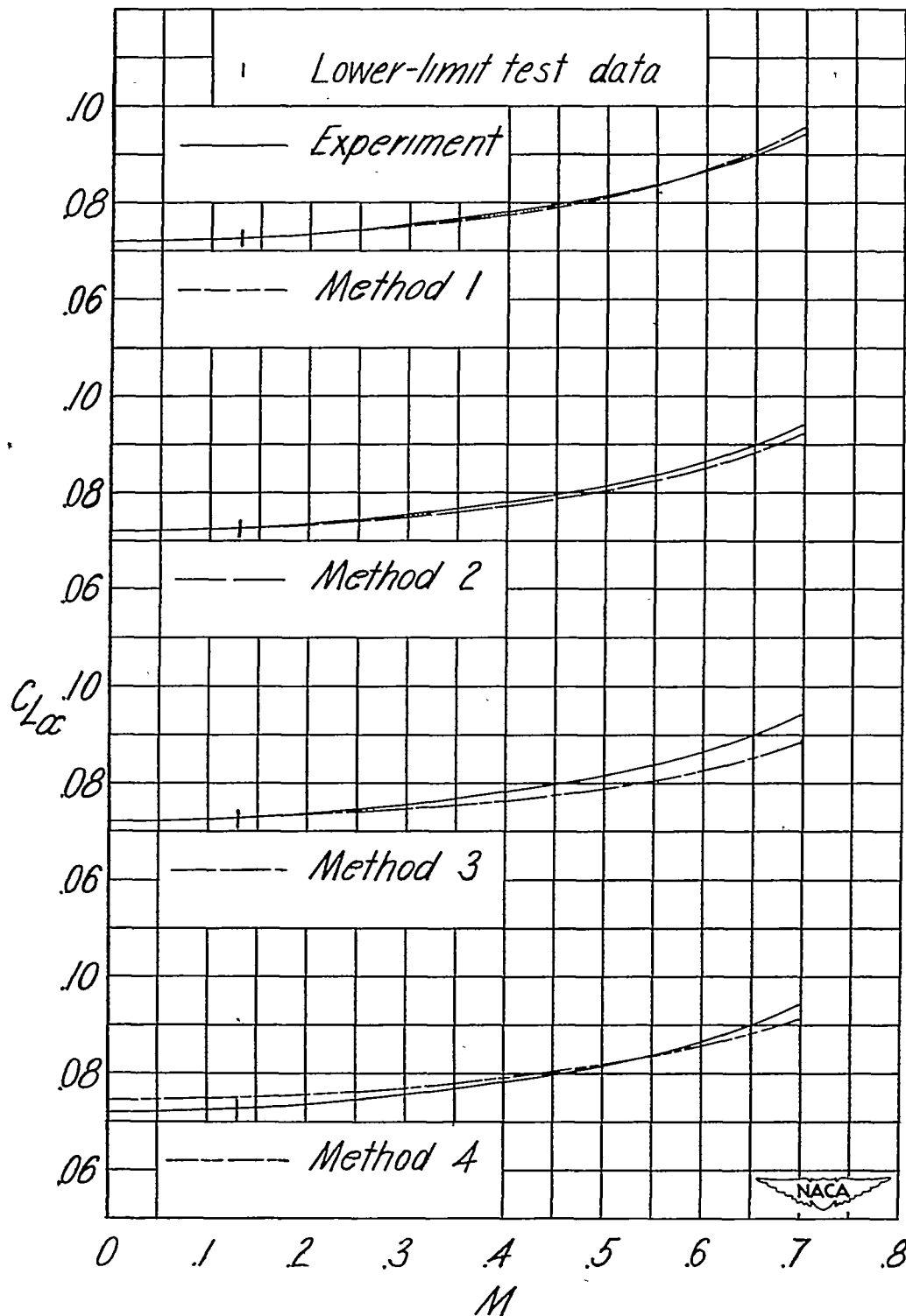
Figure 5.- Variation of lift-curve slope with Mach number. \Lambda = 0^\circ . Model 4.
