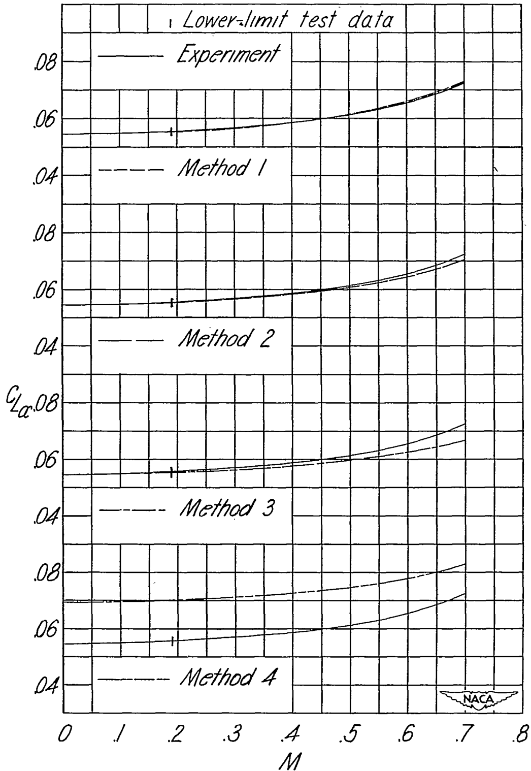
Figure 6.- Variation of lift-curve slope with Mach number. \Lambda = 8^\circ . Model 5.
