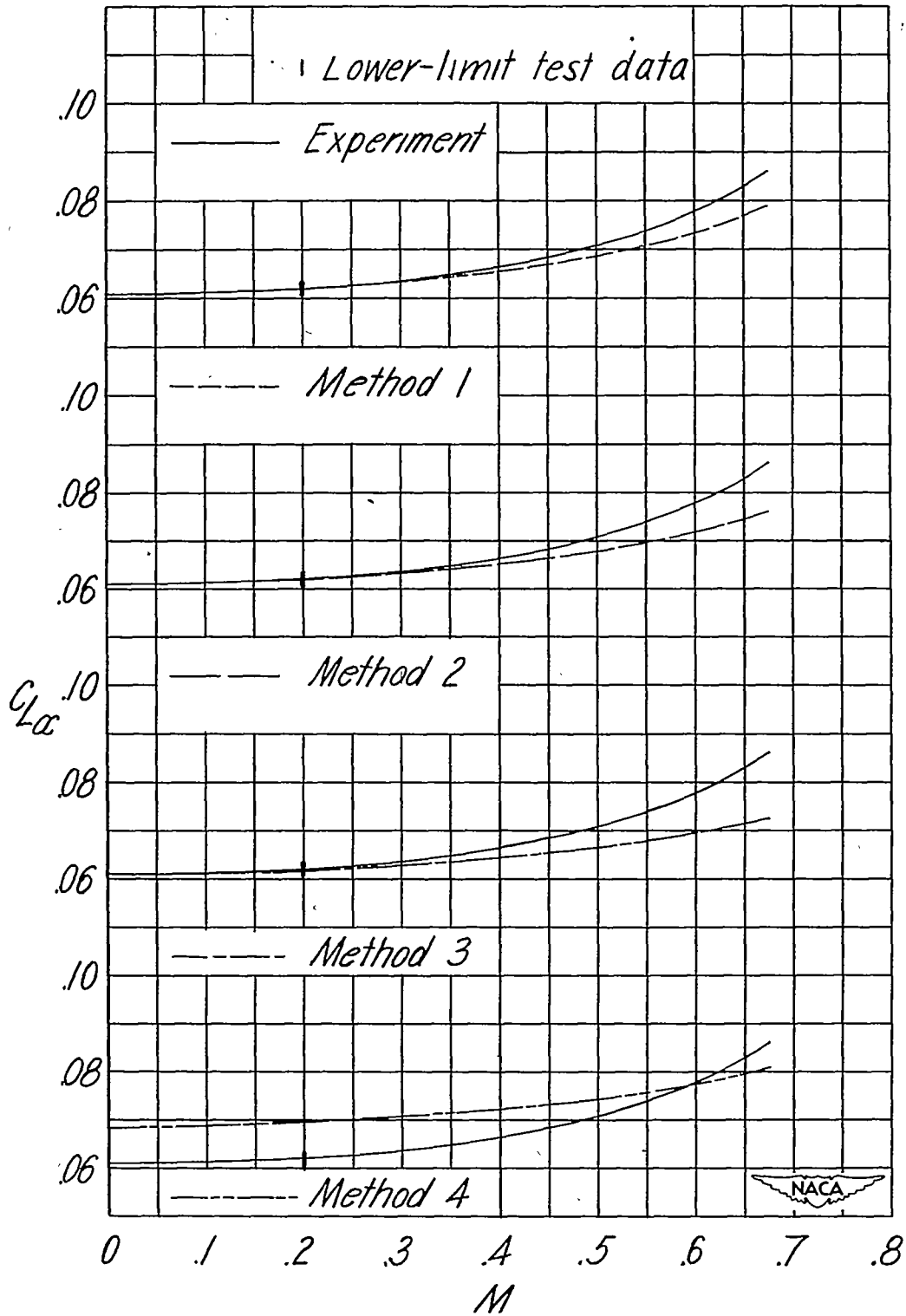
Figure 10.- Variation of lift-curve slope with Mach number. \Lambda = 6.3^\circ . Model 9.
