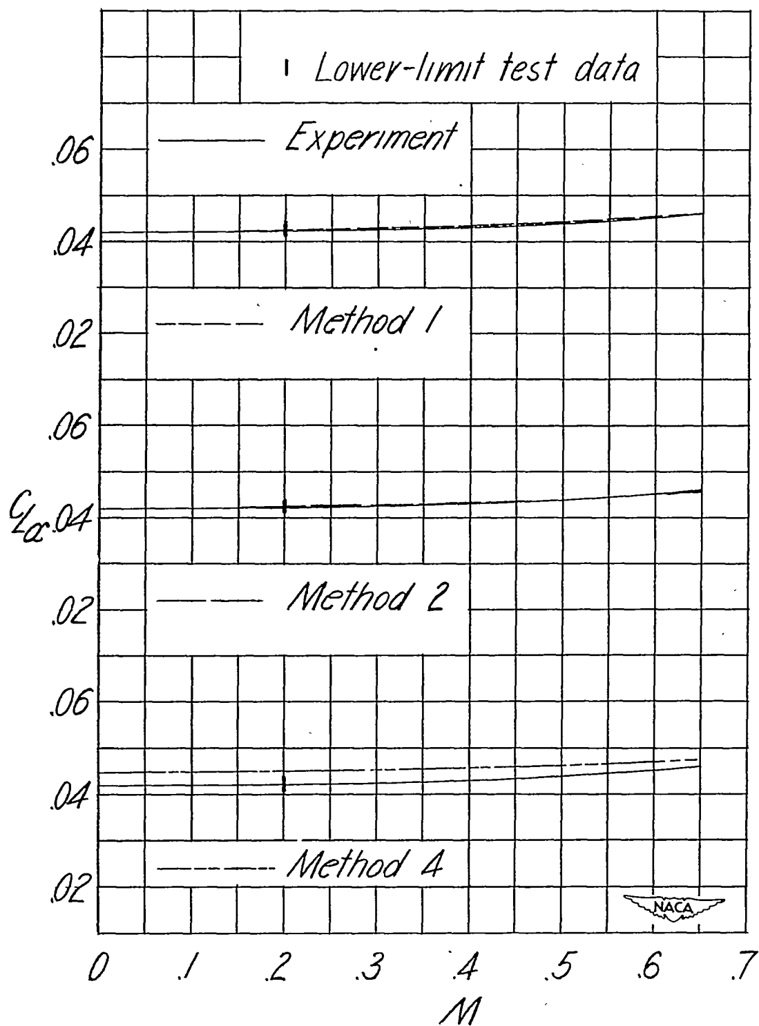
Figure 15.- Variation of lift-curve slope with Mach number. \Lambda = -45.0^\circ . Model 1A.
