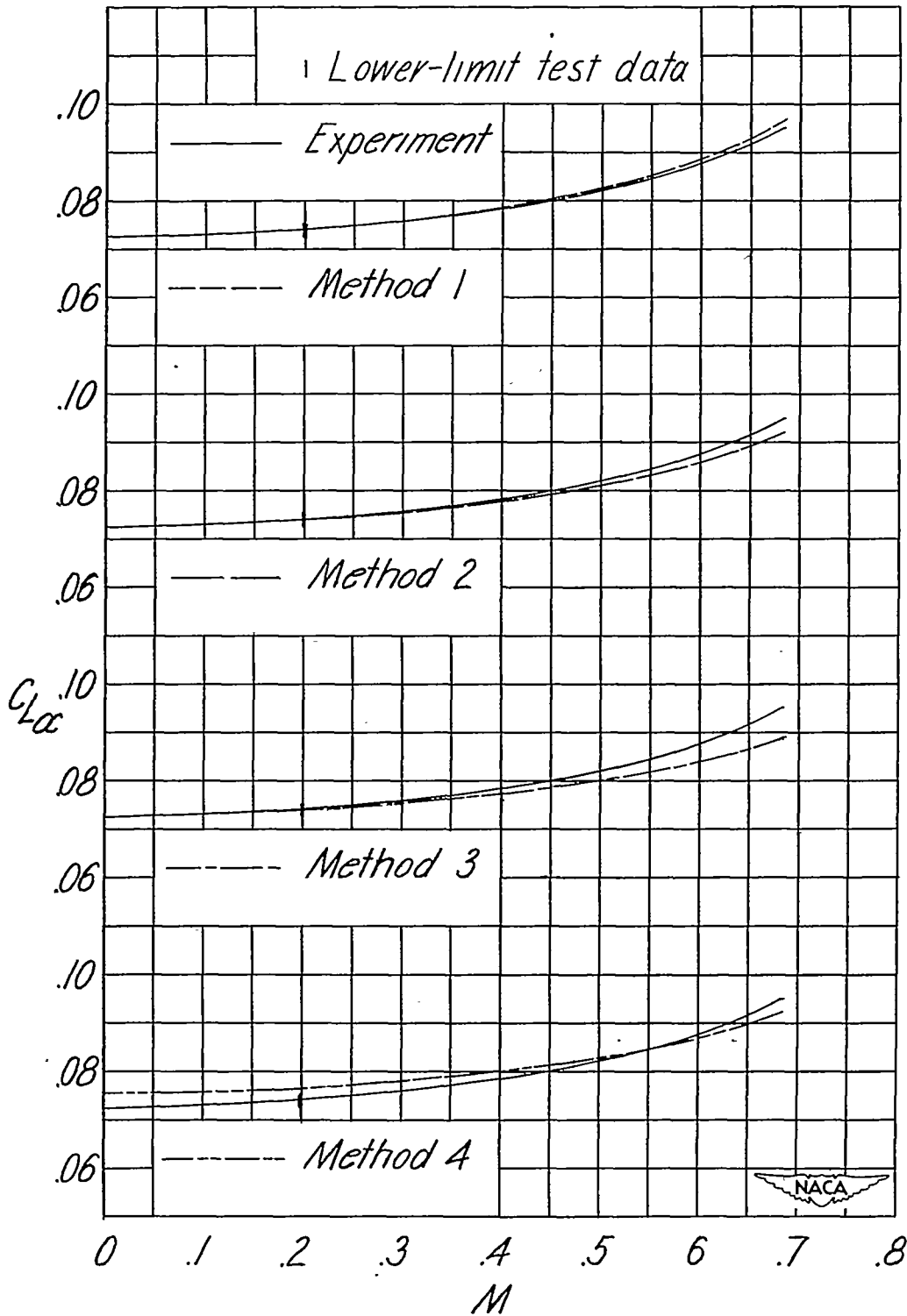
Figure 7.- Variation of lift-curve slope with Mach number. \Lambda = 0^\circ . Model 6.
