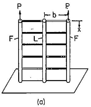
Figure 1.- Single-stringer panel.
