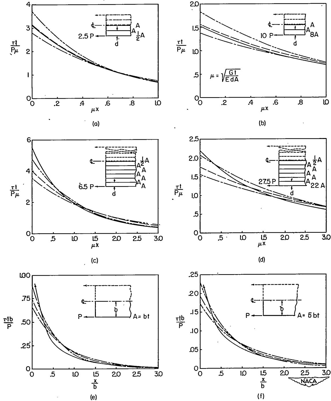
Figure 5.- Comparisons between solutions obtained by rigorous methods (on assumption of infinite transverse stiffness) and substitute-single-stringer method.
