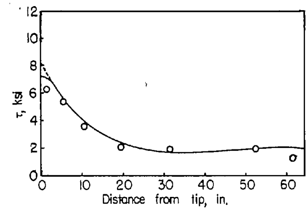
(b) Shear stresses in panel E. P = 7.5 kips.
