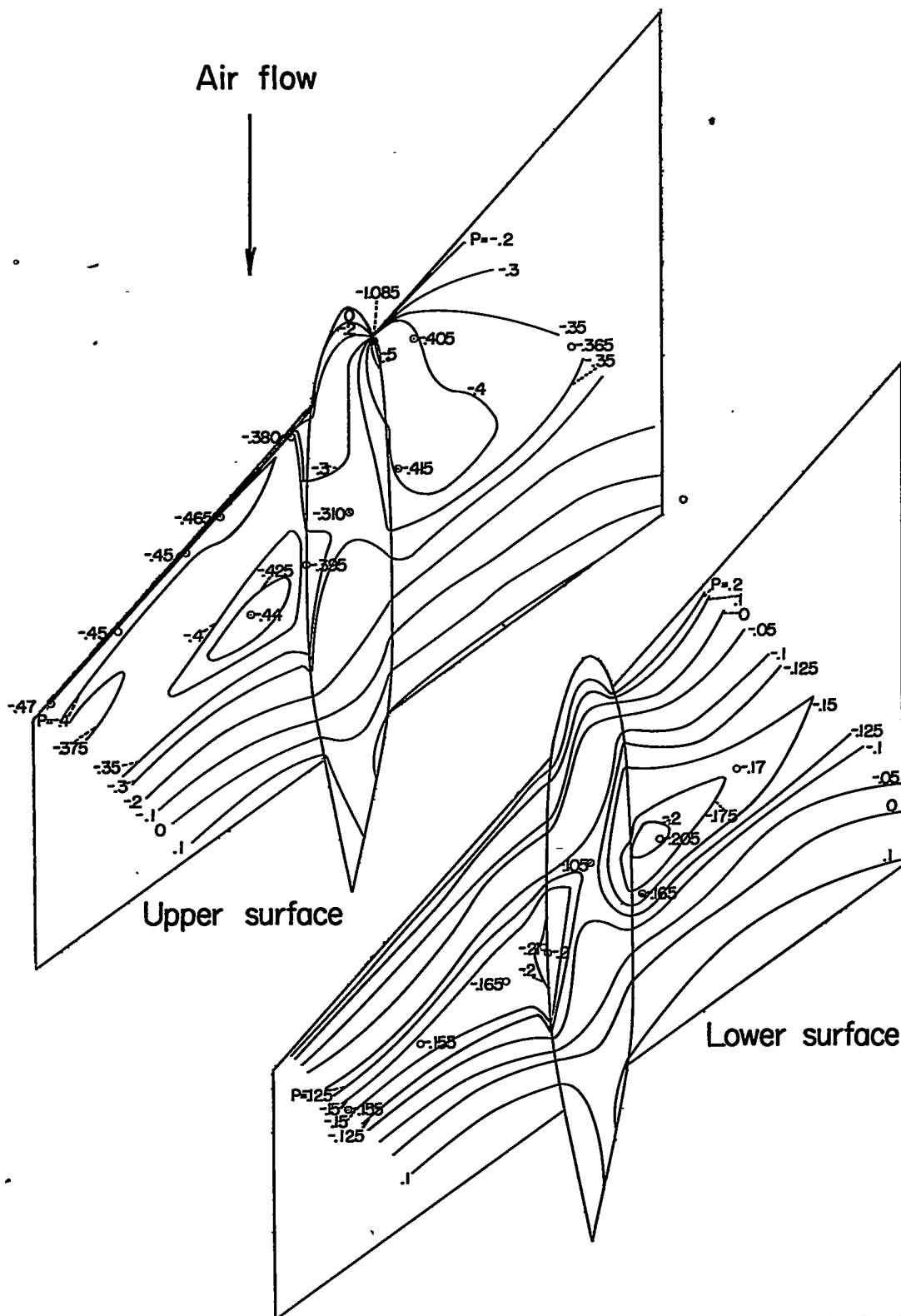
Figure 47.—Pressure contours for the wing-nacelle combination.
