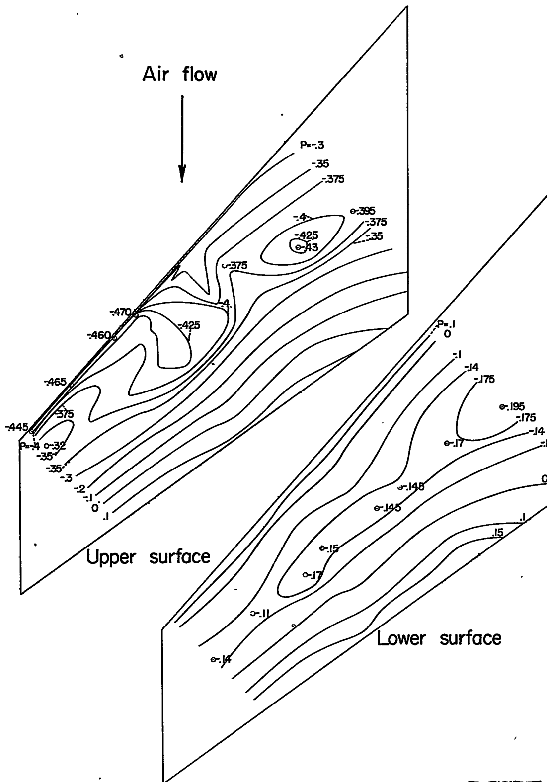
Figure 37.—Pressure contours for the wing alone. \Lambda = 45^\circ ; C_L = 0.20 ; M = 0.20 .
