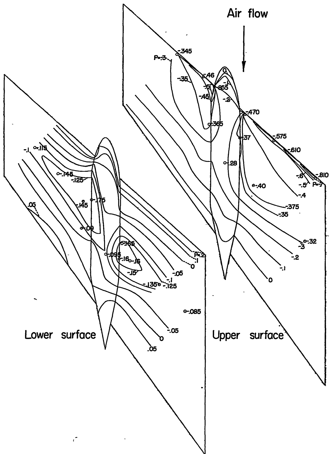
Figure 48.—Pressure contours for the wing-nacelle combination. \Lambda = -45^\circ ; C_L = 0.20 ; M = 0.20 .
