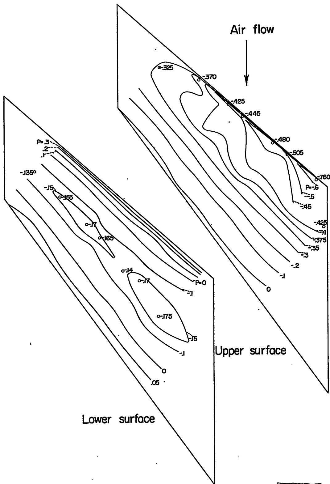
Figure 33.—Pressure contours for the wing alone. \Lambda = -45^\circ ; C_L = 0.20 ; M = 0.61 .
