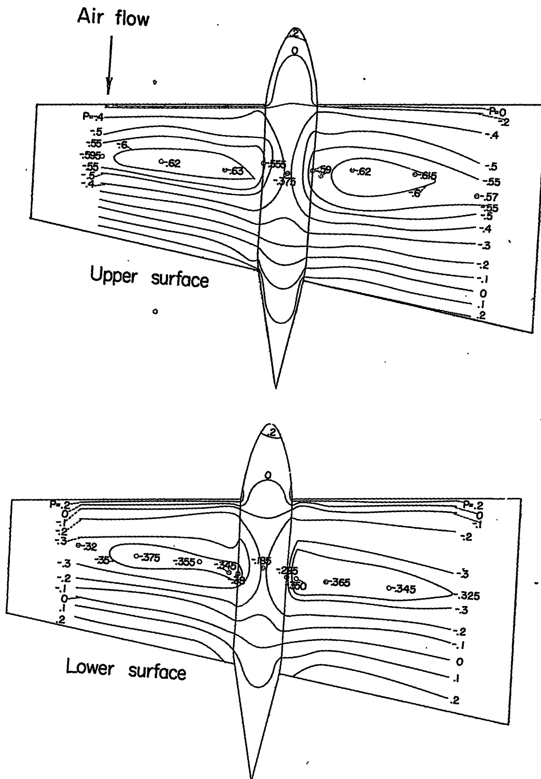
Figure 46.—Pressure contours for the wing-nacelle combination. \Lambda = 0^\circ ; C_L = 0.20 ; M = 0.20 .
