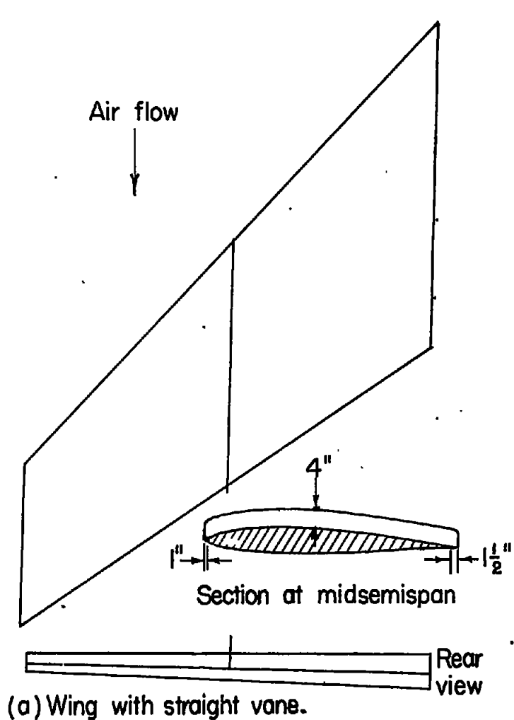
Figure 8.— Wing at 45° sweepback with straight and curved vanes mounted at midsemispan.
