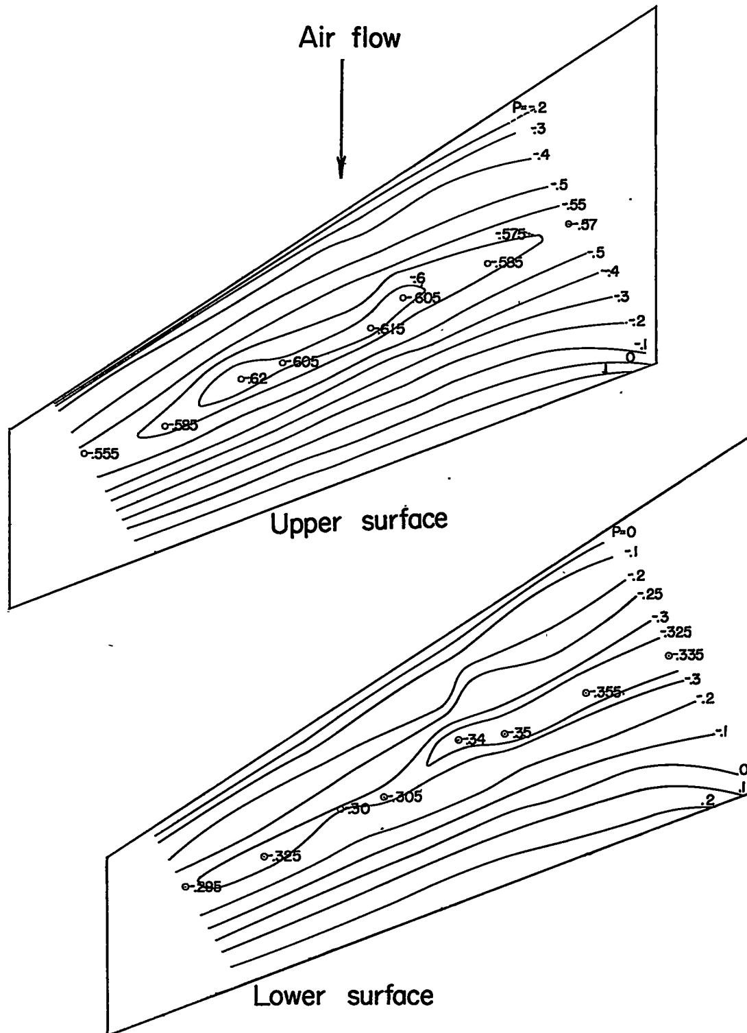
Figure 35.—Pressure contours for the wing alone. \Lambda = 30^\circ ; C_L = 0.20 ; M = 0.61 .
