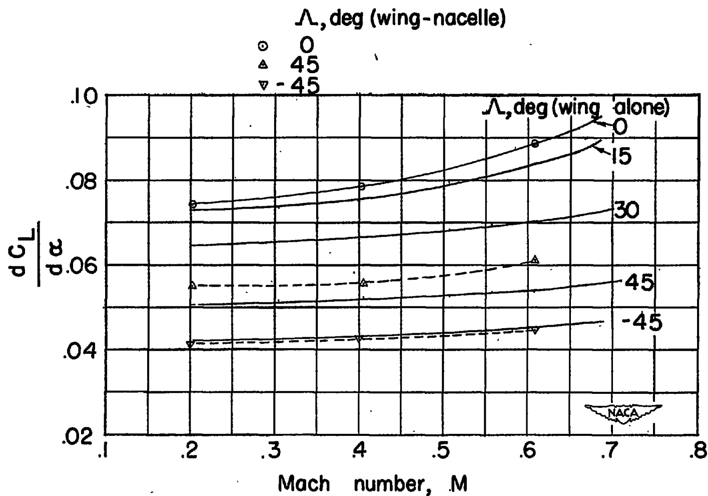
Figure 15.— Variation of lift - curve slope with Mach number for wing alone and wing-nacelle combination.
