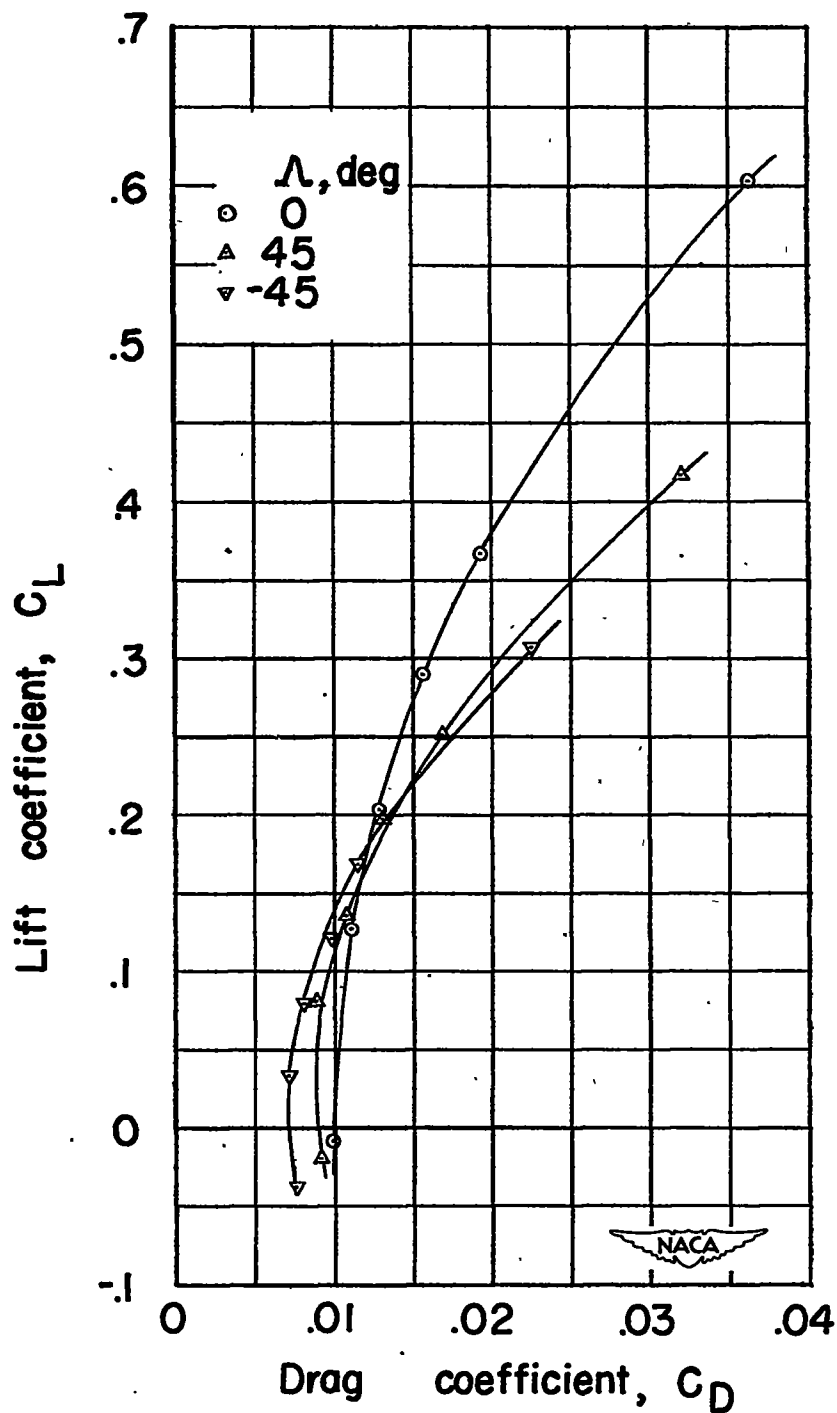
Figure 18. — Variation of drag coefficient with lift coefficient for wing-nacelle combination.
