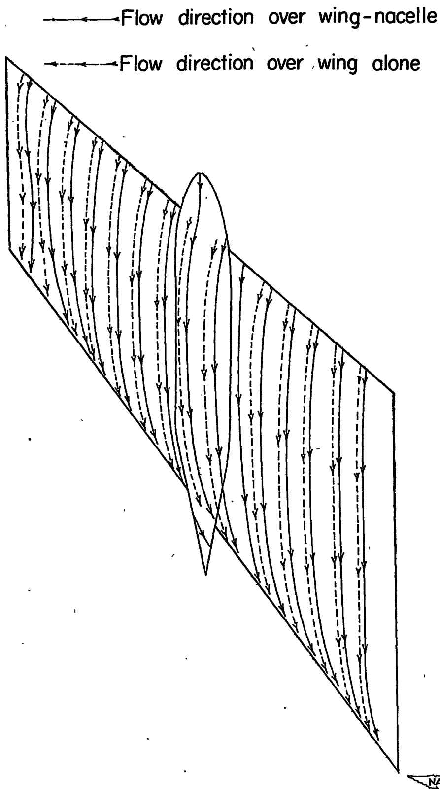
Figure 56.—Flow patterns over the wing and wing-nacelle combination. \Lambda = -45^\circ ; \alpha_g = 9^\circ ; M = 0.13 .
