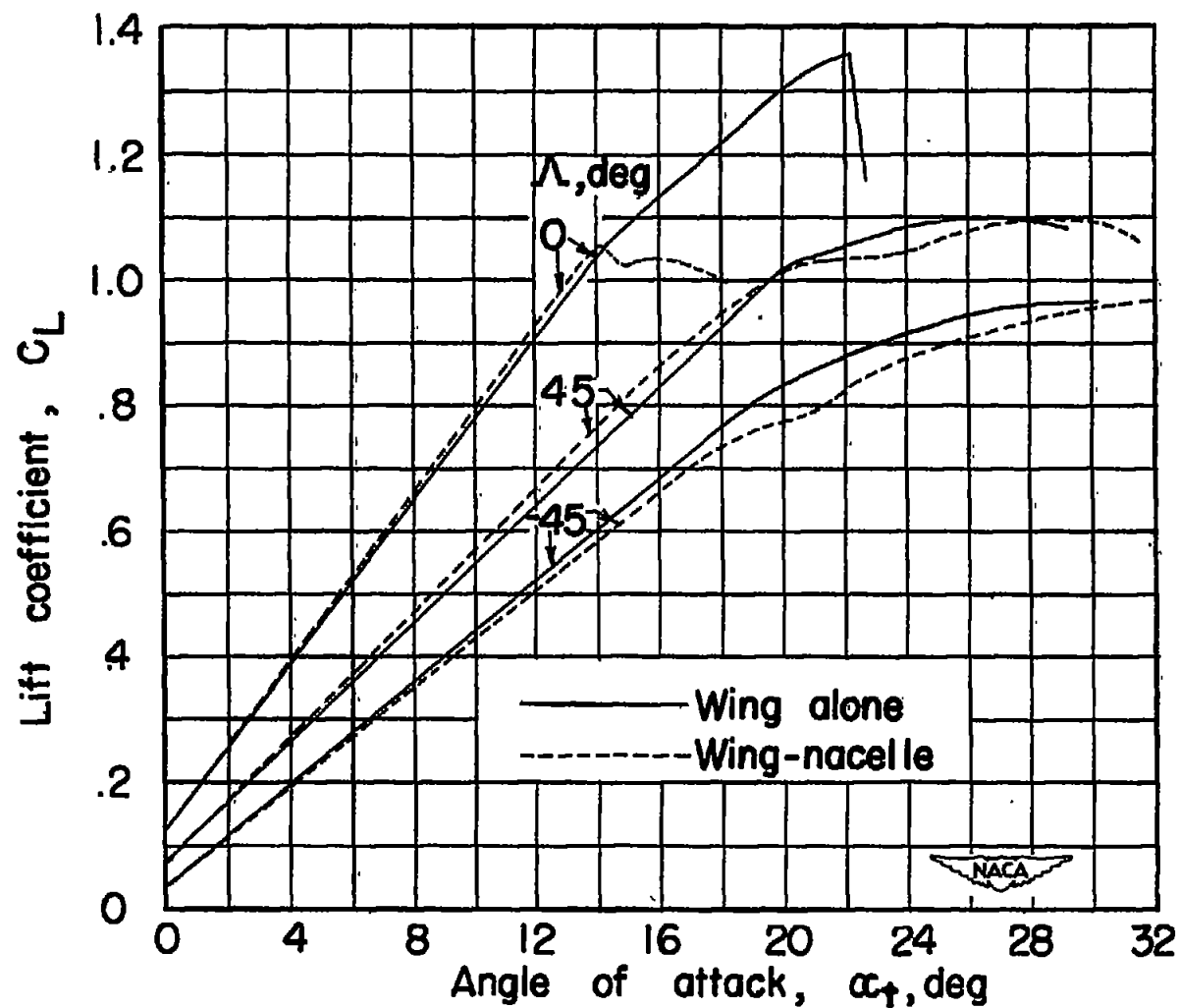
Figure 16.—Variation of lift coefficient with angle of attack for wing alone and wing-nacelle combination. M=0.13 .
