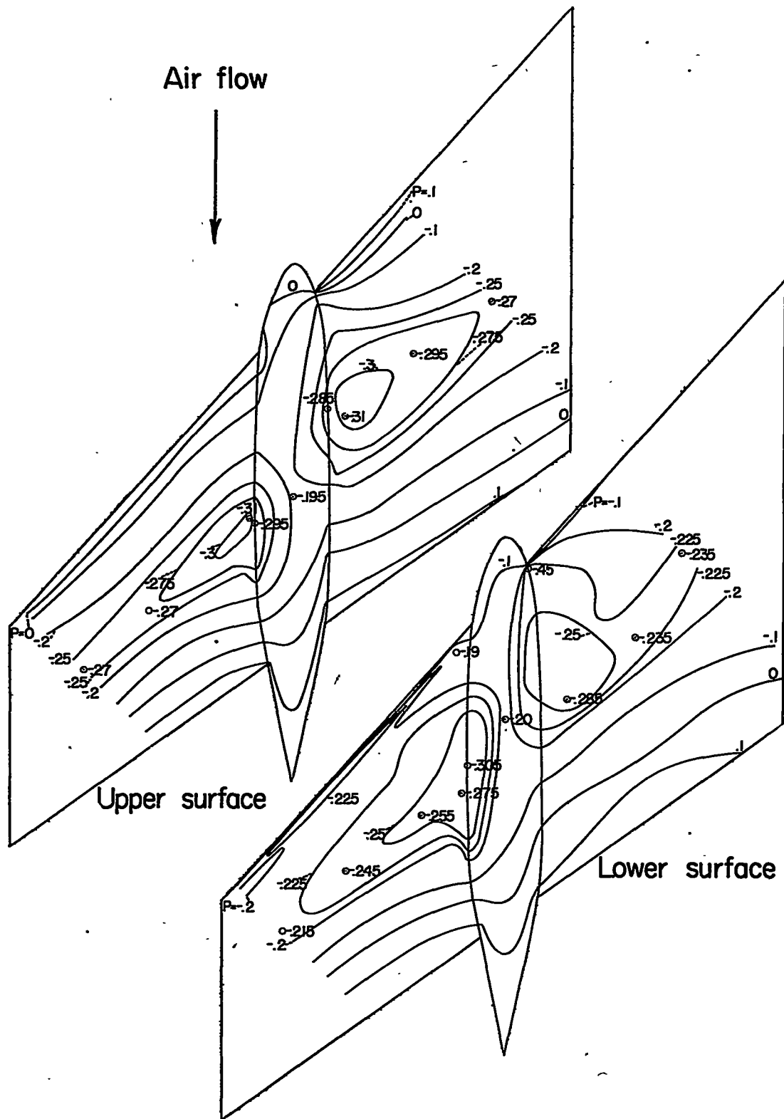
Figure 49.- Pressure contours for the wing-nacelle combination.
