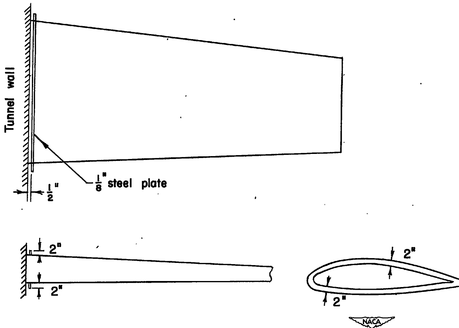
Figure 5.—Location of leakage deflection plates.
