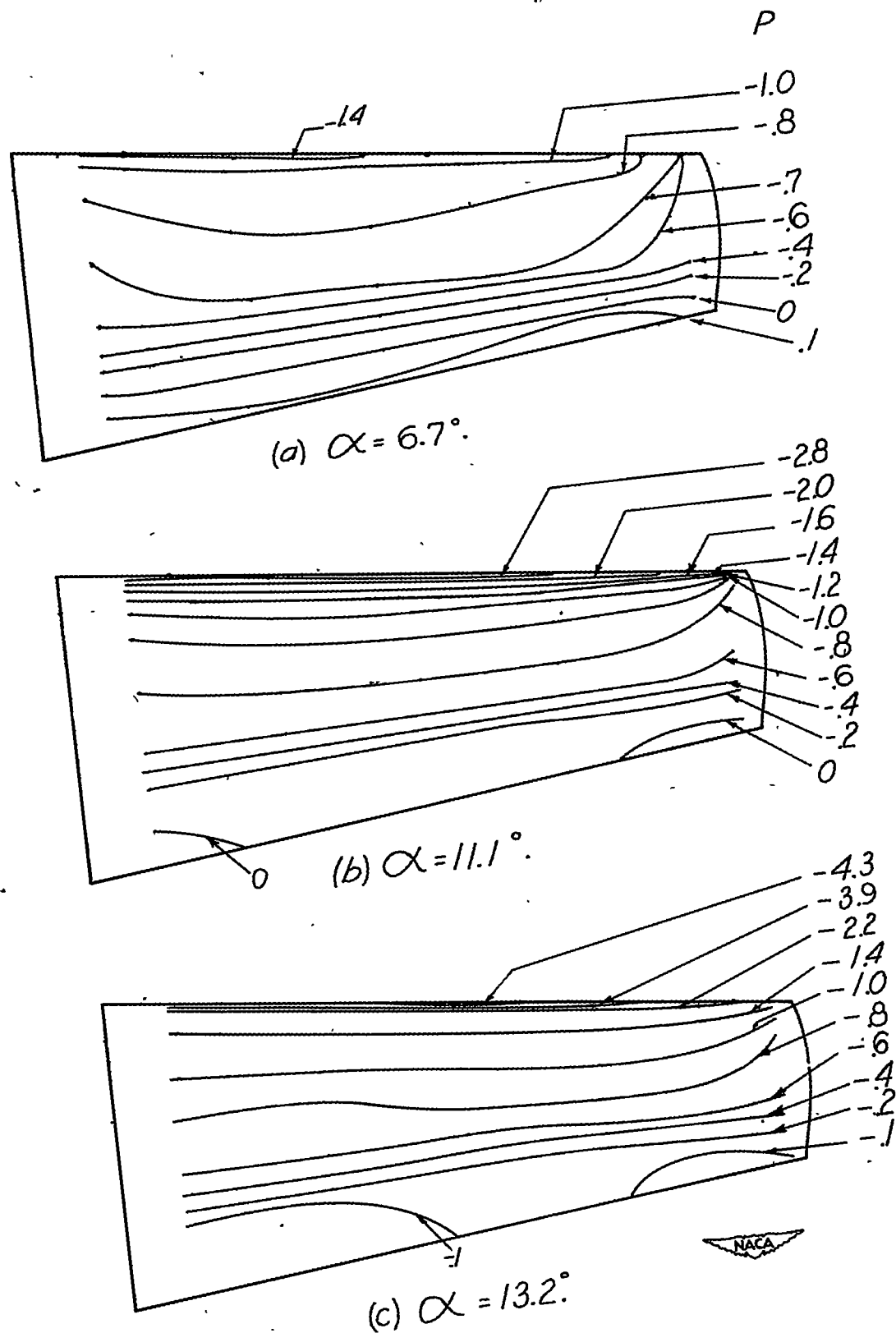
Figure 11.- Pressure contours over the upper surface of the wing for representative angles of attack for M_\infty = 0.20 .
