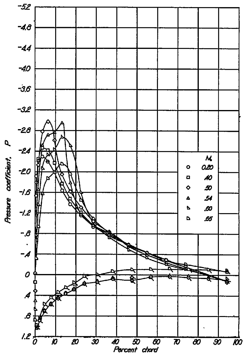
(a) NACA 230-series wing, \alpha = 11.2^\circ , \frac{y}{b/2} = 0.47 .
