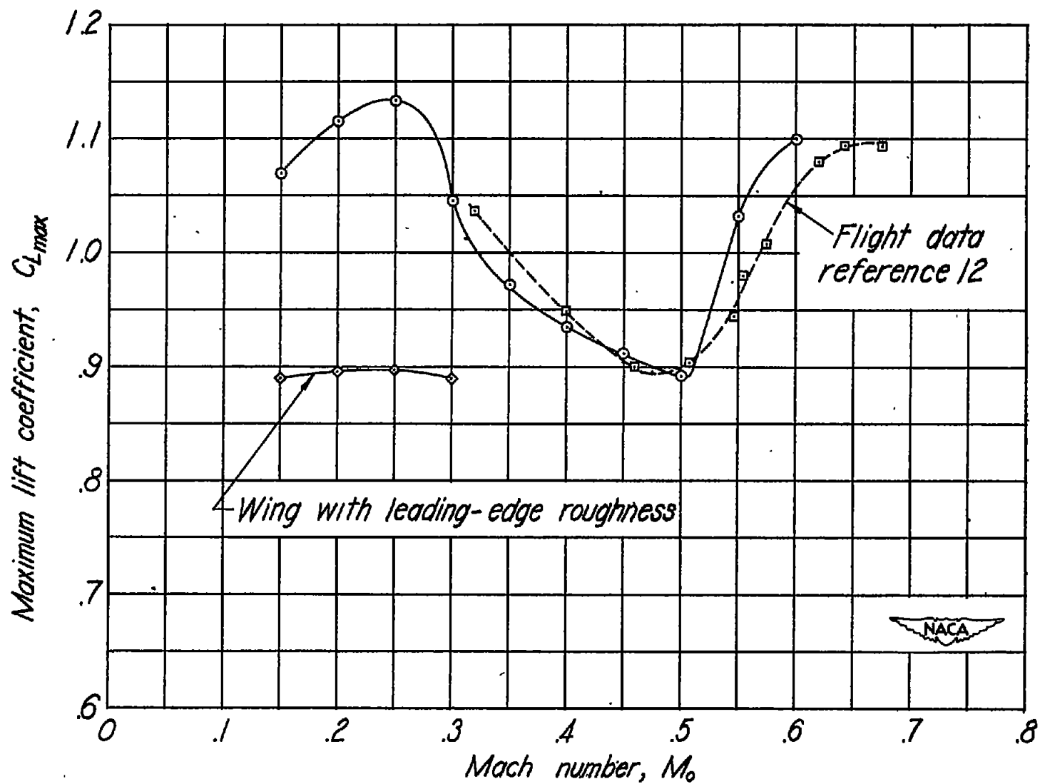
Figure 8.- Variation of maximum lift coefficient with Mach number.
