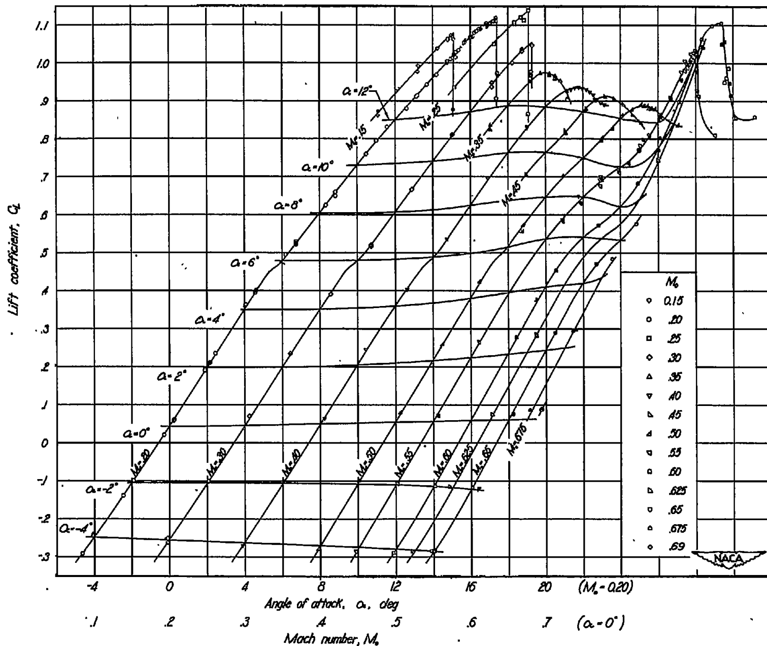
Figure 6.-Wing lift coefficient as a function of angle of attack and Mach number.
