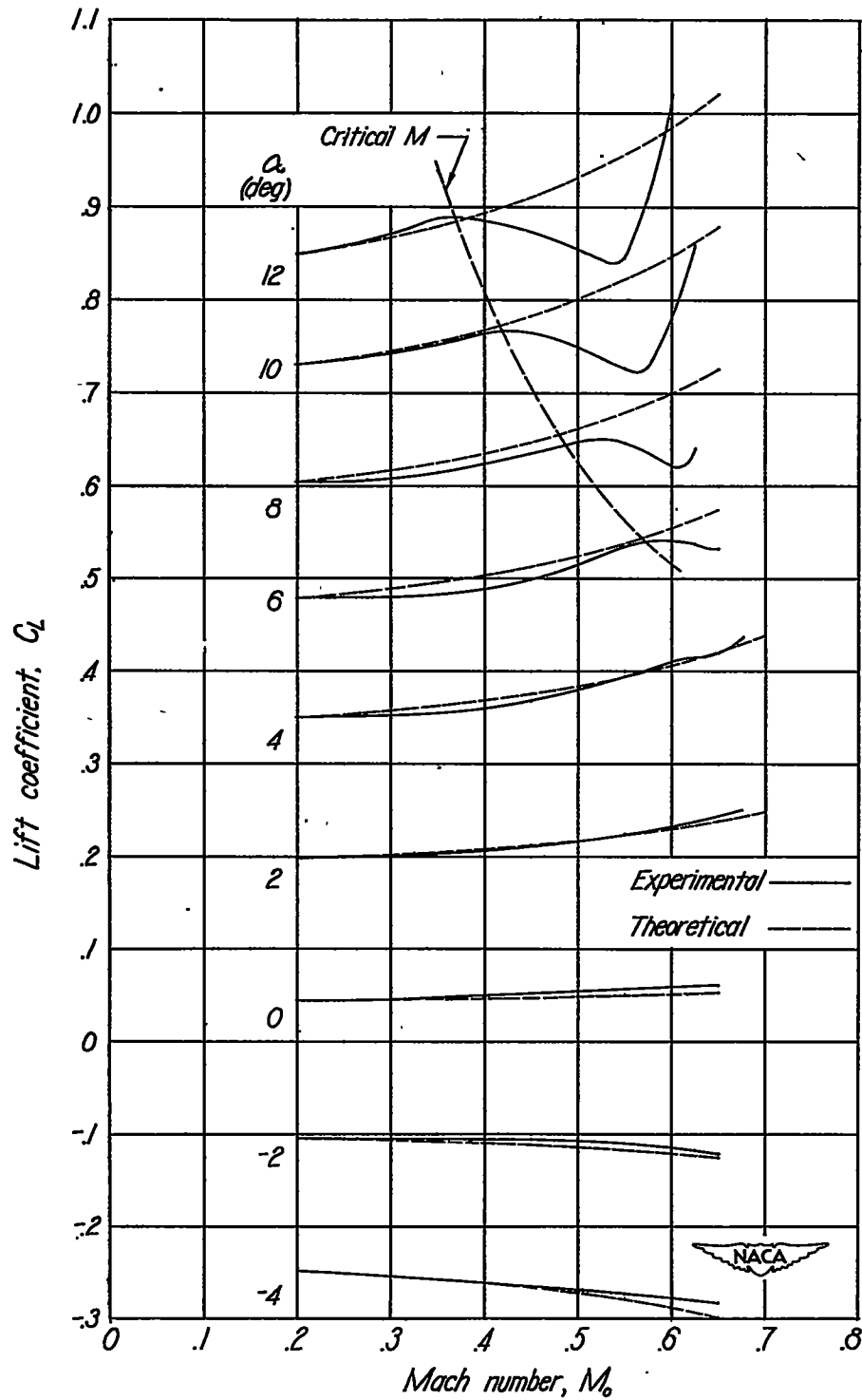
Figure 7.- Comparison of the experimental and theoretical variation of wing lift coefficient with Mach number.
