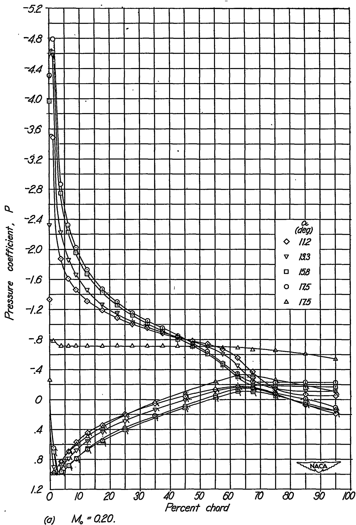
Figure 10.-Variation of section pressure distribution with angle of attack at the mid-semispan station ( y/l_2 = 0.5 ) for Mach numbers of 0.20, 0.40, and 0.60.
