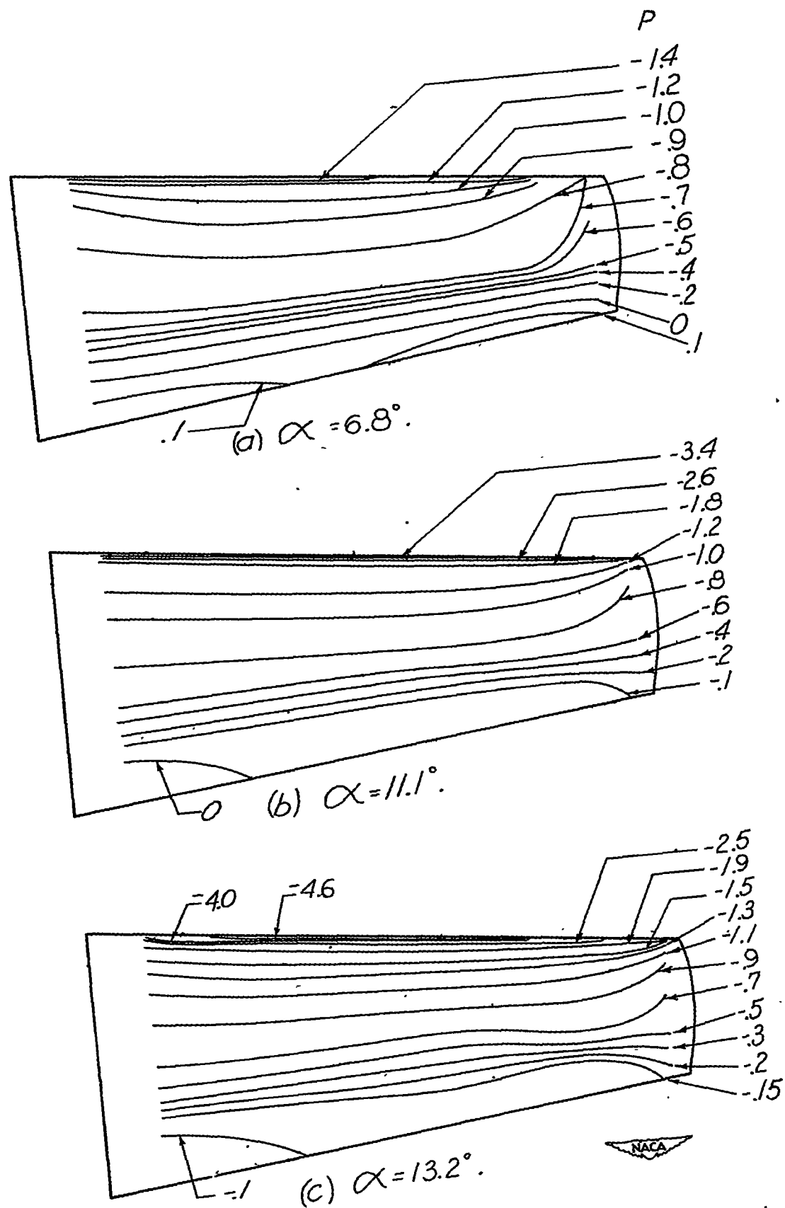
Figure 12.- Pressure contours over the upper surface of the wing for representative angles of attack for M_\infty = 0.40 .
