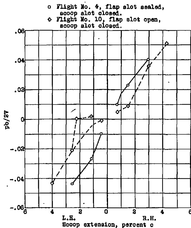
Figure 15.- Rate of roll at 100 mph, ( C_L = 1.57 ) flaps and gear down.
