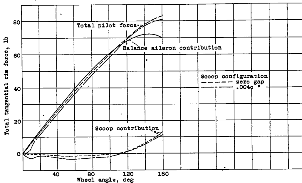
Figure 6.- Pilot-force curves.
