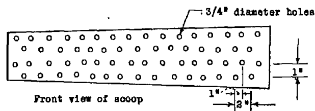
Figure 8.- Scoop geometry.
