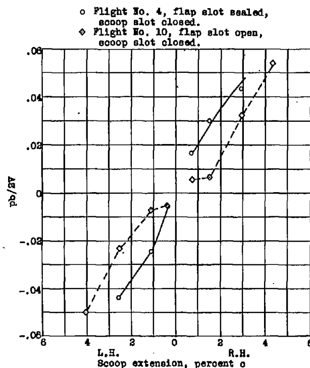
Figure 16.- Rate of roll at 160 mph, ( C_L = .81 ) flaps and gear down.
