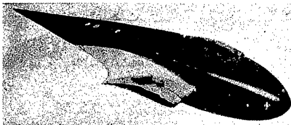
Figure 9.-Wing roots and fuselage of comparative model no. 1 with filleting.
