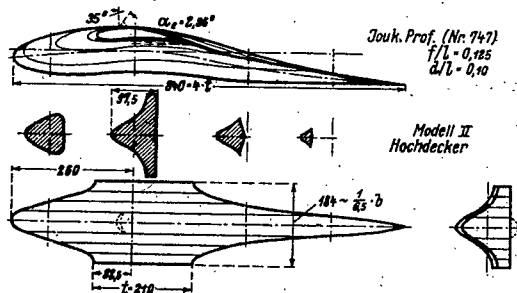
Figure 24.-High-wing.
