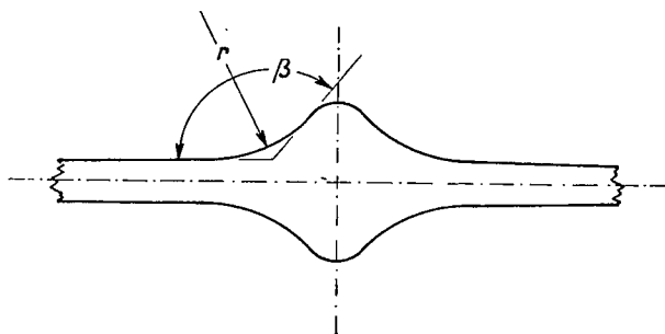
Figure 3.-Front view of aerodynamically beneficial filleting.
