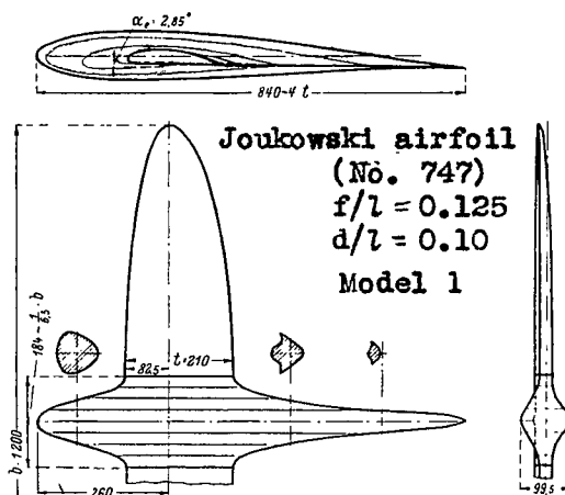
Figure 4.-Wing and fuselage with fuselage faired smoothly into the wing. (Model no.1)
