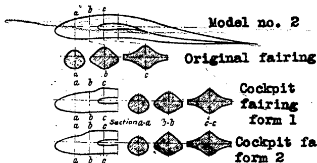
Figure 28.-Model no. 2 with cockpit fairing.
