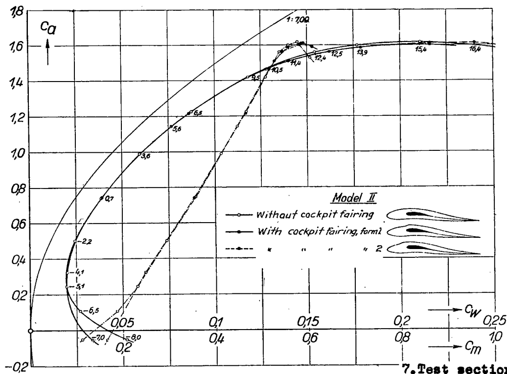
Figure 29.-Polar diagrams of model no. 2 with and without cockpit fairings.
