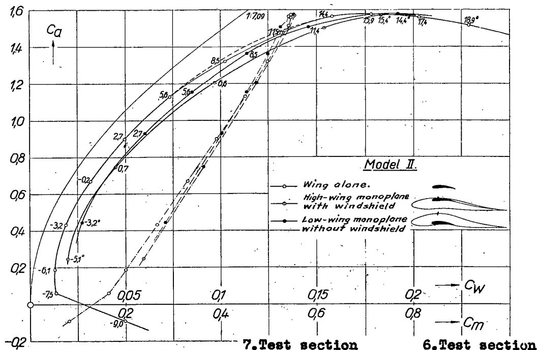
Figure 27.-Polar diagrams of "wing alone" and high and low wing with windshield.
