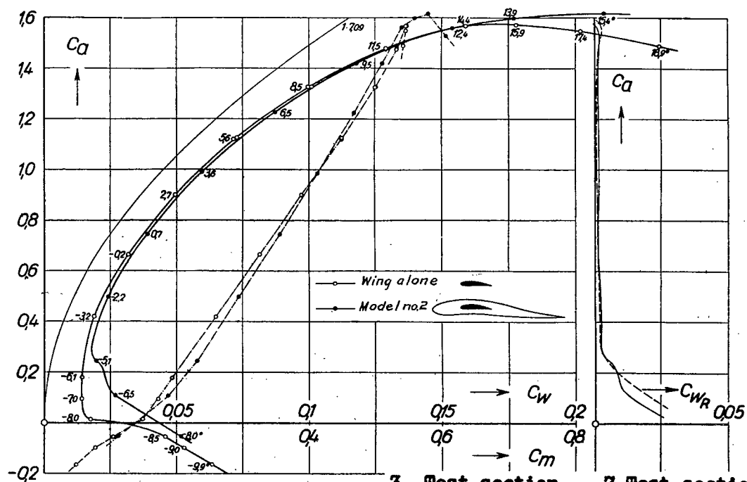
Figure 21.-Polar diagram of "wing alone" and model no. 2.
