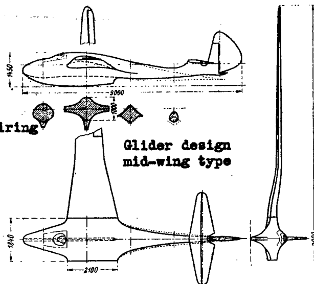
Figure 30.-Design of glider (mid-wing type) with fuselage adapted to flow around the wing.
