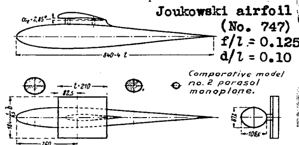
Figure 10.-Comparative model no.2 ; parasol type.
