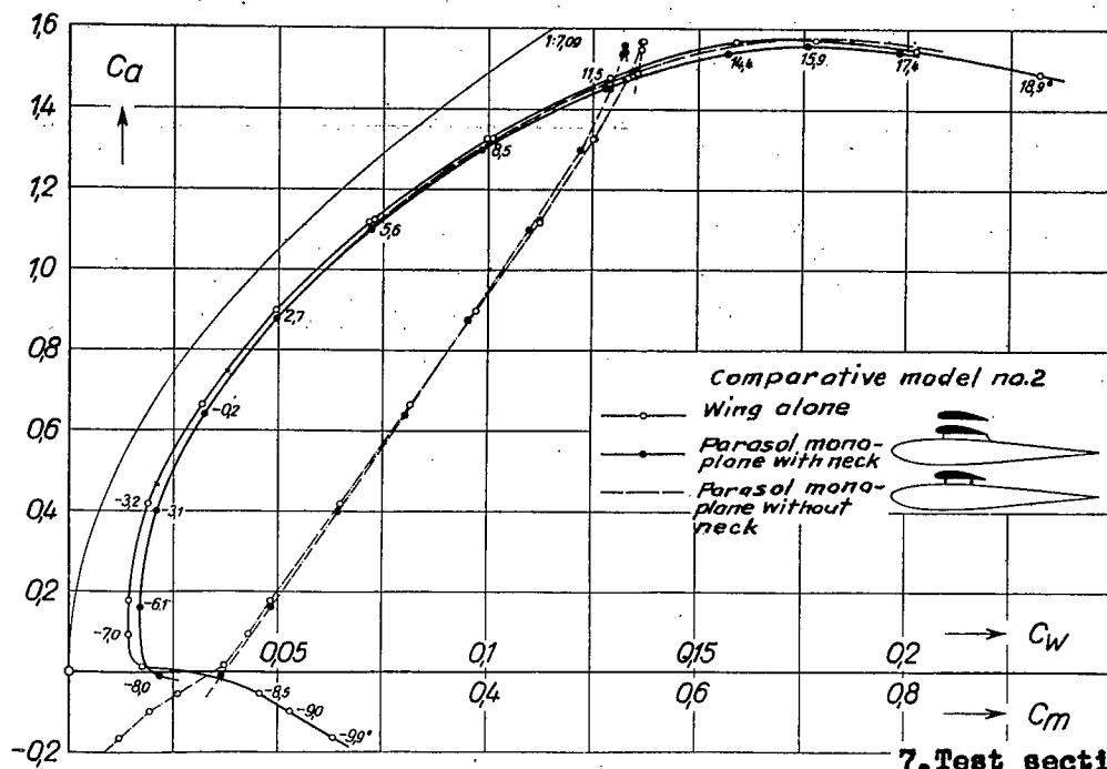
Figure 14.-Polar diagram of "wing alone" and of comparative model no.2 .
