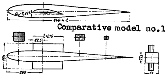
Figure 7.-Comparative model: wing with square fuselage (mid-wing type).
