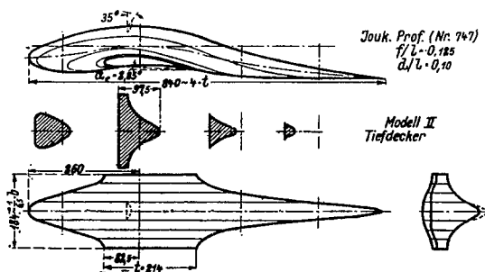
Figure 20.-Comparison of bodies of models no.1 and 2 .
