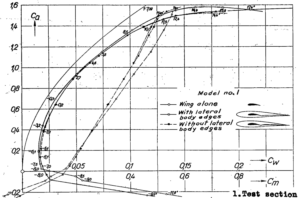
Figure 12.-Polar diagram of "wing alone" and of model no.1 .
