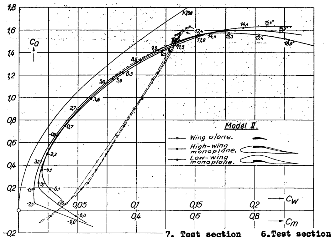
Figure 26.-Polar diagrams of "wing alone" and of high and low wing.
