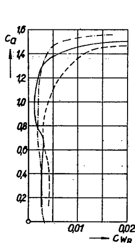
Figure 15.- Body drag coefficients of model no.1 and comparative models nos.1 and 2 .
