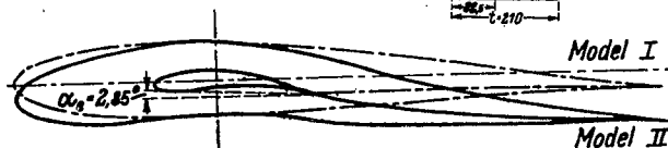
Figure 20.-Comparison of bodies of models no.1 and 2 .
