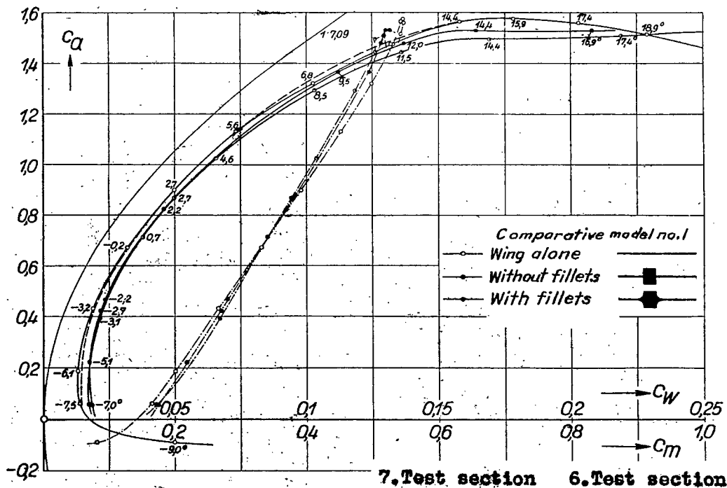
Figure 13.-Polar diagram of "wing alone" and of comparative model no.1 .
