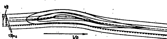
Figure 17.-Adaptation of fuselage to flow around wing.
