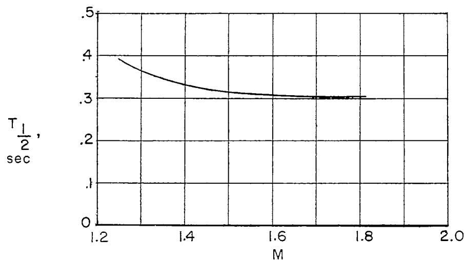
(a) Time for pitching oscillation to damp to one-half amplitude.
