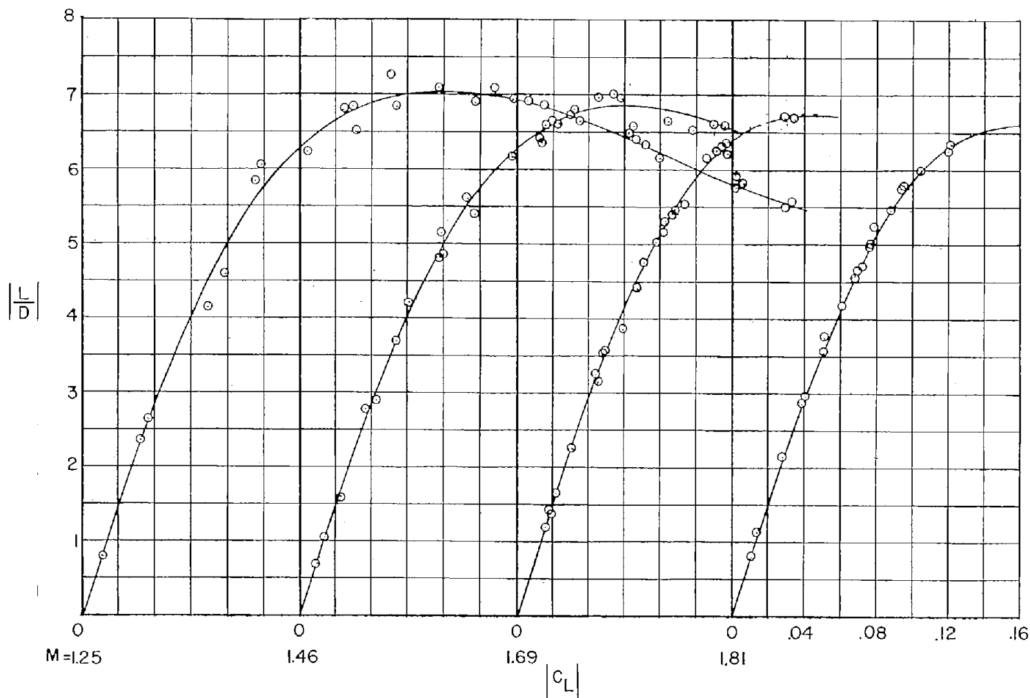
Figure 14.- Lift-drag ratio plotted against lift coefficient.
