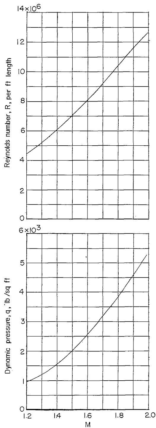
Figure 8.- Flight test conditions.
