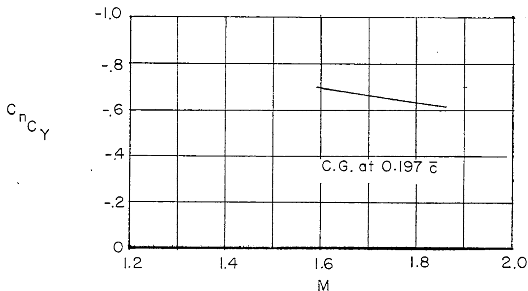
(b) Static stability parameter in yaw C_{nCY} .
