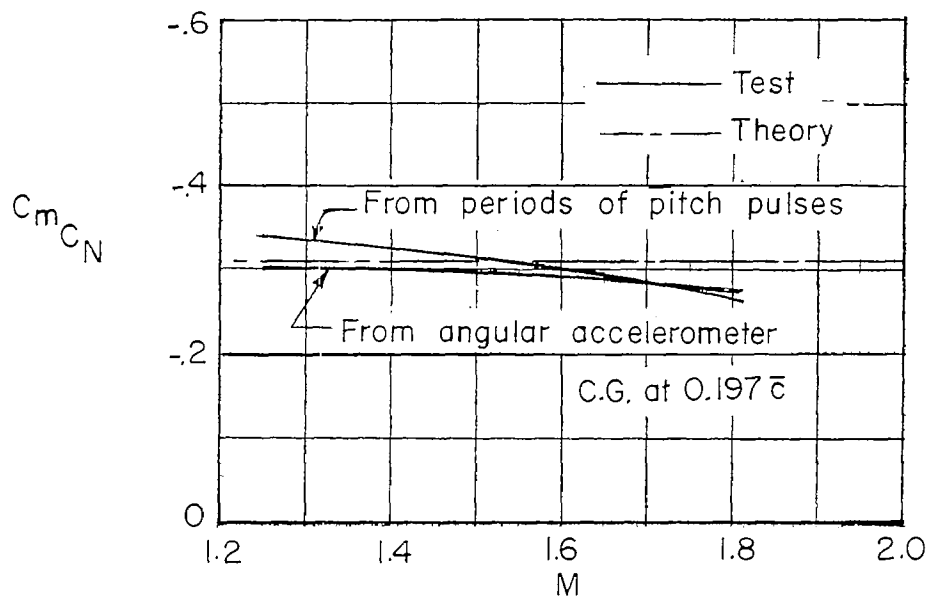
(b) Static stability parameter in pitch C_{mC_N} .
