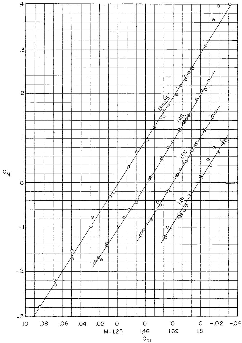
Figure 17.- Variation of normal-force coefficient with pitching-moment coefficient.
