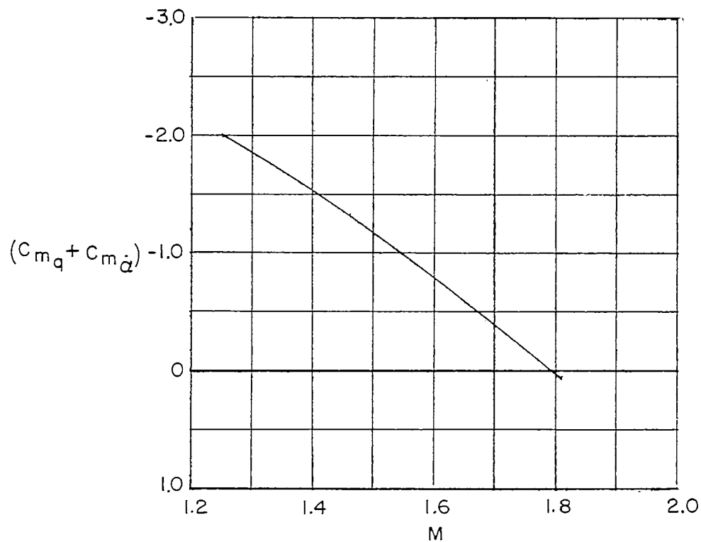
(b) Rotary damping derivatives.
