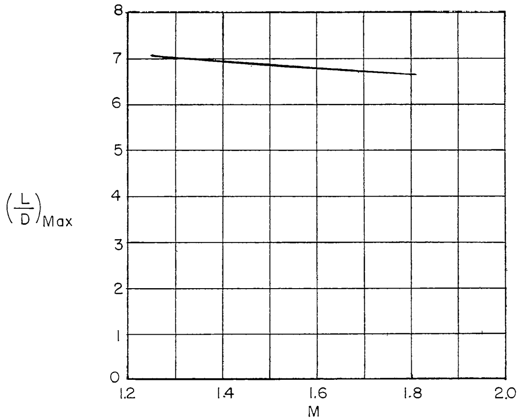
(a) Maximum lift-drag ratio.
