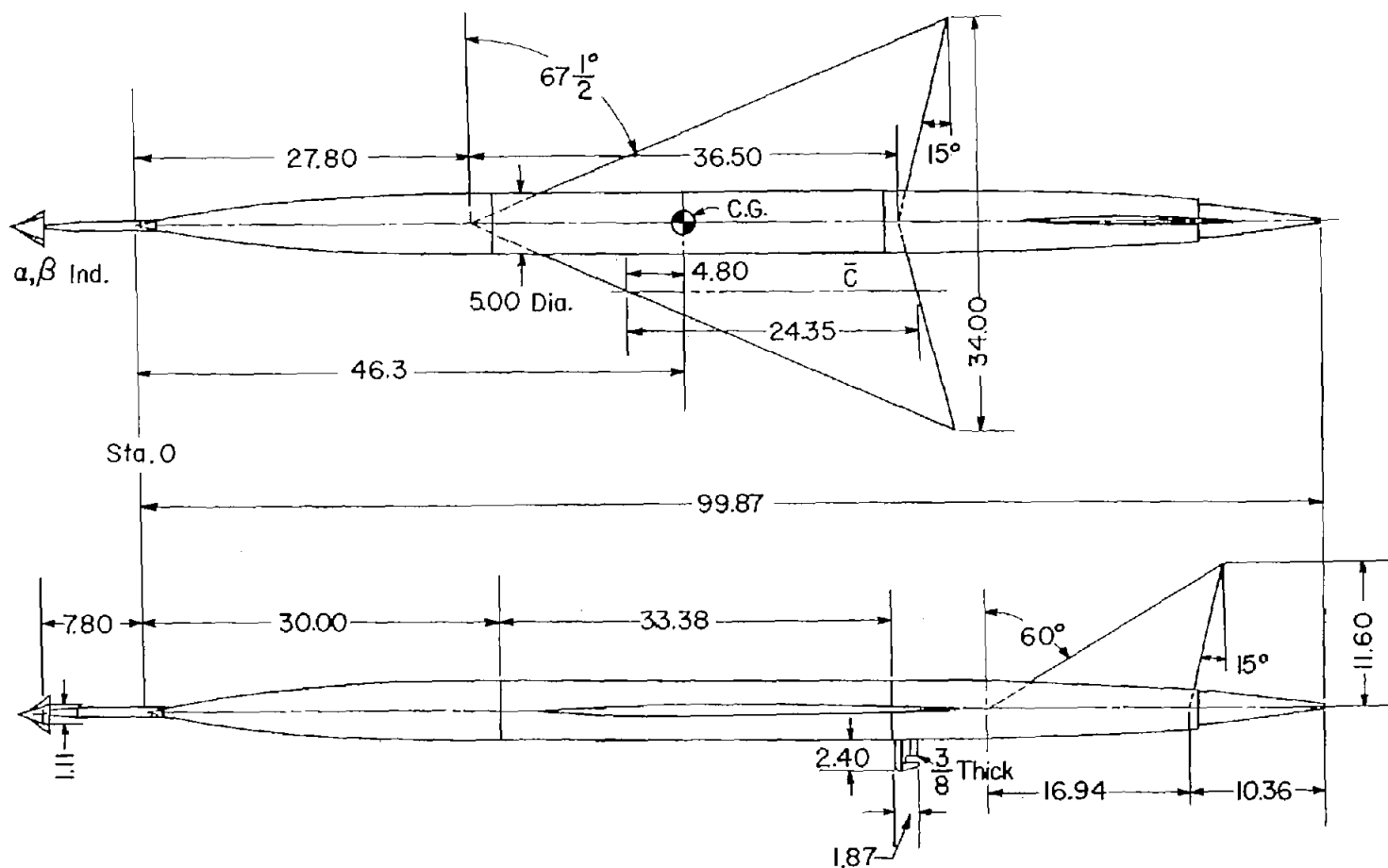
Figure 2.- Test configuration. All linear dimensions are in inches.
