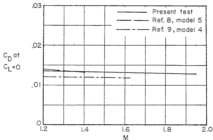
(a) Drag coefficient at C_L = 0 .
