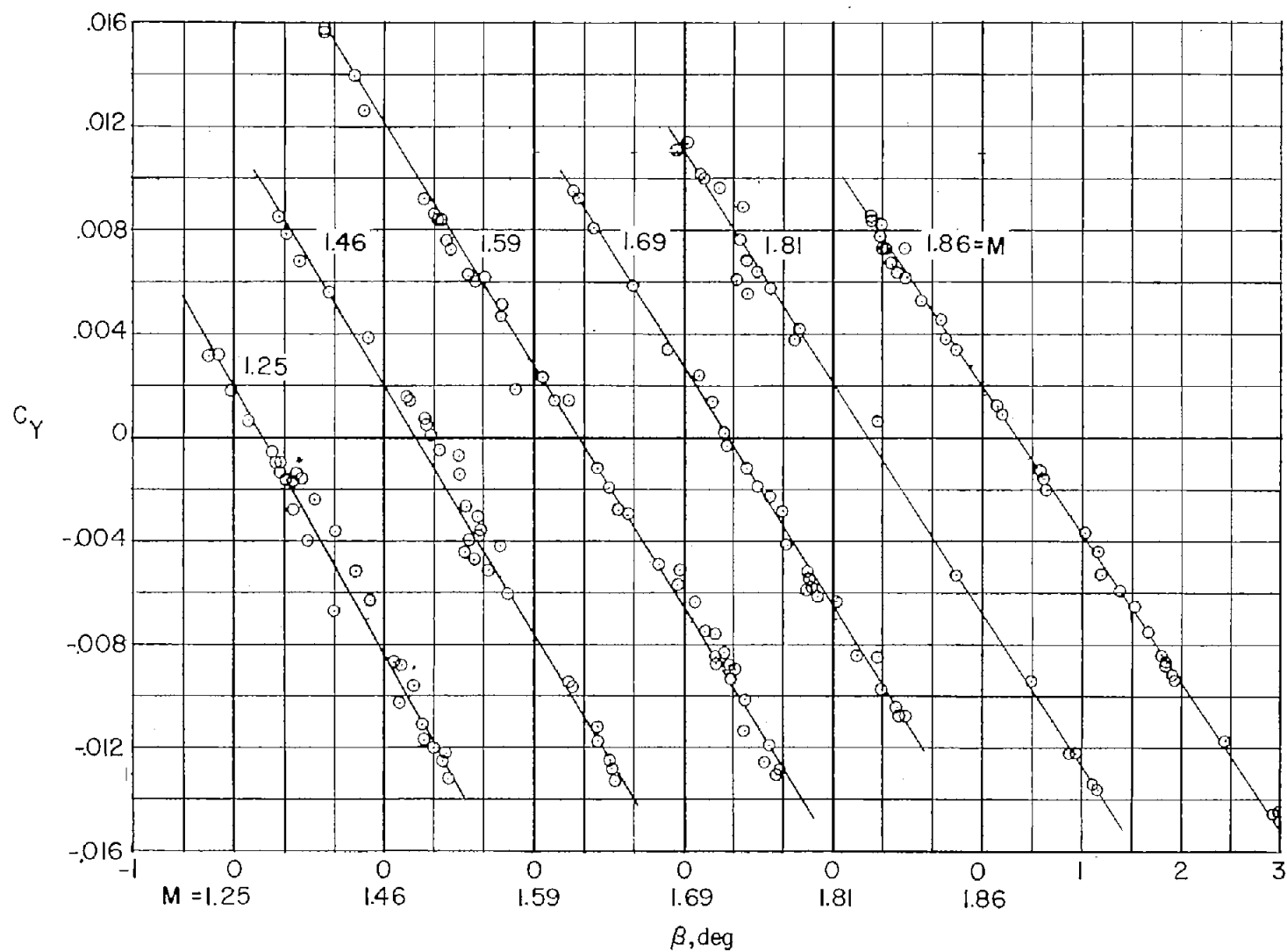
Figure 20.- Variation of side-force coefficient with angle of sideslip.
