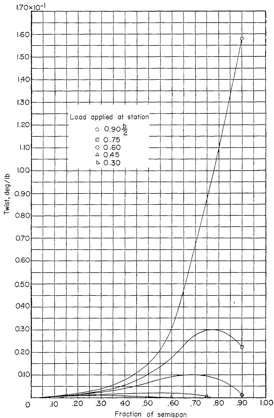
Figure 7.- Tail streamwise average twist resulting from a concentrated load applied along 50-percent-chord line.
