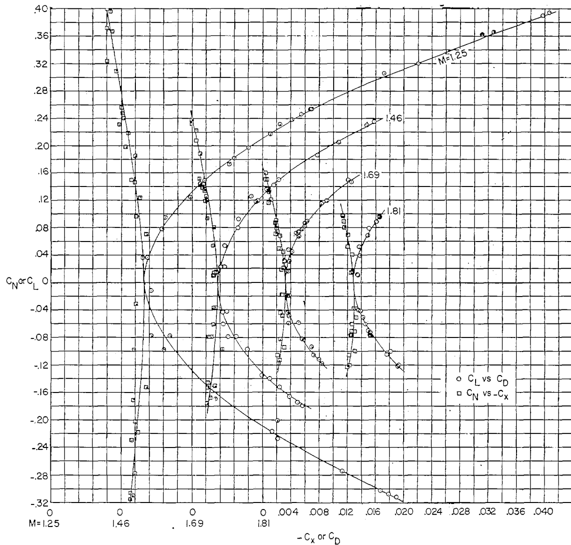
Figure 12.- Variation of normal-force coefficient with axial-force coefficient and lift coefficient with drag coefficient at constant Mach numbers.
