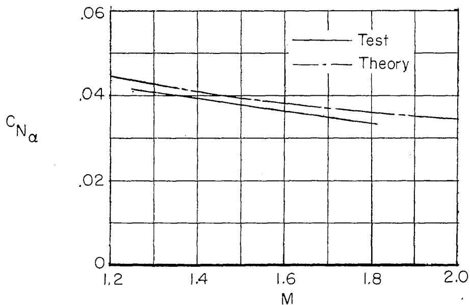
(a) Normal-force-curve slope C_{N\alpha} .
