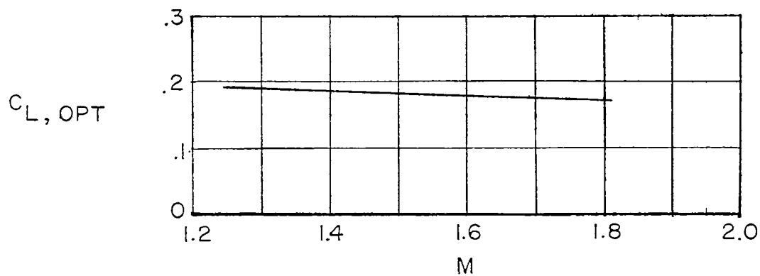
(b) Lift coefficient at \left(\frac{L}{D}\right)_{\text{max}} .
