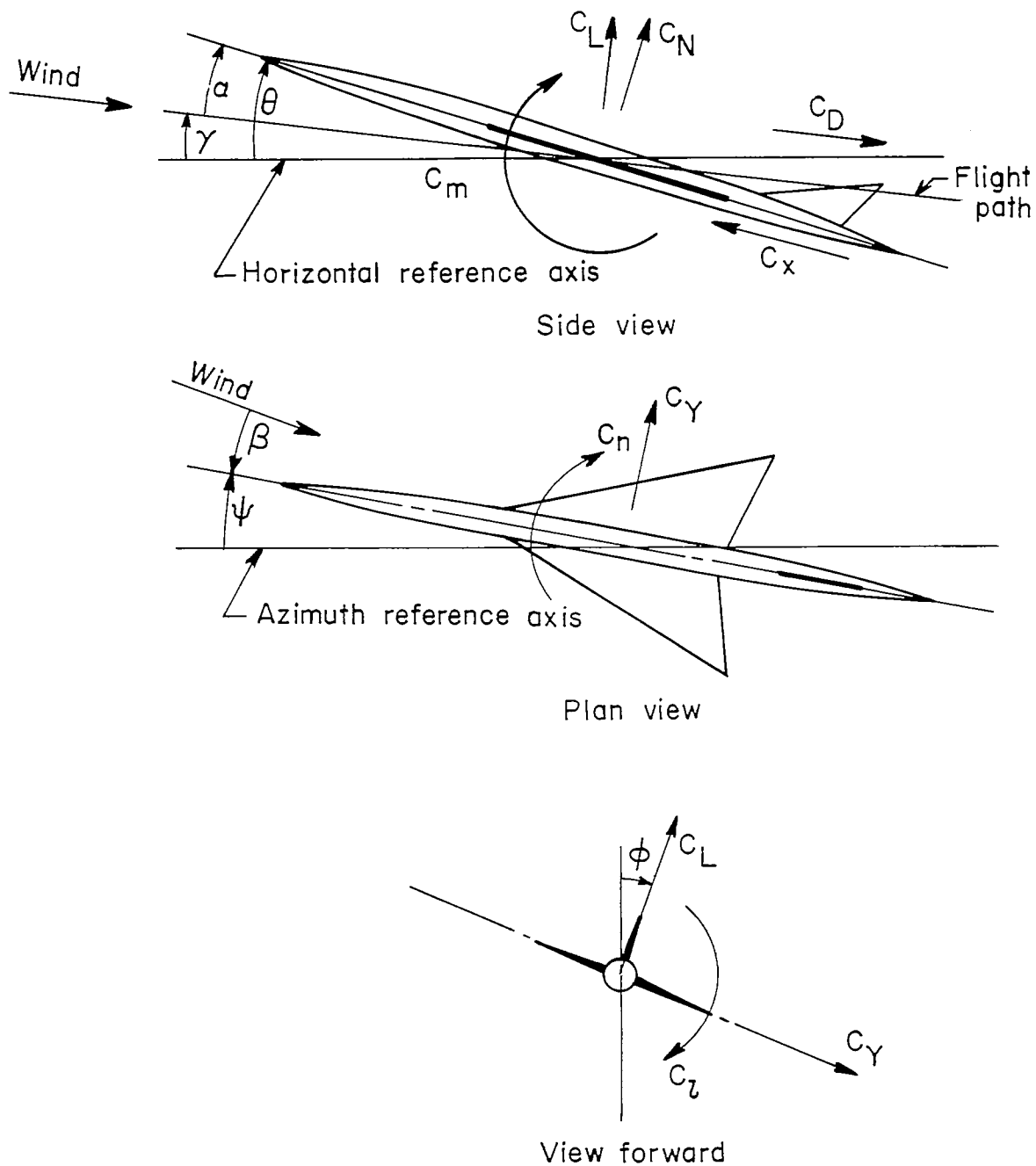
Figure 1.- System of axes. Arrows indicate positive directions; origin is at center of gravity.
