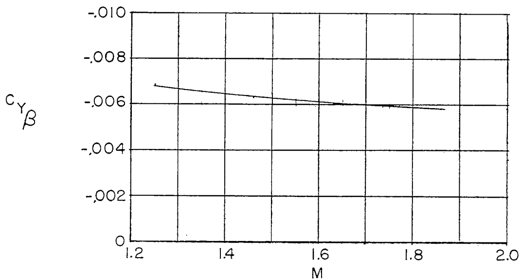
(a) Side-force-curve slope C_{Y\beta} .
