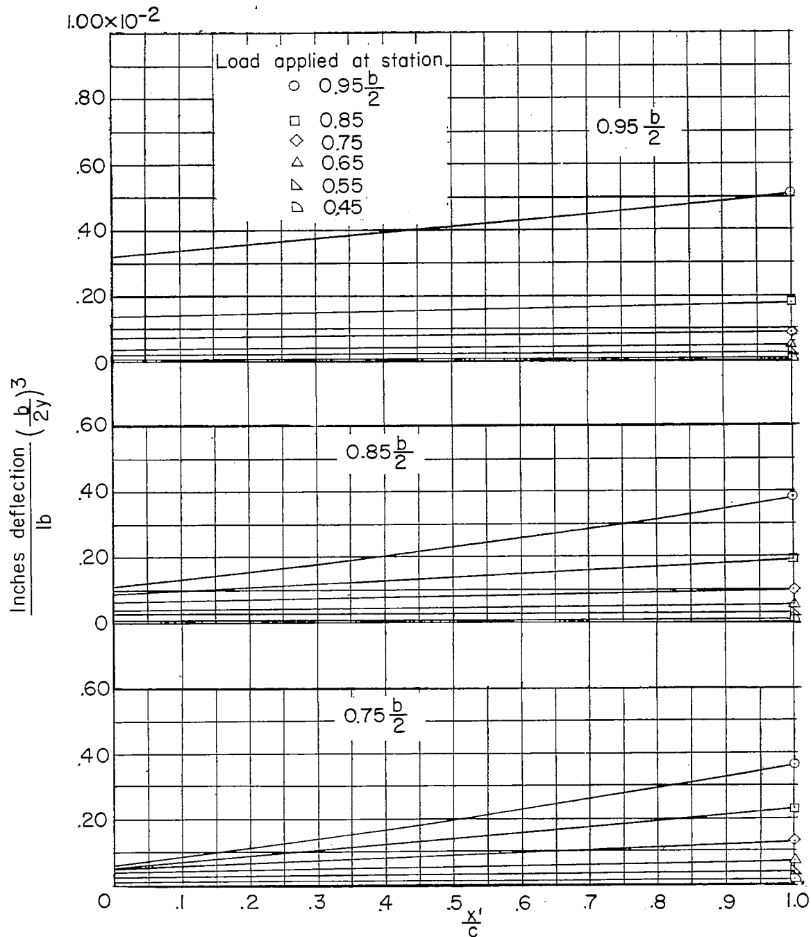
Figure 5.- Wing static deflection resulting from a concentrated load applied along 50-percent-chord line.
