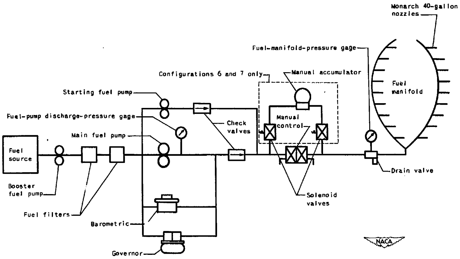
Figure 4. - Schematic diagram of standard fuel system of I-40 jet-propulsion engine with barometric and 40-gallon nozzles (configurations 1 to 7).
