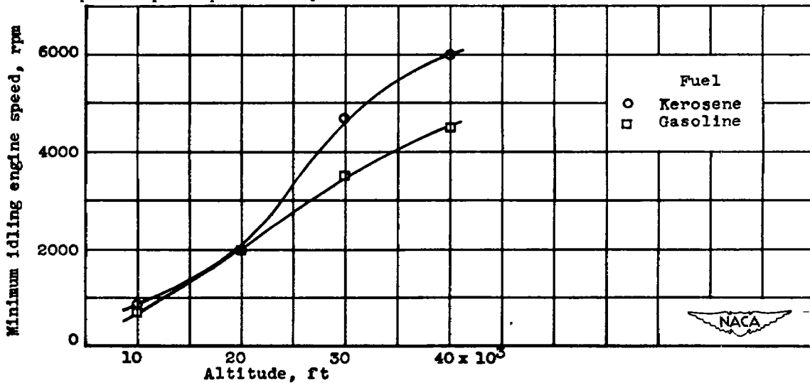
Figure 17.- Effect of altitude and fuel on minimum idling speed of I-40 jet-propulsion engine equipped with Syracuse barometric fuel control (configuration 9). Free-stream impact pressure, 40 pounds per square foot.
