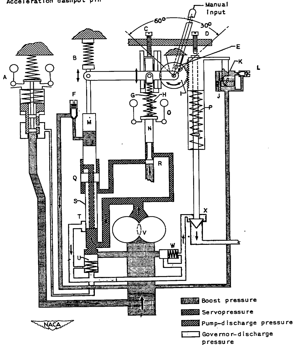
Figure 35. - Schematic diagram of Woodward fuel governor.
