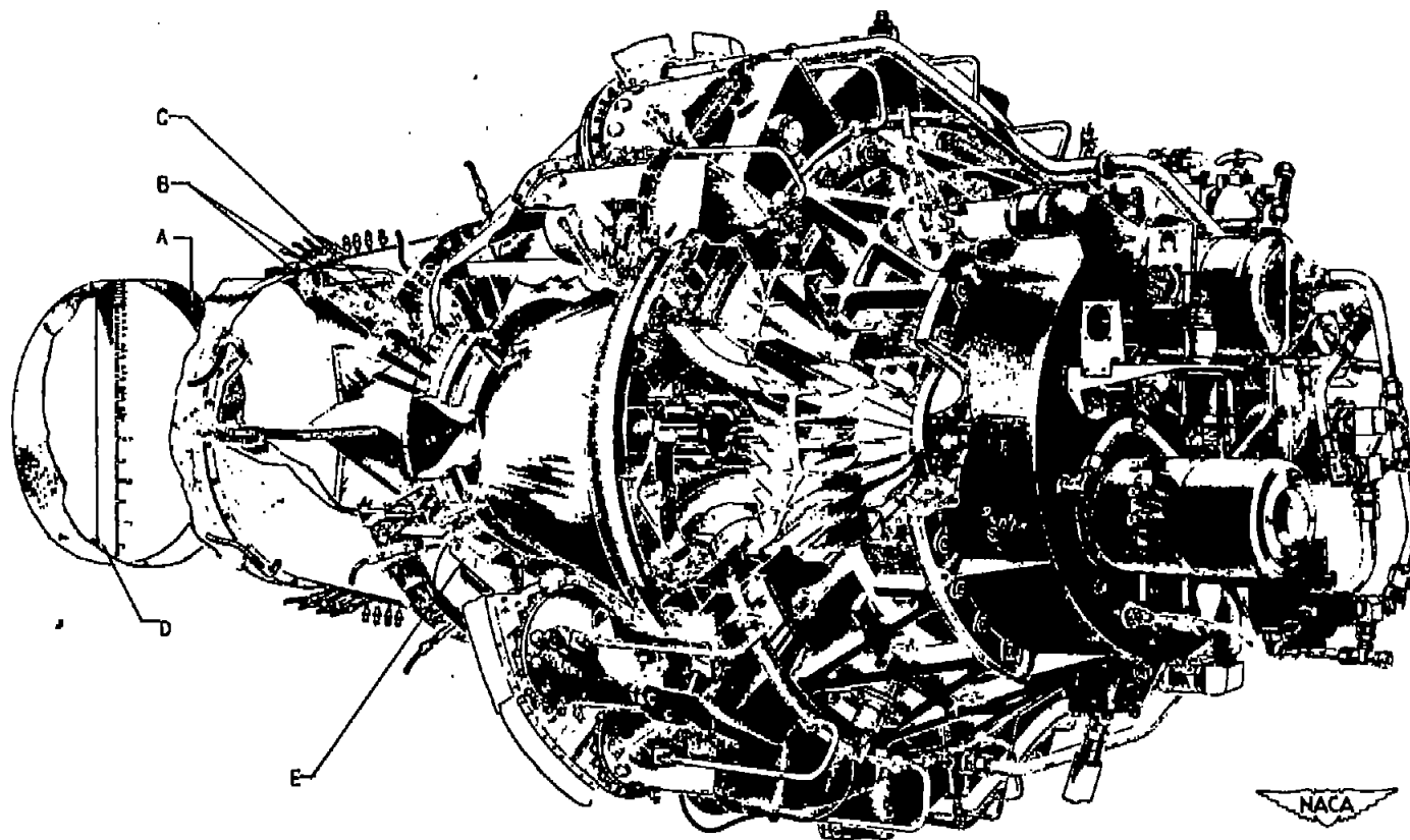
Figure 3. - Drawing of L-40 jet-propulsion engine showing location of instrumentation.
