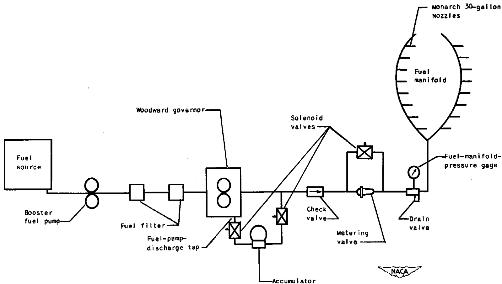
Figure 8.- Schematic diagram of fuel system of 1-40 jet-propulsion engine with Woodward governor and 30-gallon nozzles (configuration 12). Woodward governor incorporates main fuel pump, main governor, overspeed governor, relief valve, and manual-control valve.
