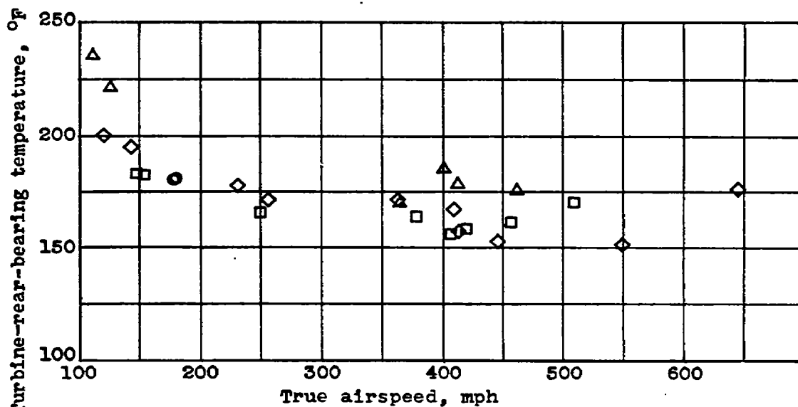
Figure 29.- Effect of airspeed and altitude on turbine-rear-bearing temperature at engine speed of 11,500 rpm. Airspeed based on 100-percent free-stream total-pressure recovery.
