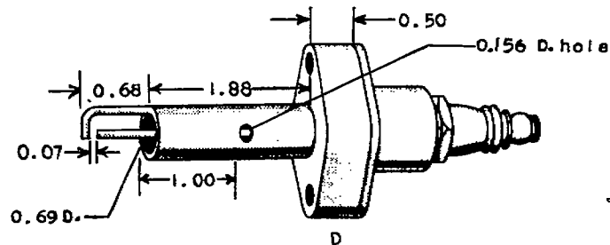
Figure 12. - Modifications of Champion D8 spark plug used in wind-tunnel investigation of I-40 jet-propulsion engine. (All dimensions in in.)
