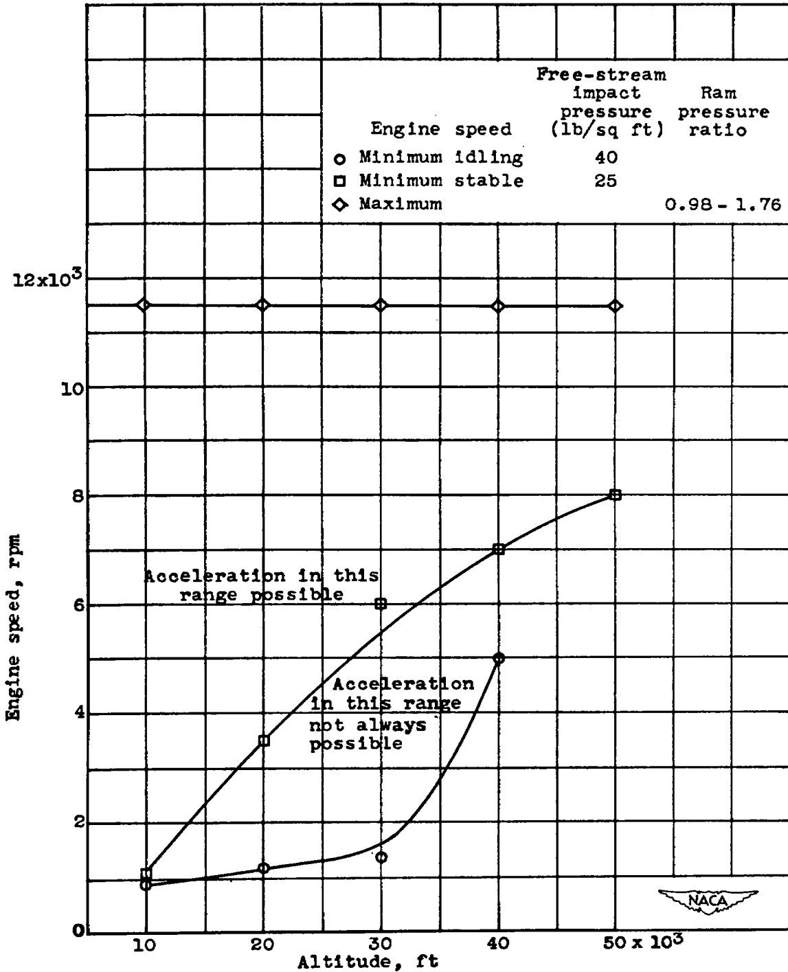
Figure 14.- Effect of altitude on operating range of I-40 jet-propulsion engine equipped with standard fuel system (configurations 1 to 7).
