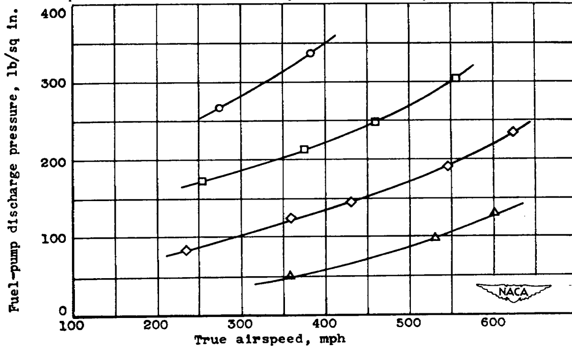
Figure 20.- Effect of airspeed and altitude on fuel-pump discharge pressure during windmilling of I-40 jet-propulsion engine (configurations 1-7). Airspeed based on 100-percent free-stream total-pressure recovery.
