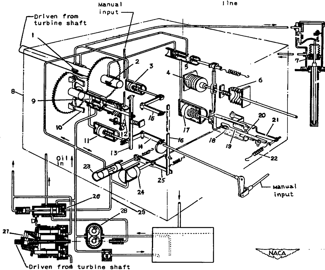
Figure 34.- Schematic diagram of Edwards fuel regulator.
