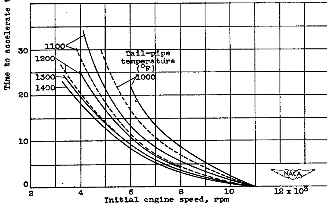
(b) Effect of tail-pipe temperature at altitude of 20,000 feet.
