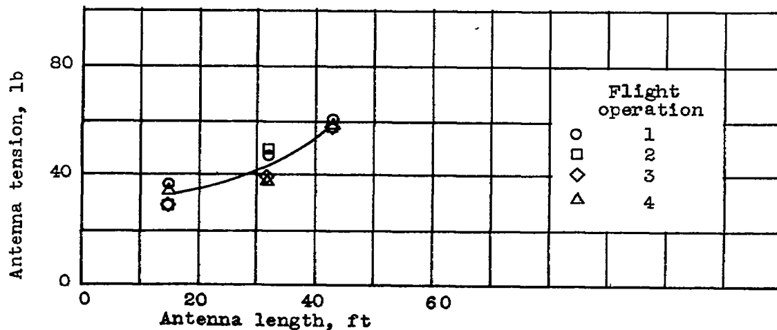
Figure 10. - Variation of antenna tension with antenna length at antenna angle of 15°. Distance flown in icing region, 115 miles.
