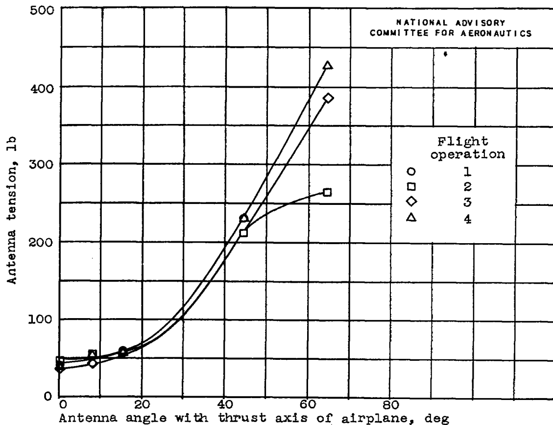
Figure 9. - Variation of antenna tension with antenna angle for antennas of 40, 41, 42, and 43 feet in length. Distance flown in icing region, 115 miles.
