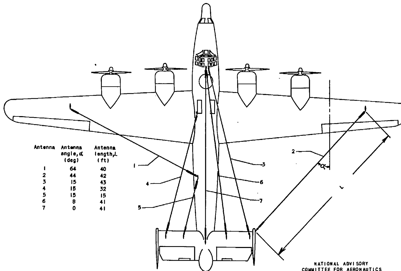
Figure 1. - Location of experimental antennas on airplane and angle and length of antennas.
