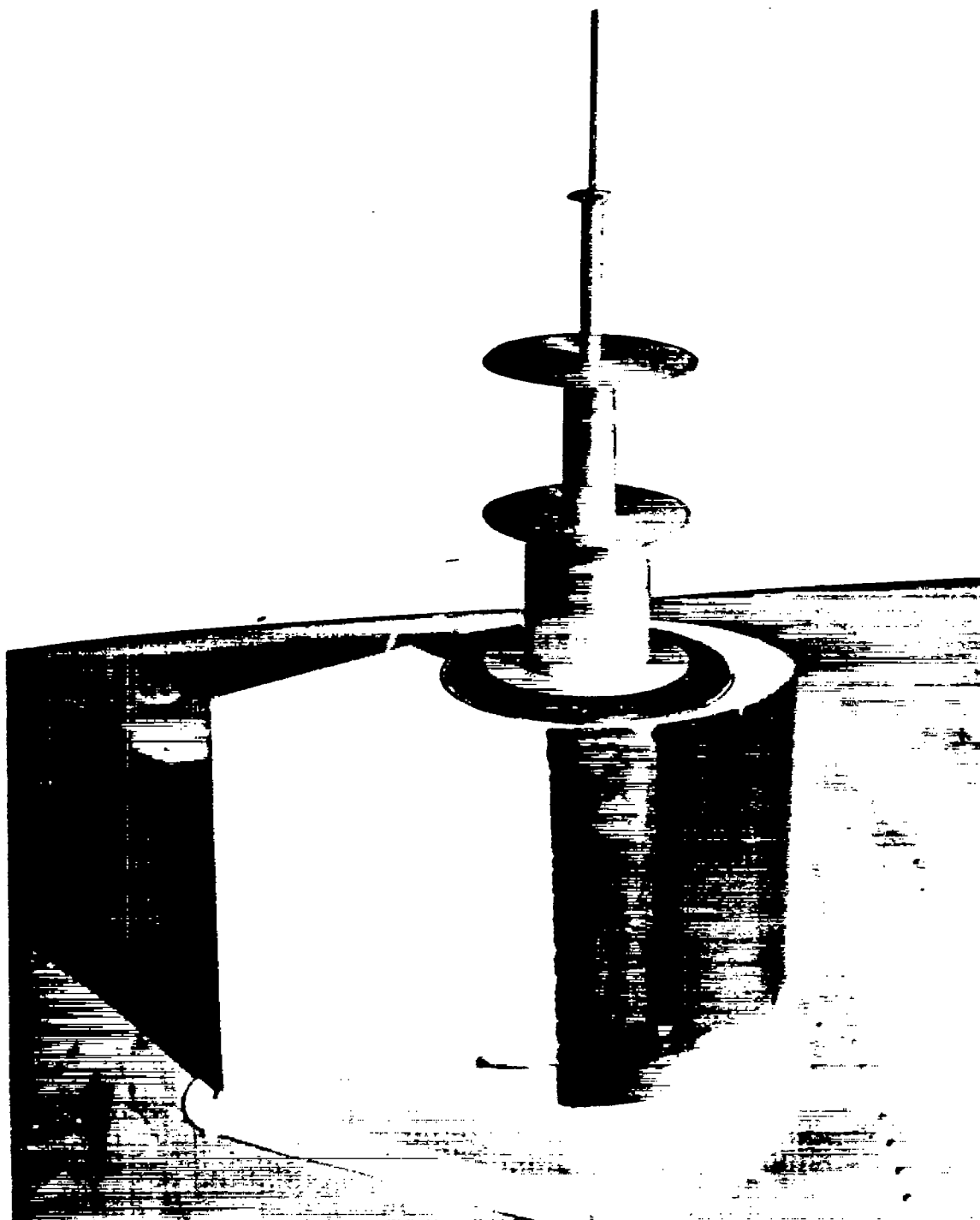
Figure 4. - Multirotating cylinder extended into air stream for collection of meteorological data.
