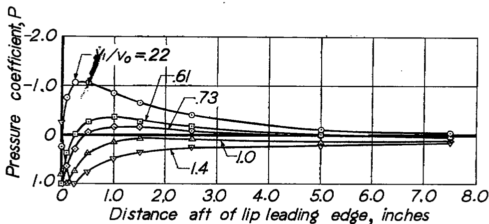
(b) Lip outer surface.
