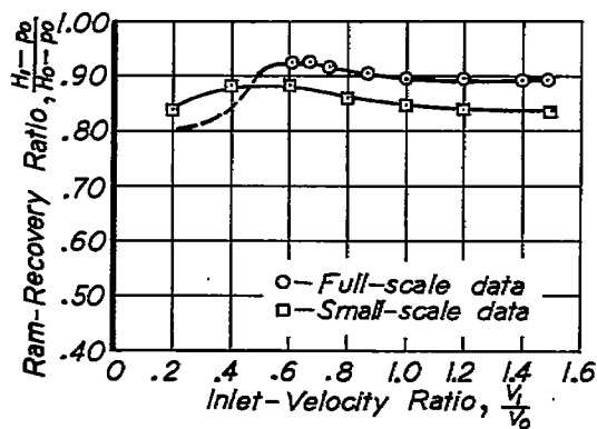
(a) 5° ramp, standard divergence.
