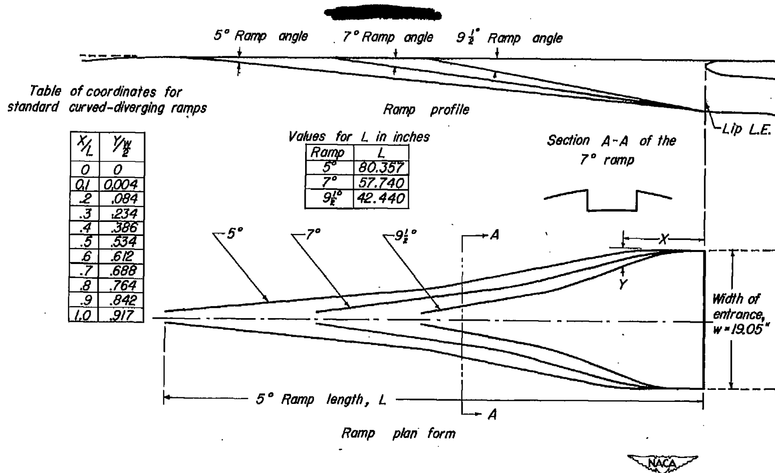
Figure 4.- Coordinates of the standard curved-diverging ramp configurations tested on the full-scale model.
