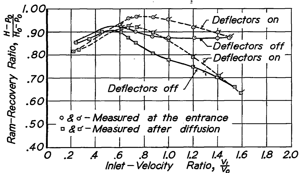
(a) 7° ramp, standard divergence
