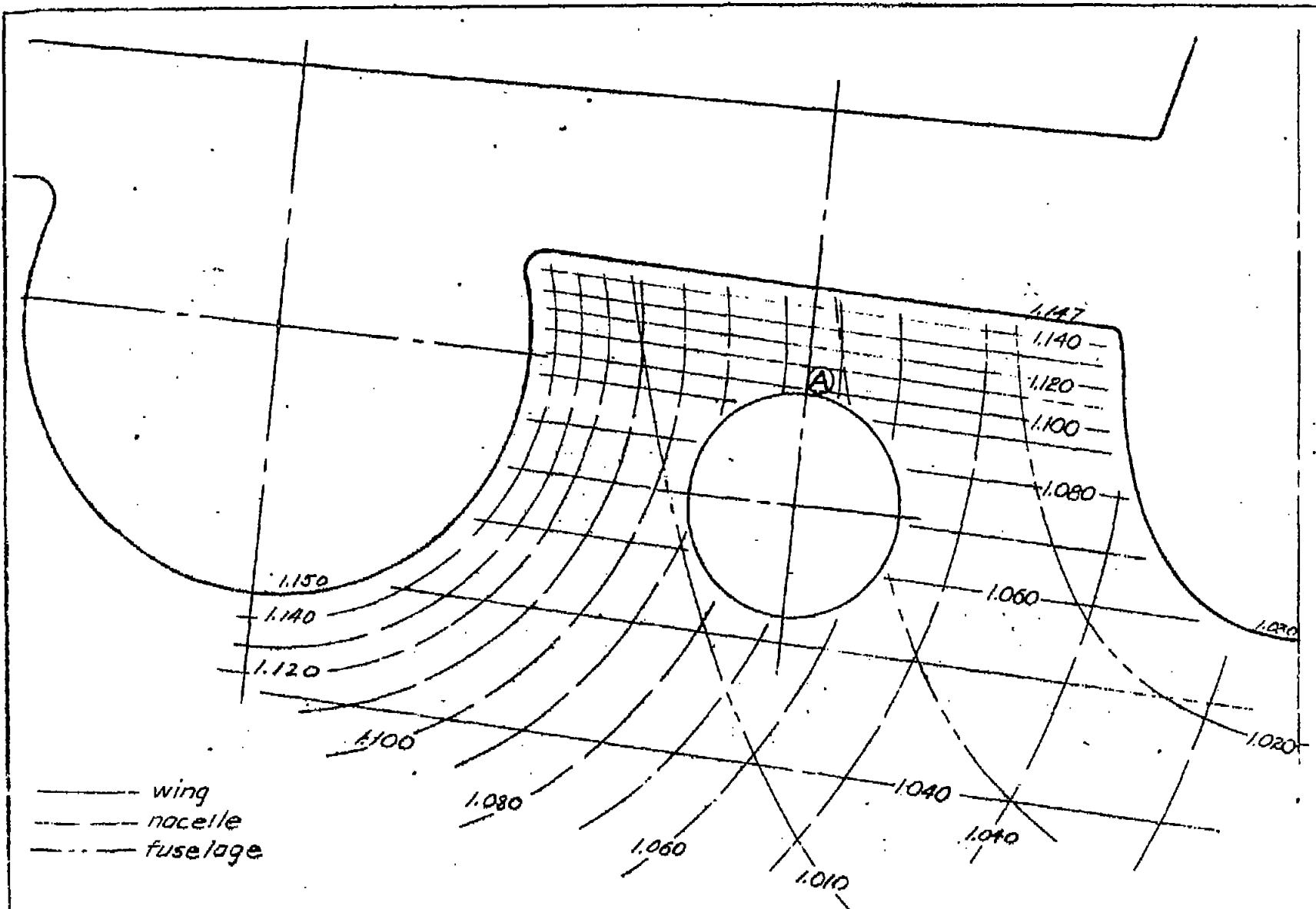
Fig. 11 - Velocity-ratio distribution in the region of the wing external store attachment position, 30% wing chord, Grumman F7F-3 airplane, C_L = 0.10 .
