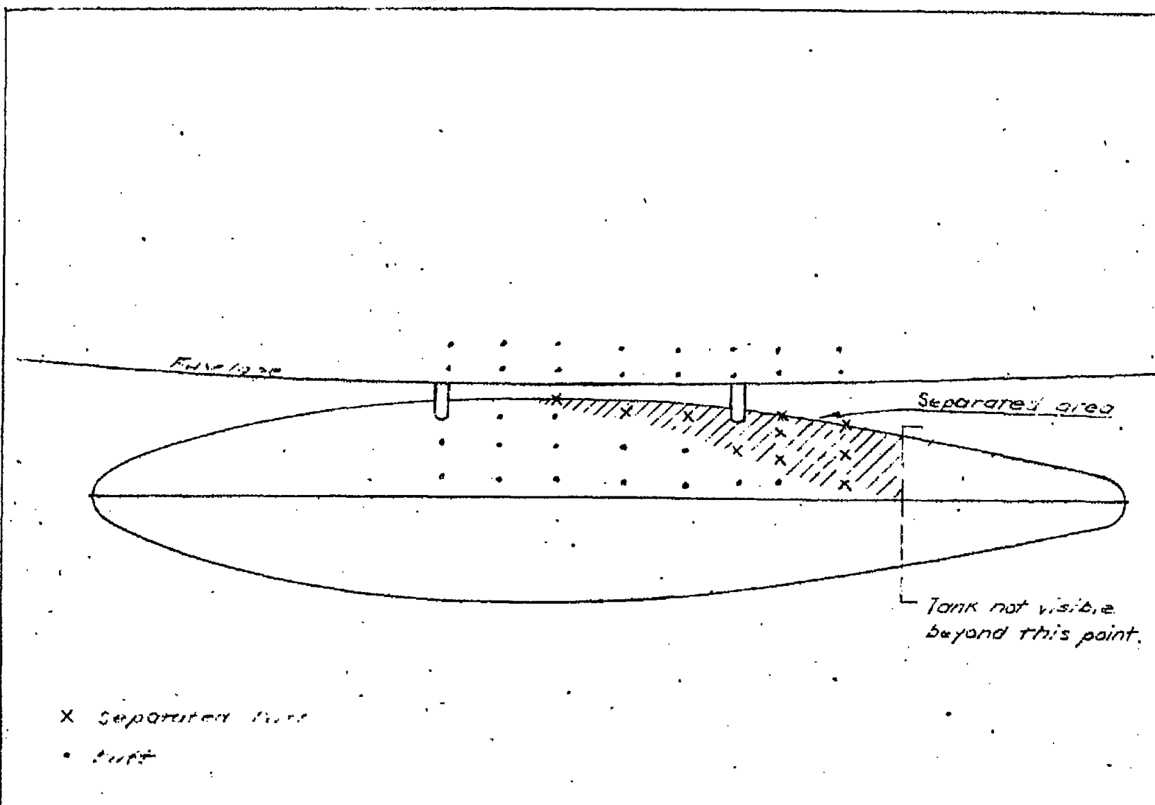
Fig. 10.- Flow separation at high speed around an auxiliary fuel tank mounted under the fuselage of a Grumman F7F-3 airplane. M \approx 0.725 .
