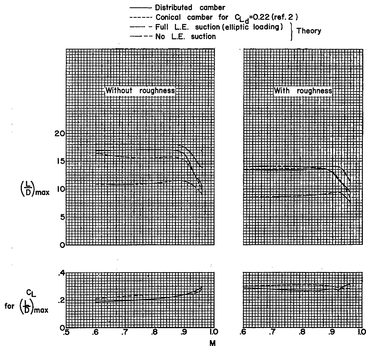
Figure 12.- The variation with Mach number of the maximum lift-drag ratios and the lift coefficients for maximum lift-drag ratios; R = 1.5 \times 10^6 .
