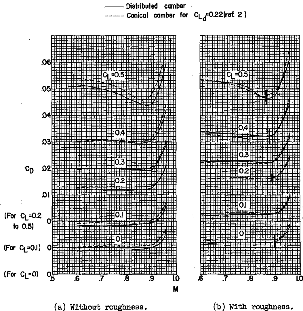
Figure 8.- The variation with Mach number of the drag coefficient at constant lift coefficients; R = 1.5 \times 10^6
