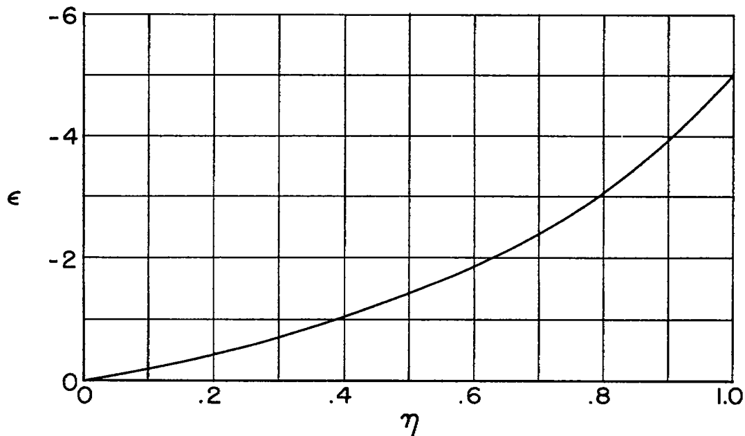
Figure 3.- Wing twist distribution.
