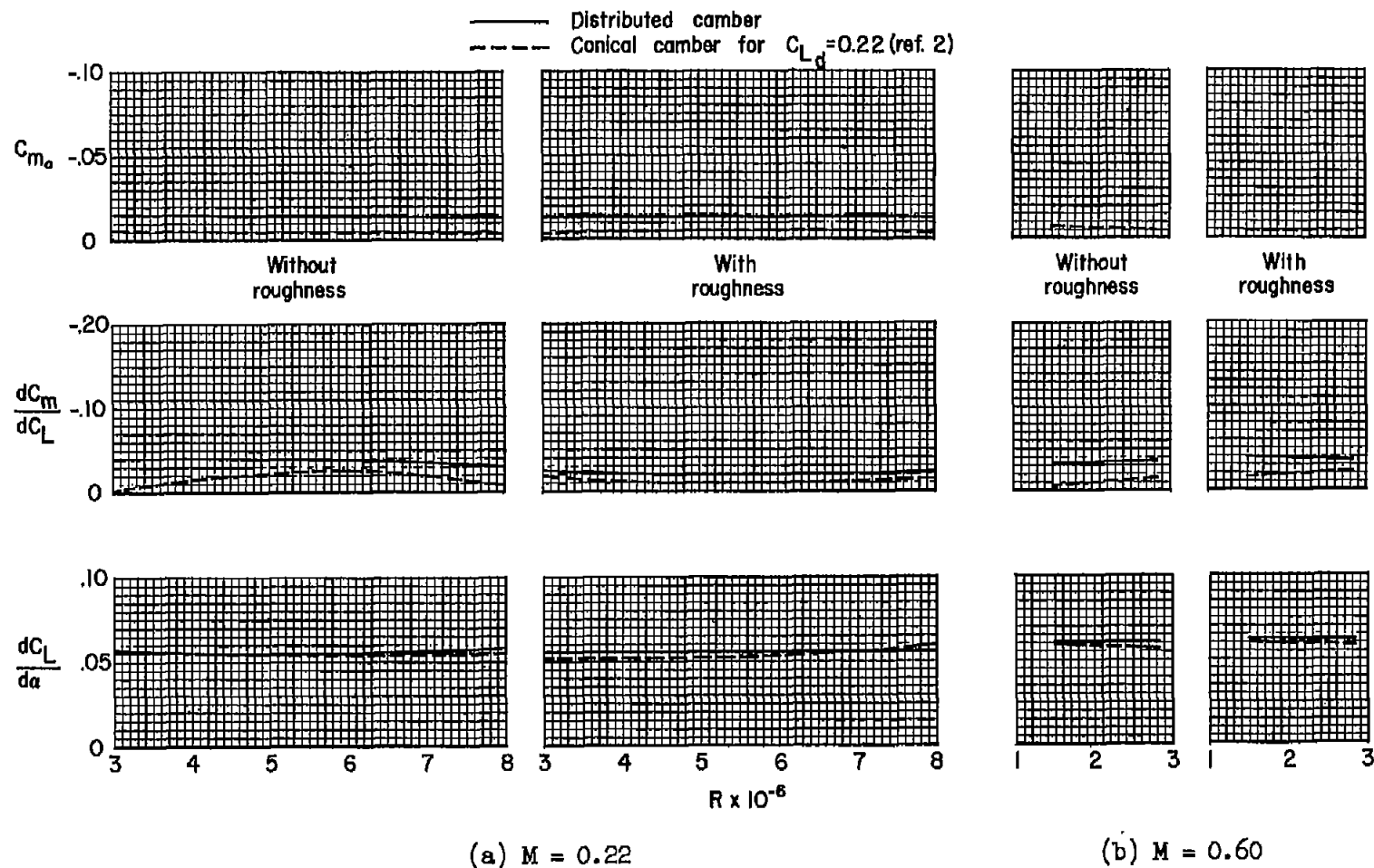
Figure 13.- The variation with Reynolds number of the pitching moment and the lift and pitching-moment curve slopes; C_{L_i} = 0 .
