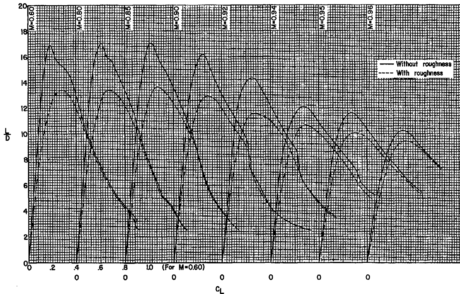
Figure 10.- The effect of Mach number on the lift-drag ratios; R = 1.5 \times 10^6 .
