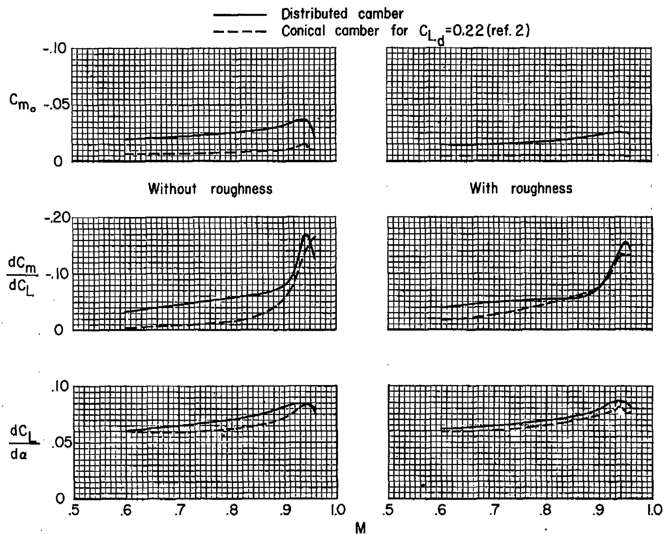
Figure 14.- The variation with Mach number of the pitching moment and the lift and pitching-moment curve slopes; C_L = 0 , R = 1.5 \times 10^8 .
