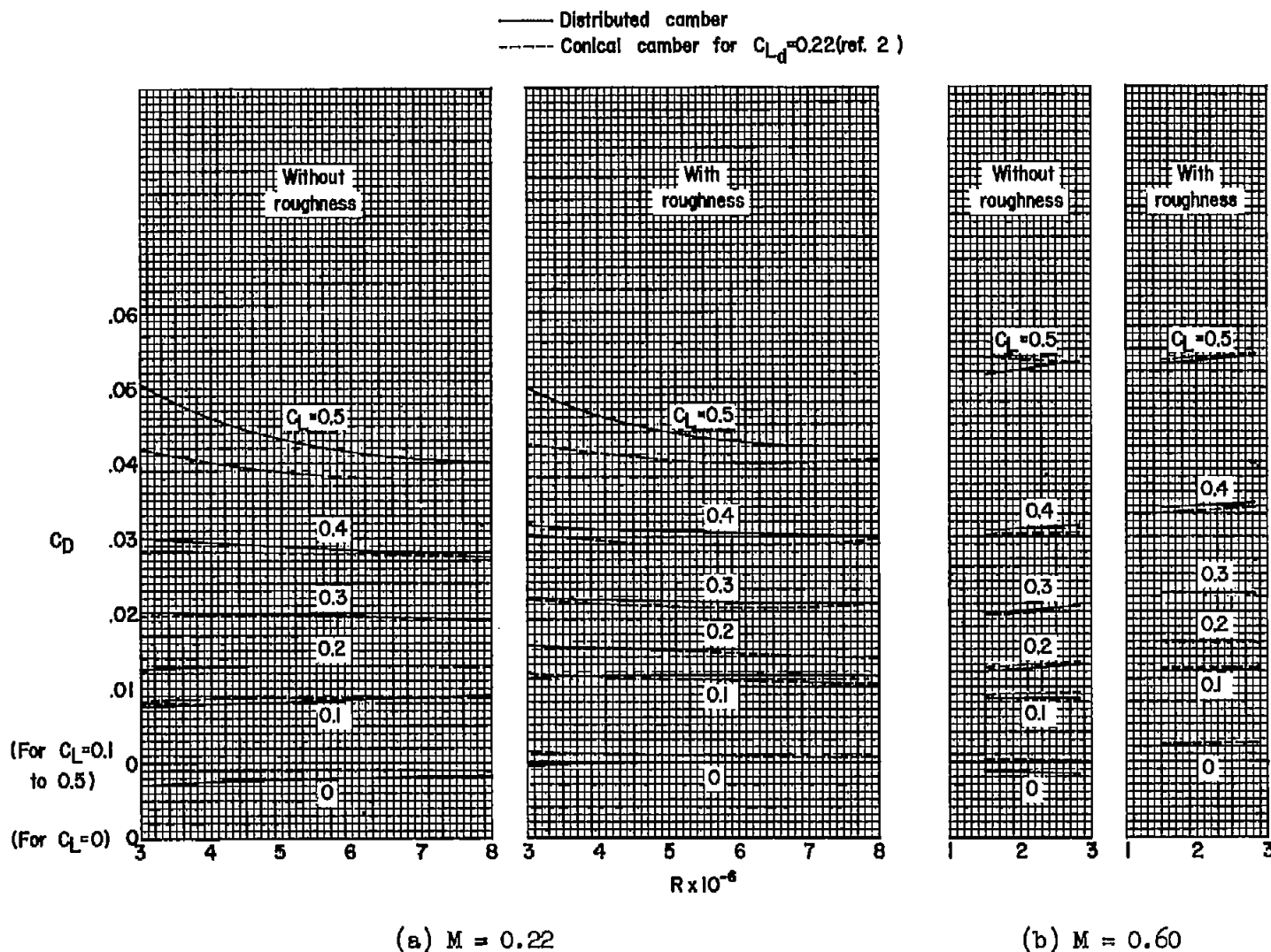
Figure 7.- The variation with Reynolds number of the drag coefficients at constant lift coefficients.
