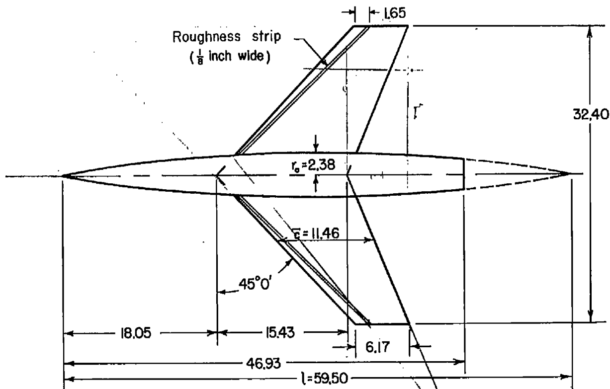
Figure 1.- Model arrangement.
