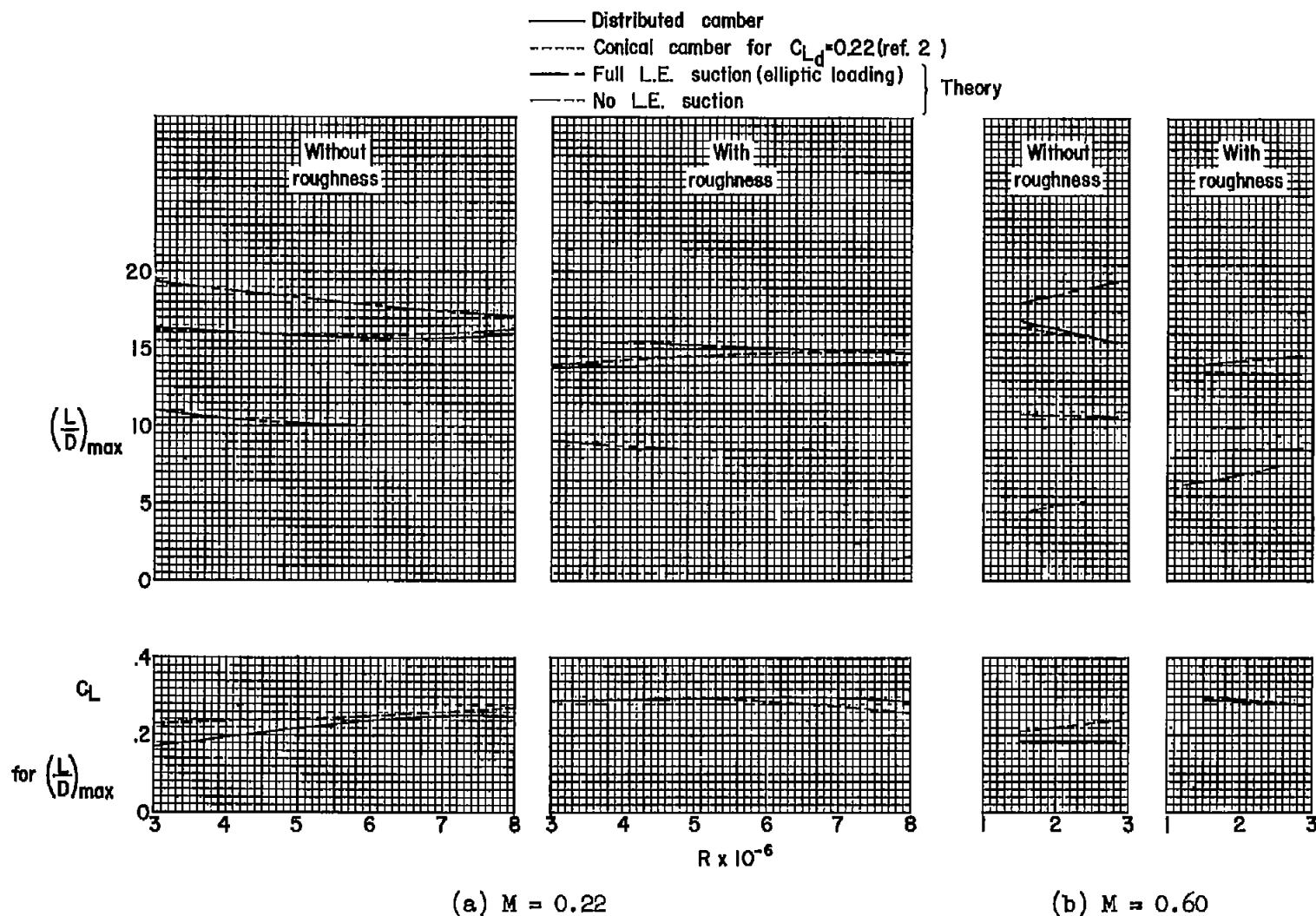
Figure 11.- The variation with Reynolds number of the maximum lift-drag ratios and the lift coefficients for maximum lift-drag ratios.
