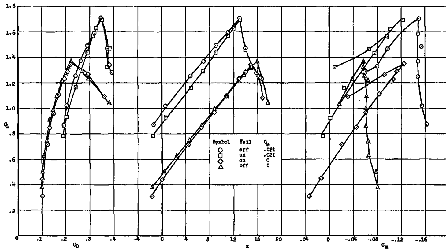
Figure 11.- Aerodynamic characteristics of the airplane with and without the horizontal tail; \delta_F = 60^\circ , R = 7.5 \times 10^6 , h_B = 0.040 inch, tail incidence = 0^\circ .
