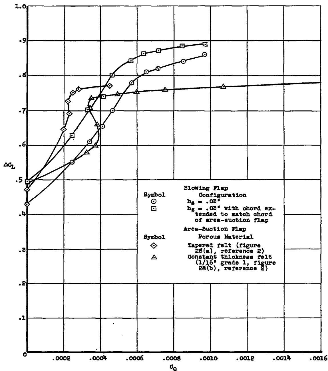
(b) Variation of lift-coefficient increment with flow coefficient; \delta_f = 55^\circ .
