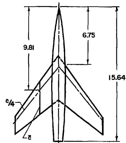
\lambda = 0.4
