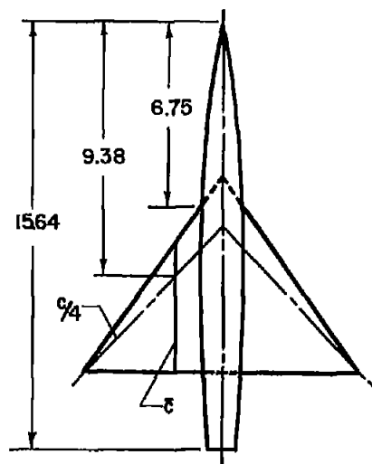
\lambda = 0
