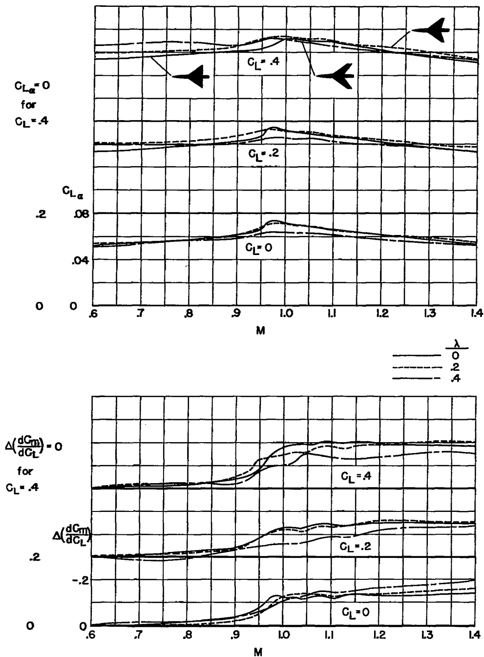
Figure 10.- Effect of taper ratio on the variation with Mach number of lift-curve slope and pitching-moment-curve slope; \Delta = 53.1^\circ .
