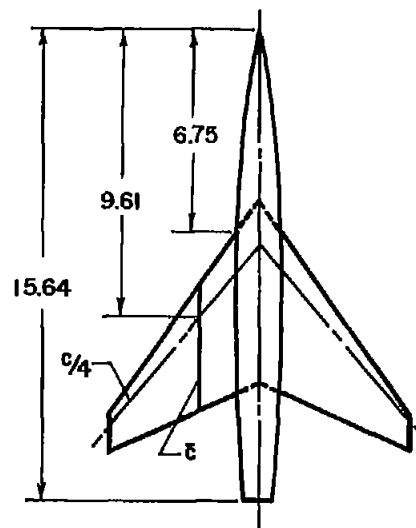
\lambda = 0.2
