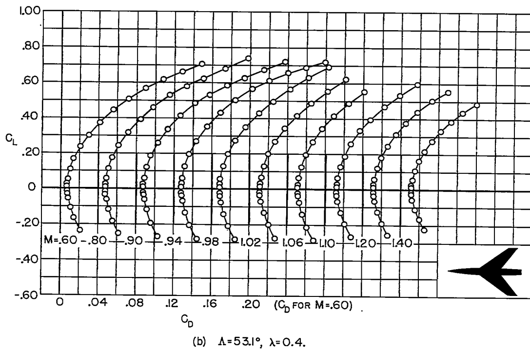
Figure 6.- Variation of drag coefficient with lift coefficient at constant Mach number.
