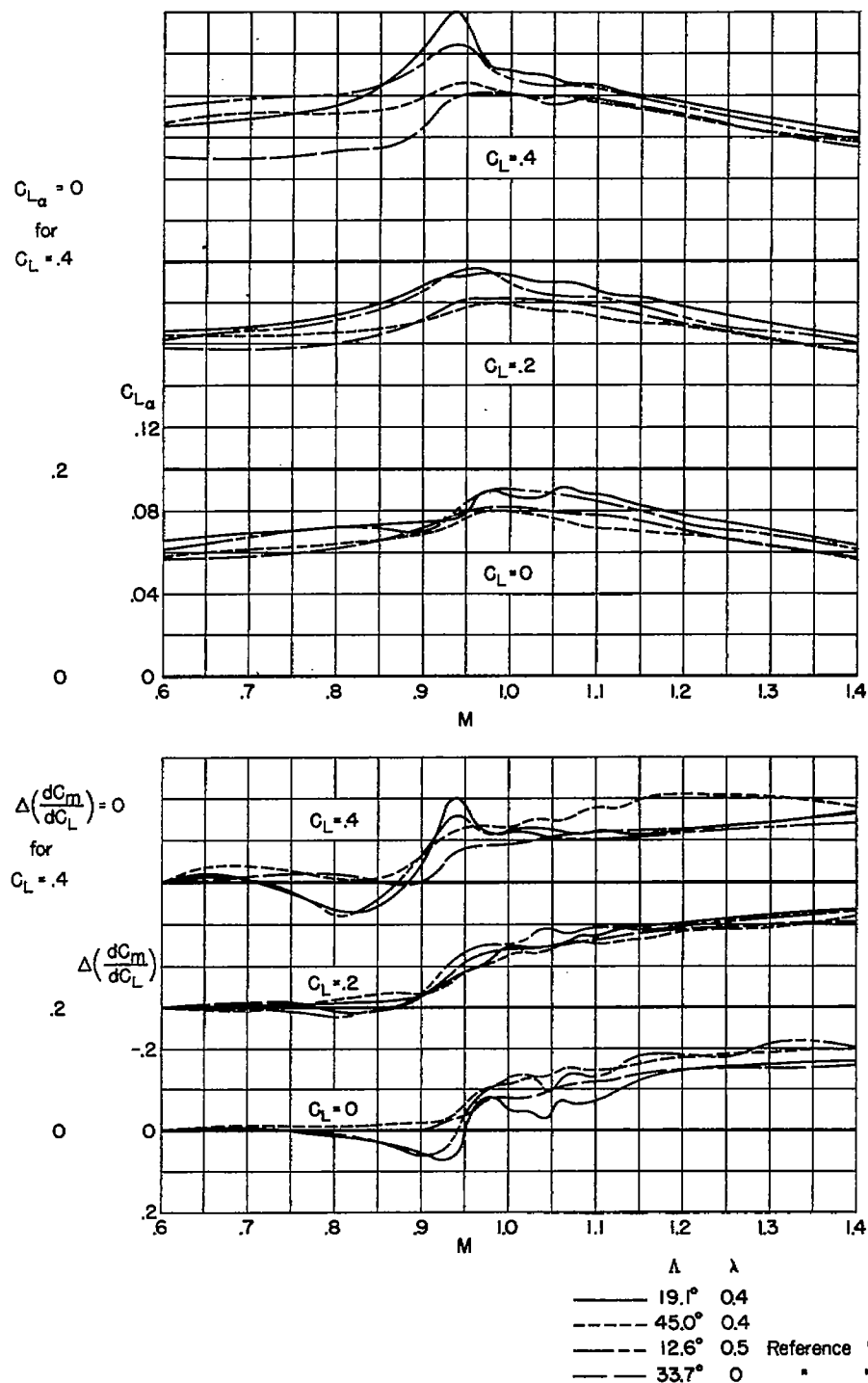
Figure 12.- Comparison of the effect of sweep as varied by two geometric methods on the variation with Mach number of lift-curve slope and pitching-moment-curve slope.
