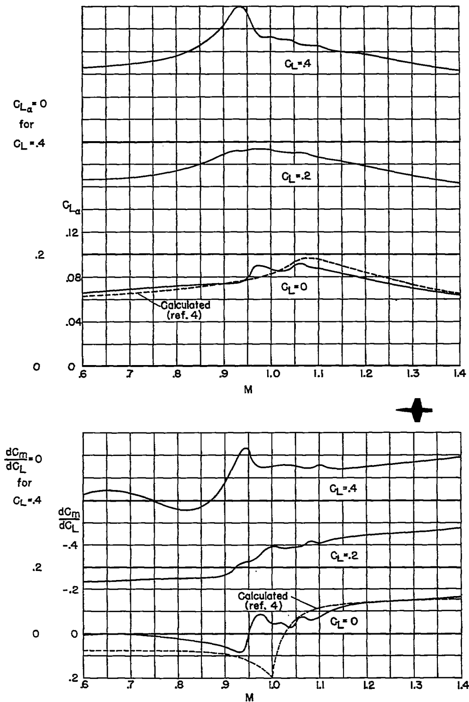
Figure 7.— Variation of lift-curve slope and pitching-moment-curve slope with Mach number.
