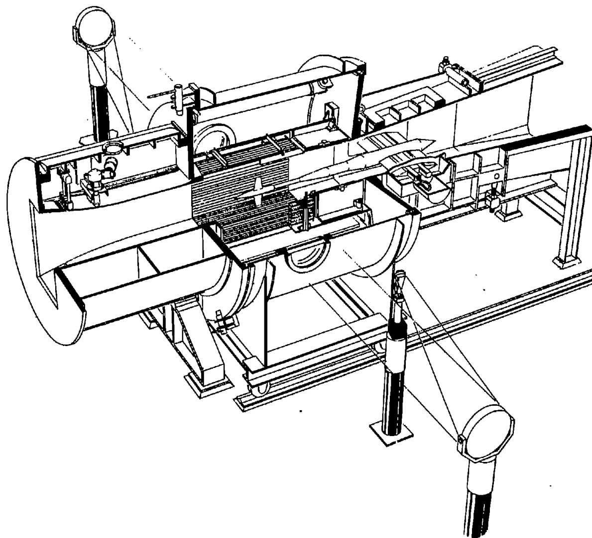
Figure 1.- The Ames 2-by 2-foot transonic wind tunnel.
