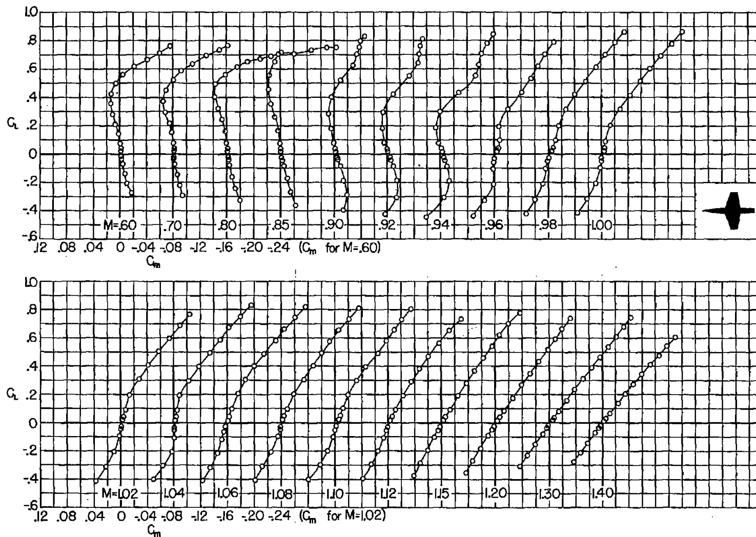
Figure 5.- Variation of pitching-moment coefficient with lift coefficient at constant Mach number.
