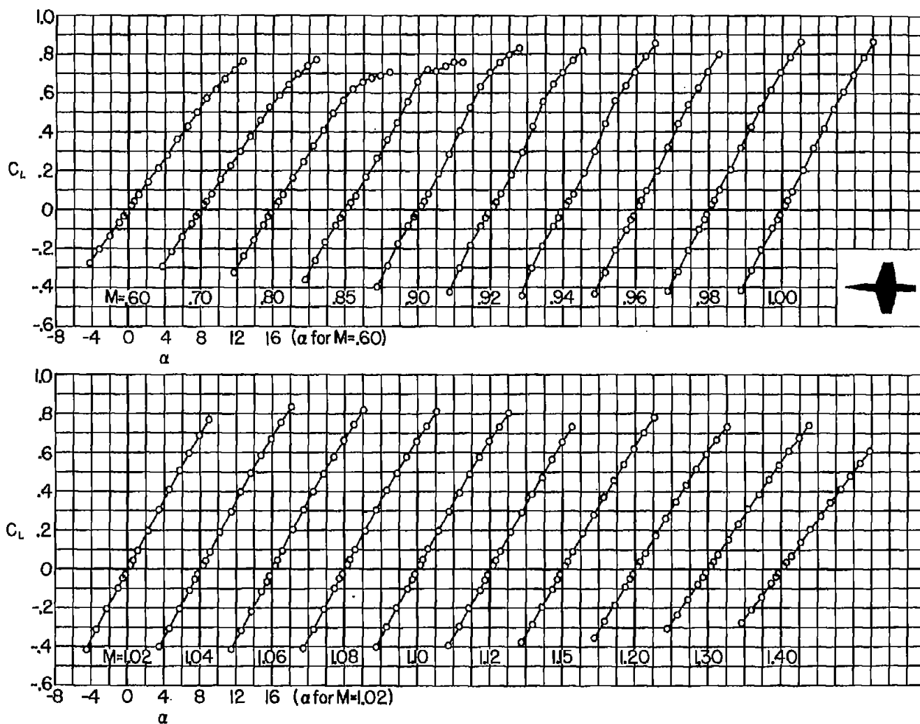
Figure 4.-Variation of lift coefficient with angle of attack at constant Mach number.
