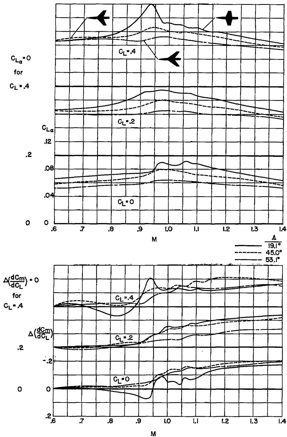
Figure 8.- Effect of sweep on the variation with Mach number of lift-curve slope and pitching-moment-curve slope; \lambda = 0.4 .
