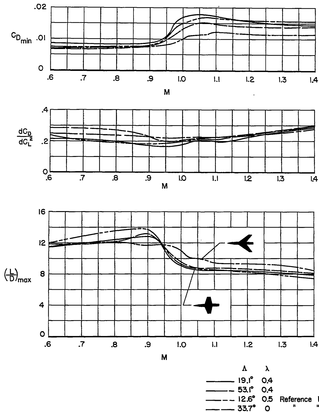
Figure 9.- Effect of sweep on the variation with Mach number of minimum drag coefficient, drag-rise factor, and maximum lift-drag ratio.
