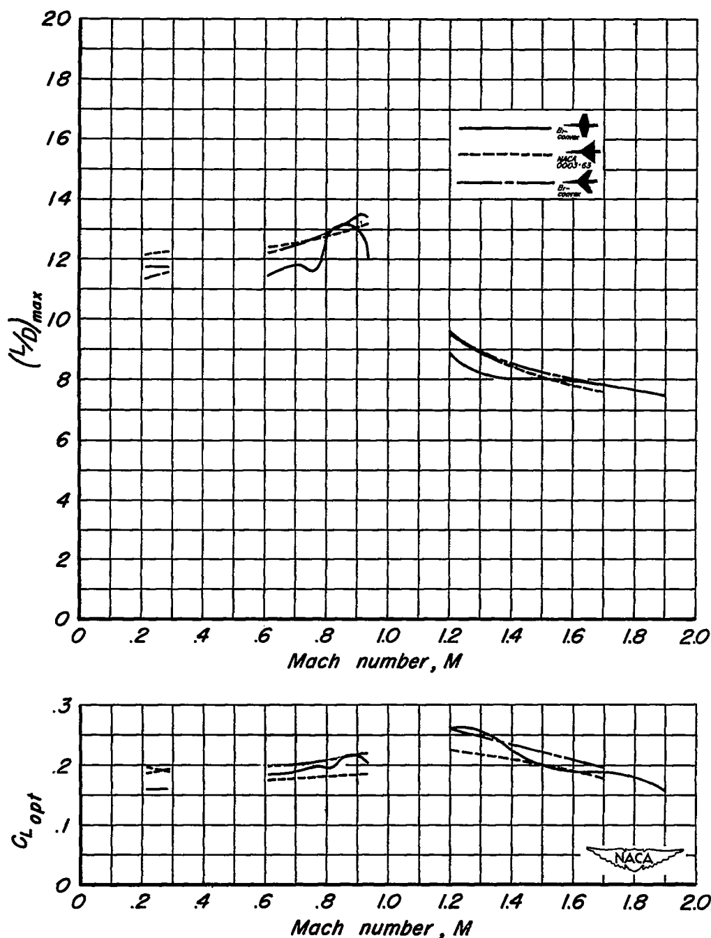
Figure 20.—The maximum lift-drag ratio and optimum lift coefficient for plane wings 3 percent thick and having different types of plan form.
